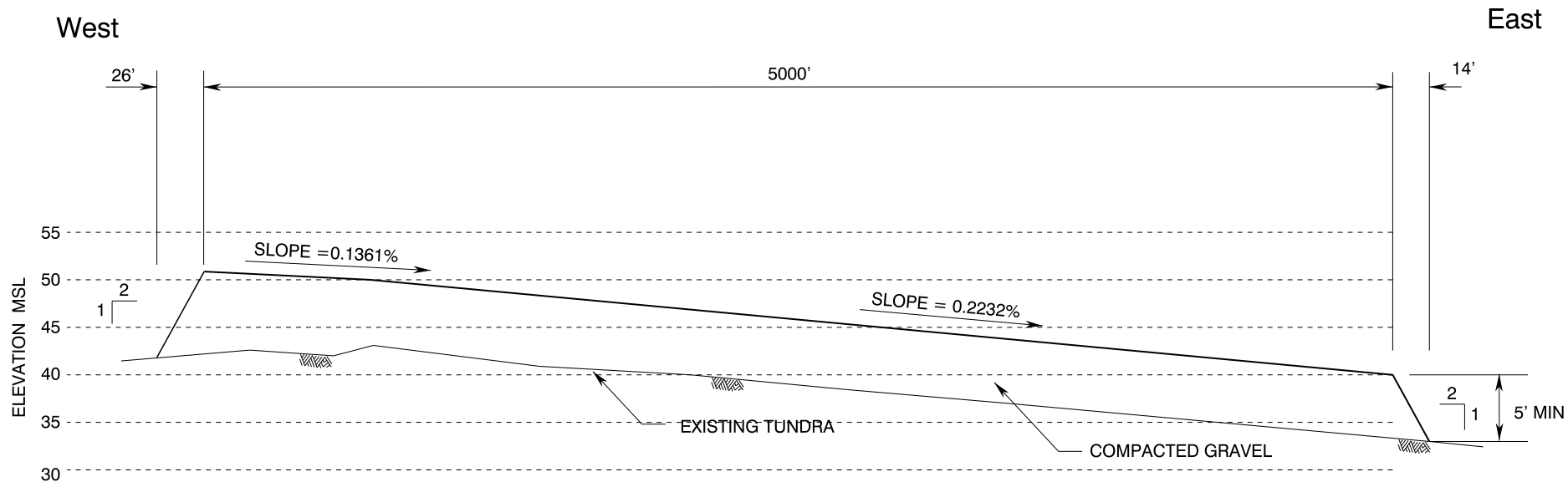
CROSS SECTION C - C'
