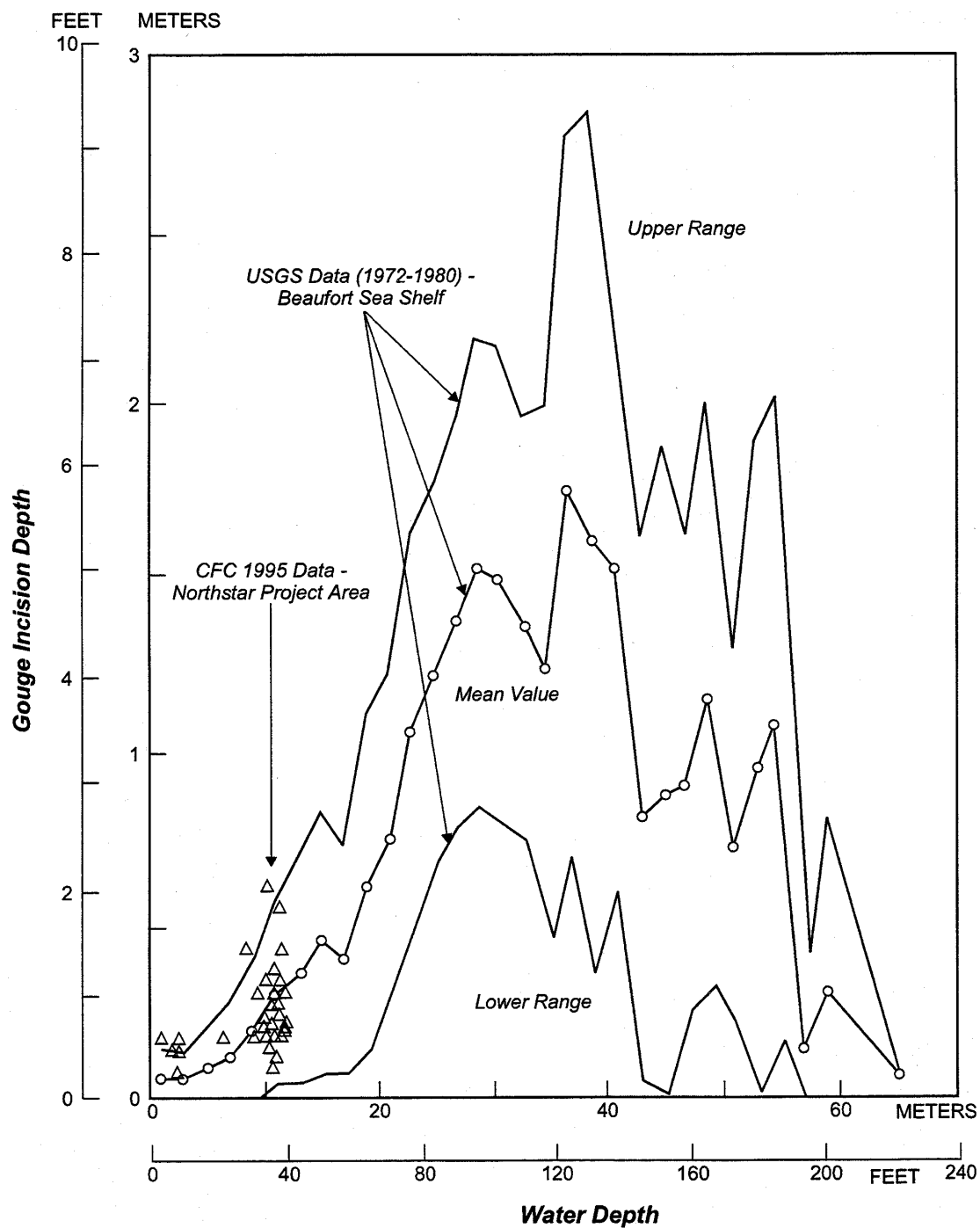
Figure 7.1-10. Gouge Depth Survey Measurements as a Function of Water Depth (COE, 1999).
