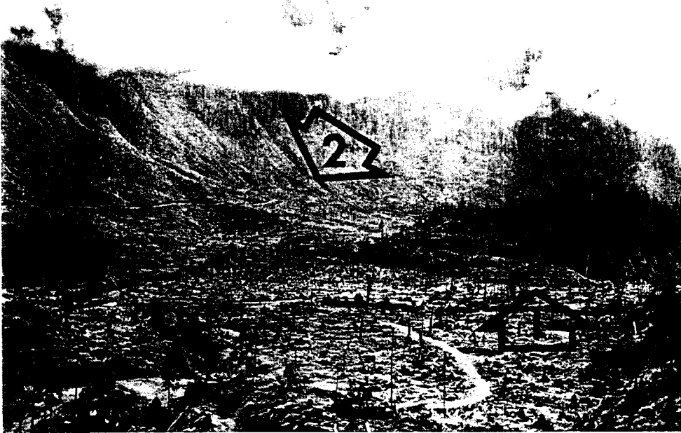
Figure 4. Glaciated Neets Creek valley, Alaska, where weak metamorphic formations have released large rock masses into the valley bottom (arrow 1). Mass wasting of soil and rock also produced the fan below the ravine (arrow 2).
