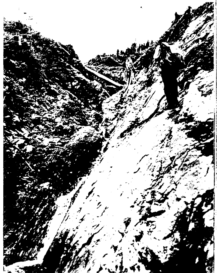
Figure 5. The effect of bedding is shown in this ravine through metamorphics. Parallel-bedded slope is bare; opposite slope retains soil mantle. Neets Bay, Alaska.
