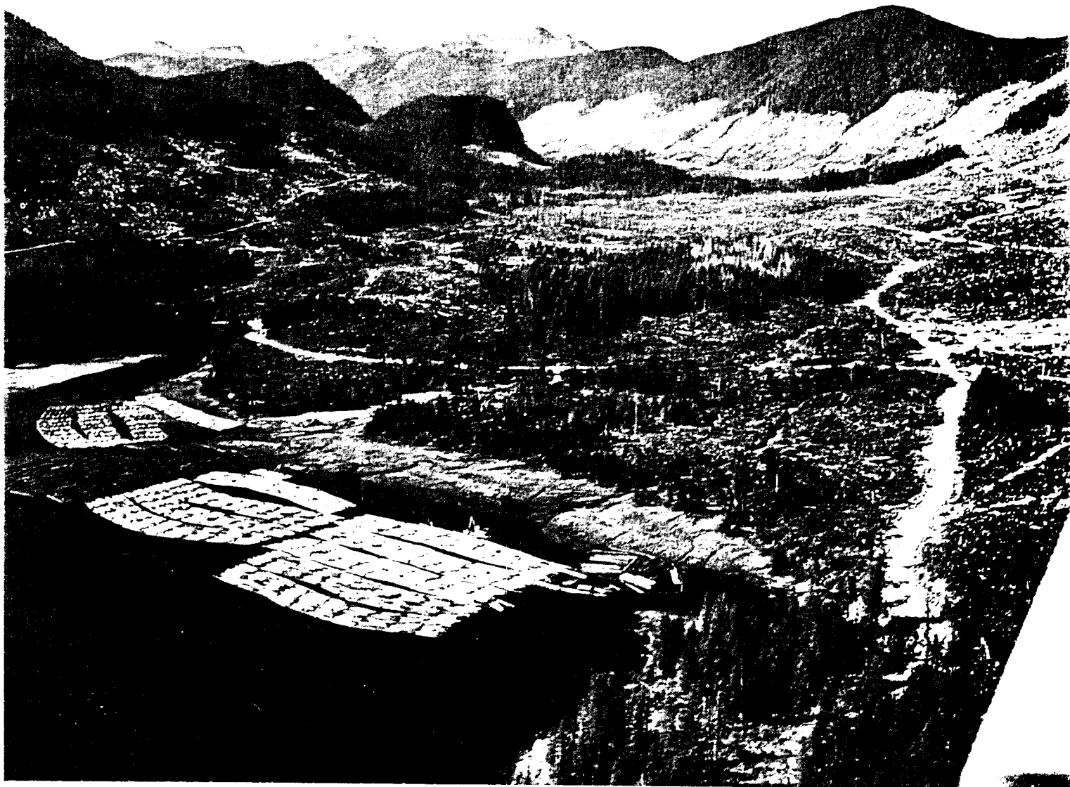
Logged areas in Mayhew Creek valley. The topography is typical of many valleys seen in Southeast Alaska.
