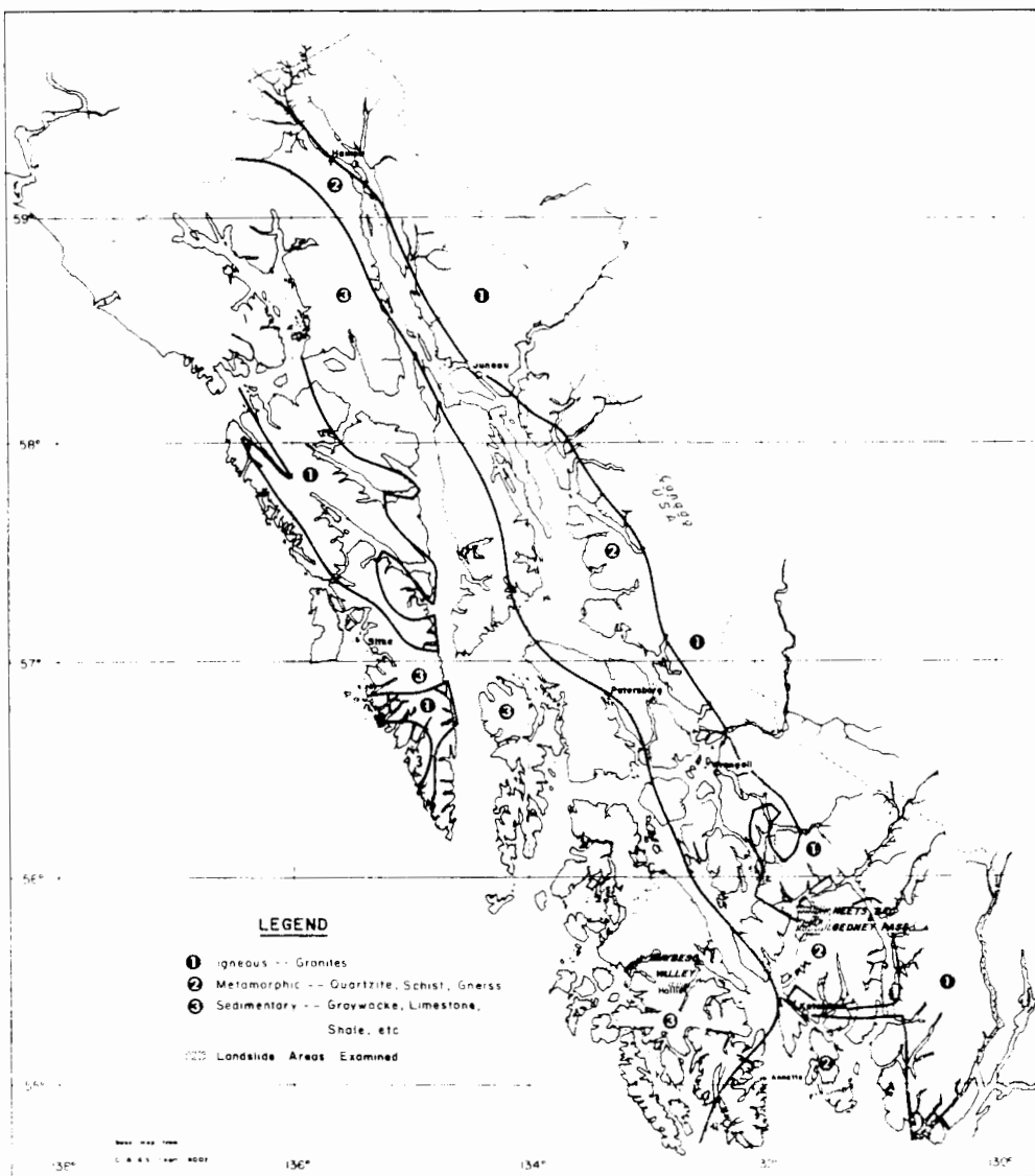
Figure 1.—Generalized bedrock geology of southeast Alaska. Adapted from Geologic Map of Alaska (Dutro and Payne, 1954).
