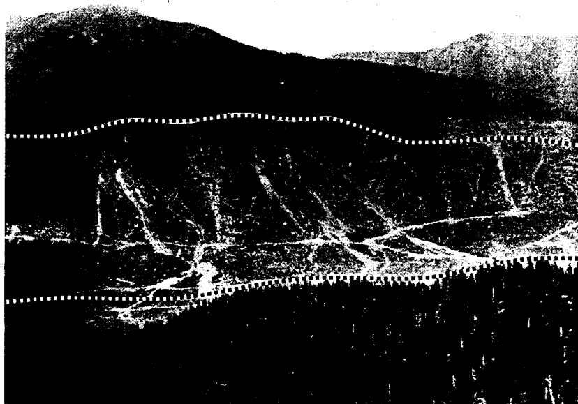
Figure 6.—October 1961 debris avalanches and flows in the mile-square clearcutting in the Maybeso Creek drainage, Hollis, Alaska. The Karta soil series is between the dashed lines. Photo taken August 8, 1962.
