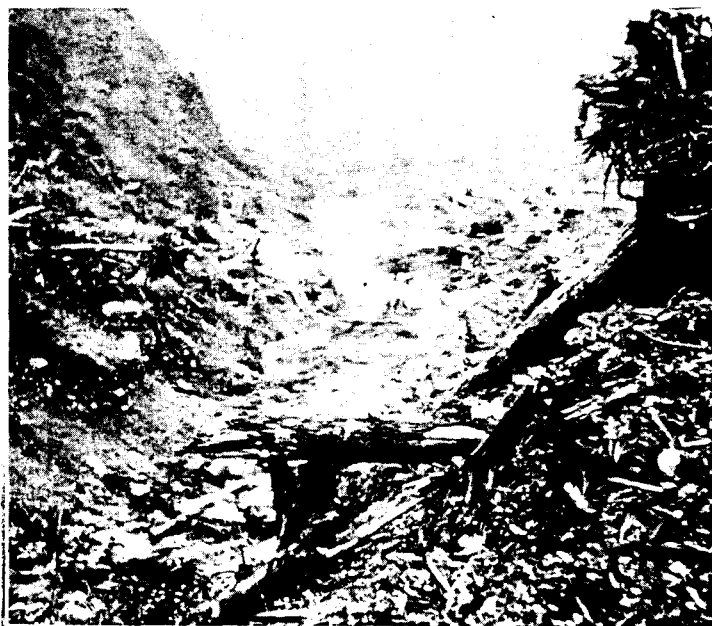
Figure 10.—Gorge from which one of the authors climbed a few minutes before it began to flow.
