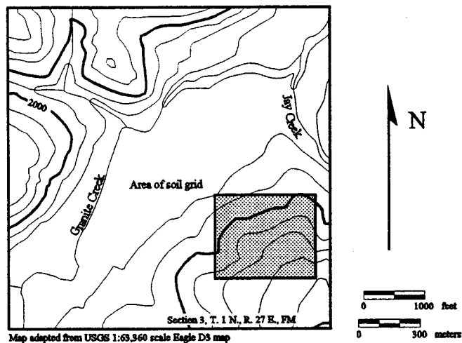
Figure 10 Jay Creek area - Sample site grid.
