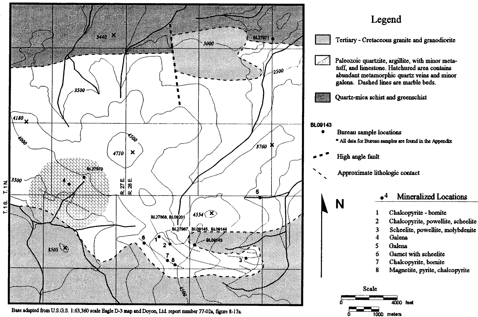
Figure 6 Deer Creek occurrence - Geology and sample sites.
