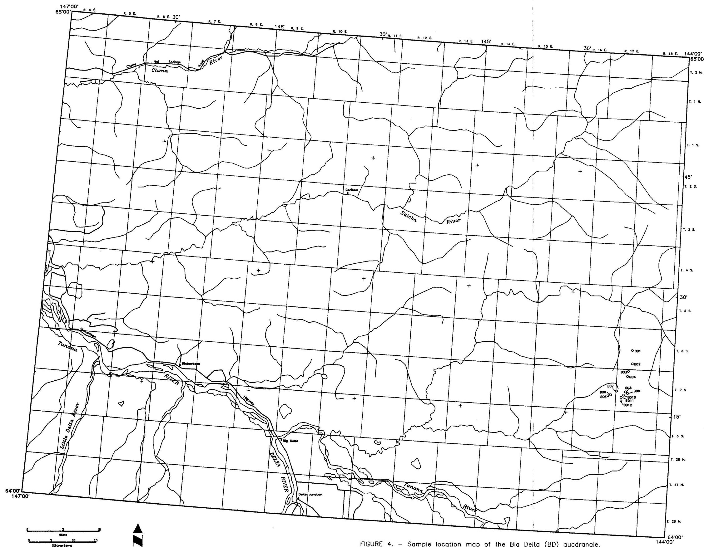
FIGURE 4. - Sample location map of the Big Delta (BD) quadrangle.
