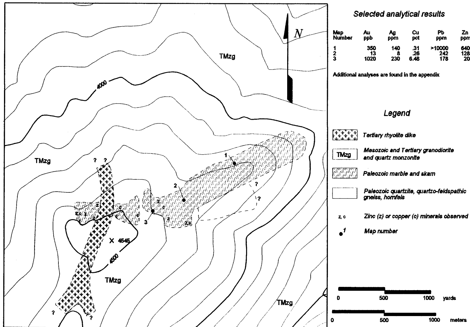
Figure 14 Mitchell Copper - Geology and sample sites.
