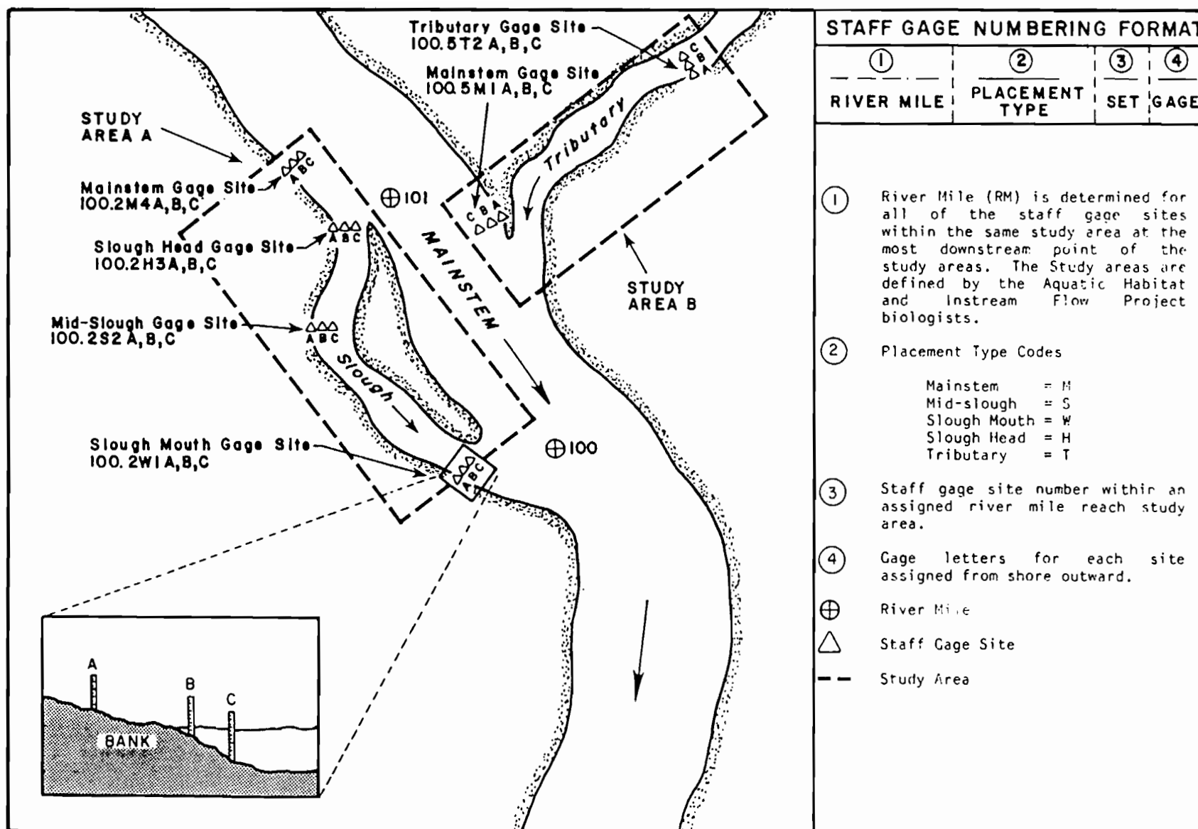
Figure 11. FY 83 ADF&G AH staff gage placement and identification system, 1982-83.
