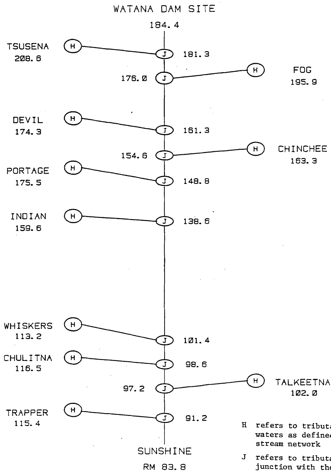
Figure 9. Stream network from Watana to Sunshine.
