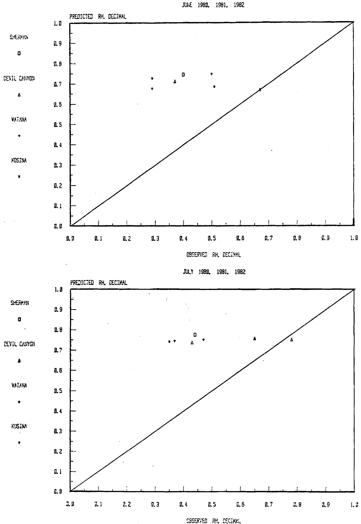
Figure 19. Susitna observed humidities vs. humidities predicted from Talkeetna data.
