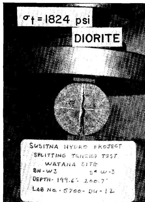
TYPICAL TENSILE TEST FAILURE
