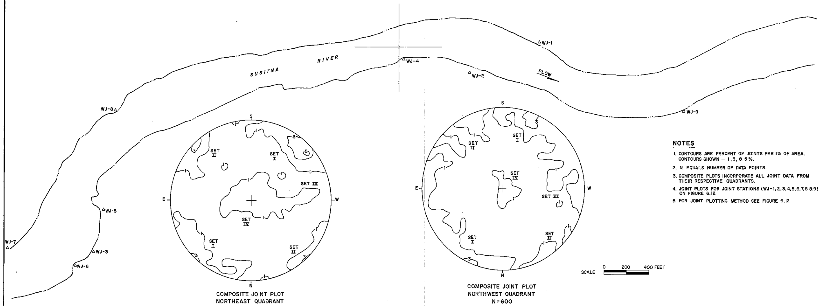
WATANA COMPOSITE JOINT PLOTS
