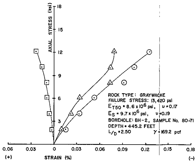
DEVIL CANYON STATIC ELASTIC PROPERTIES FOR ARGILLITE AND GRAYWACKE
