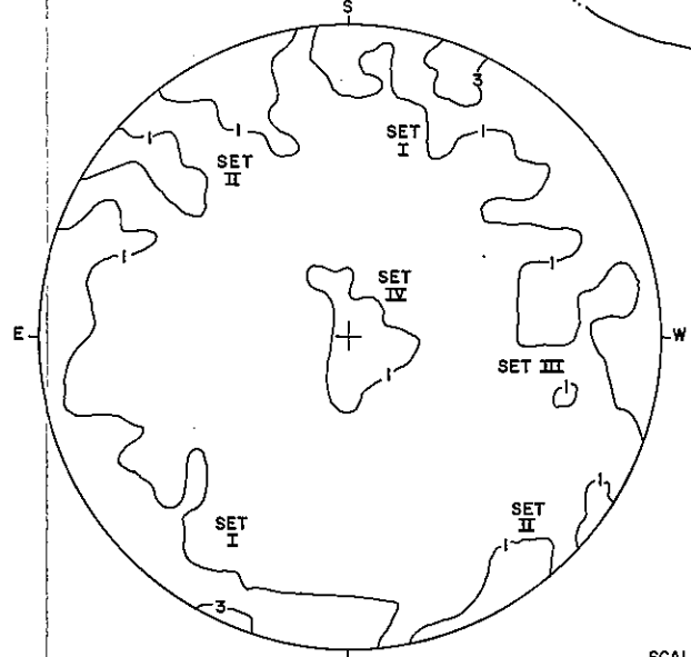
COMPOSITE JOINT PLOT NORTHWEST QUADRANT N=600
