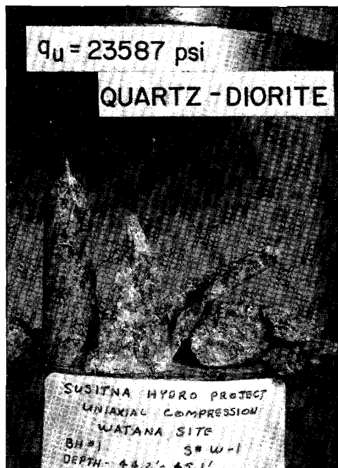
TYPICAL COMPRESSION TEST FAILURE
