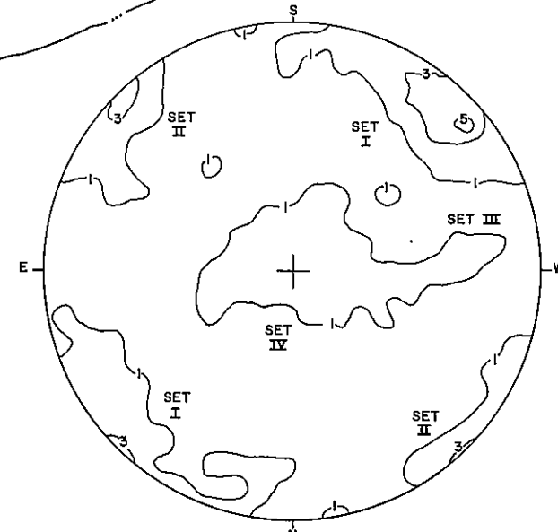
COMPOSITE JOINT PLOT NORTHEAST QUADRANT N=525
