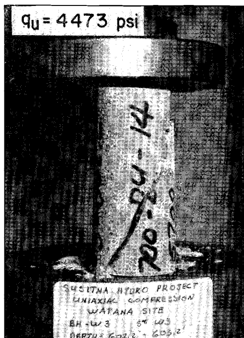
ALTERED DIORITE - COMPRESSION TEST
