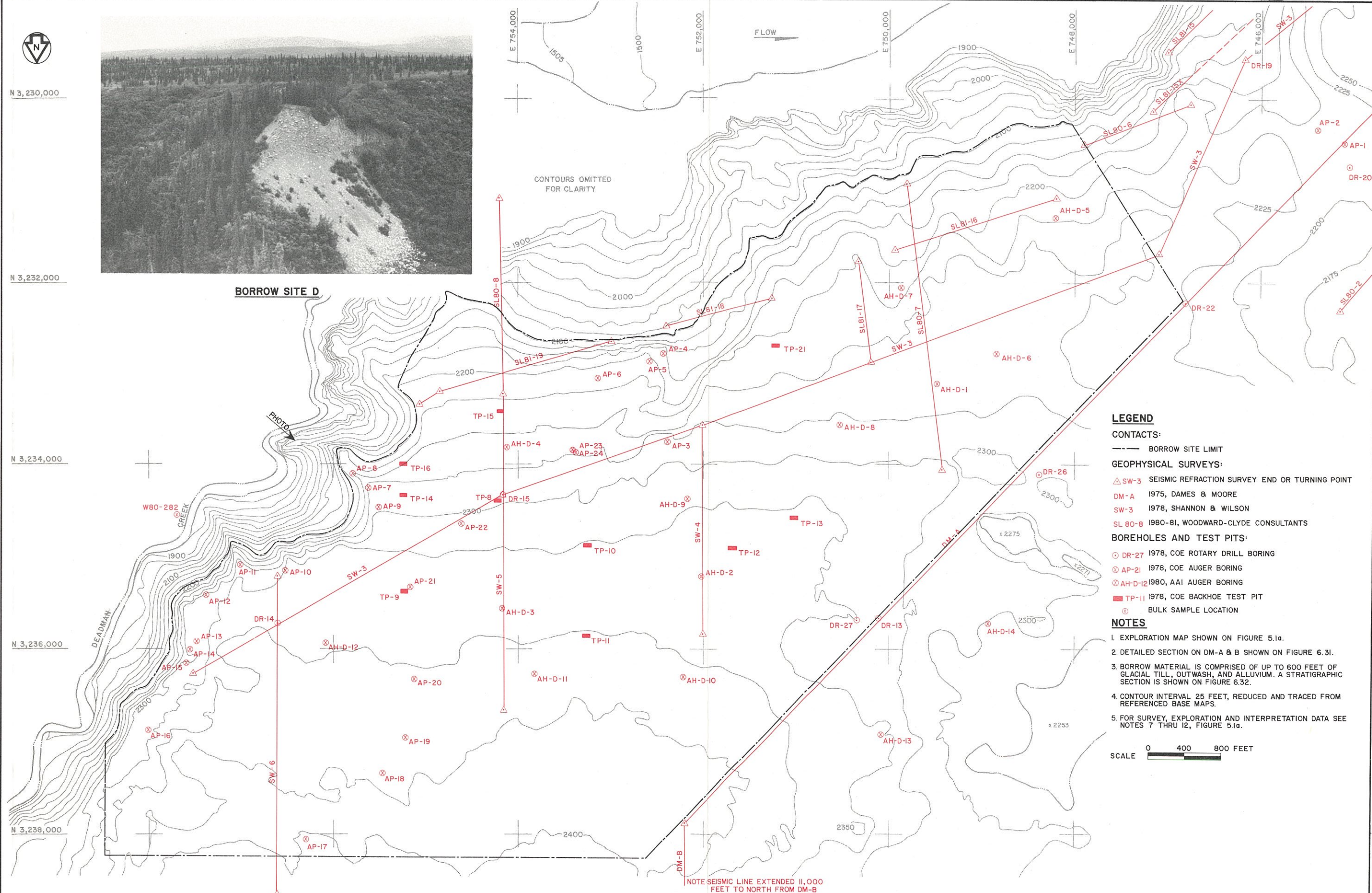
WATANA BORROW SITE D PLAN
