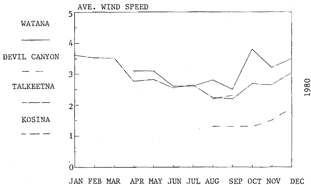
Figure 21. Average monthly wind speeds (M/S), 1980, 1981, 1982.
