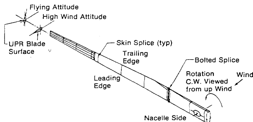
FIGURE 2.13. Rotor Blade Configuration (Source: Linscott, Dennett and Gordon 1981)
