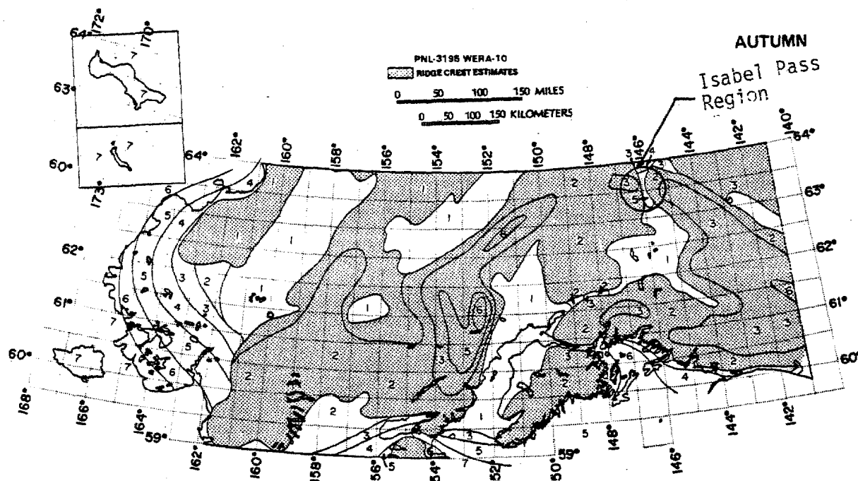
FIGURE 2.6. Seasonal Average Wind Power in Southcentral Alaska - Autumn (Source: AEIDC 1981)
