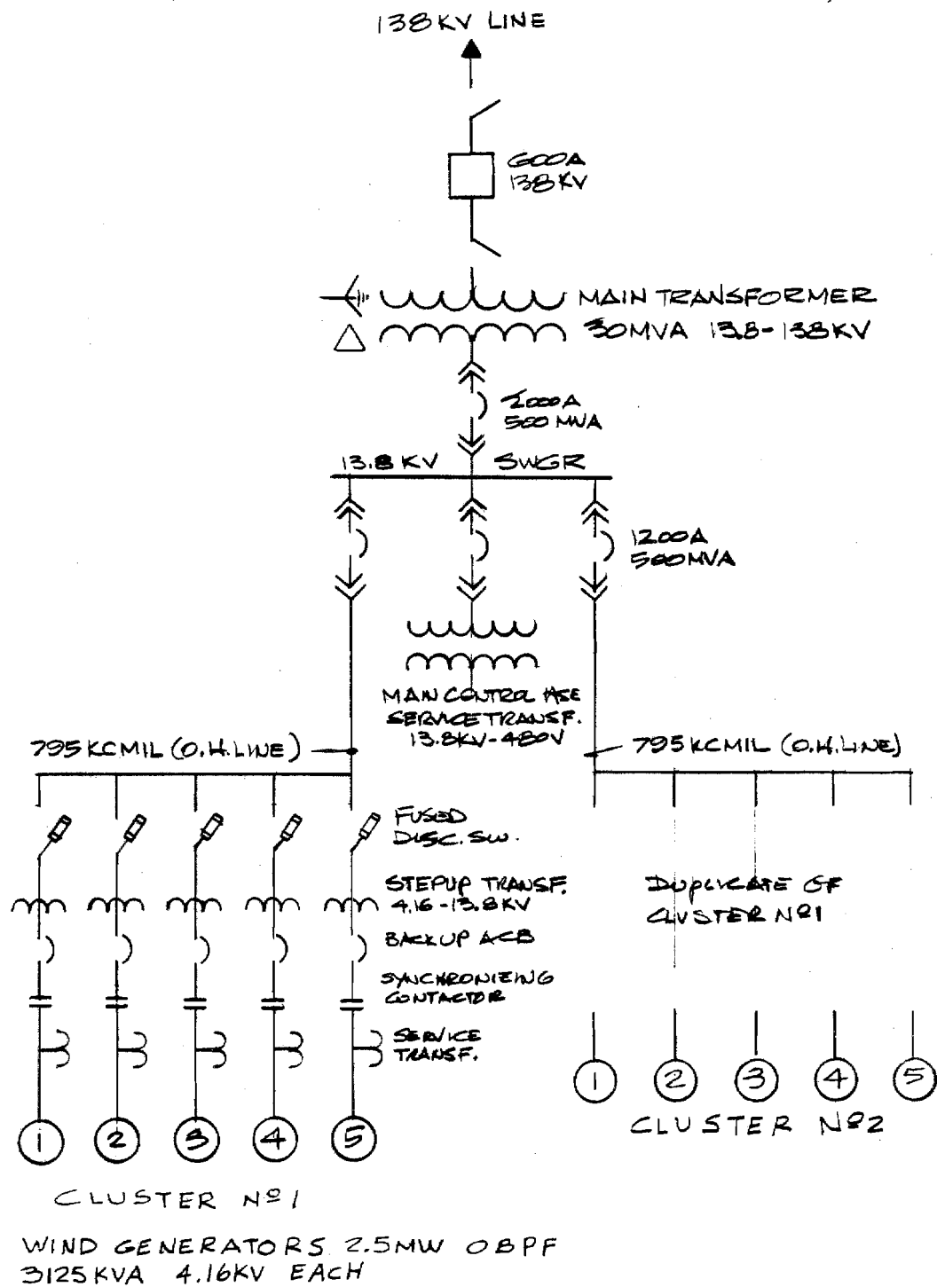
FIGURE 2.20. One-Line Diagram
