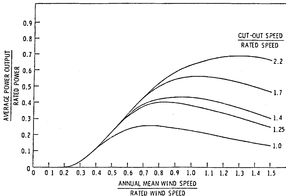
FIGURE 2.23. Estimate of Expected Average Power Output for Wind Turbines as a Function of Cutout, Rated and Mean Wind Speeds and Rated Power Output (Heister and Pennell 1980)
