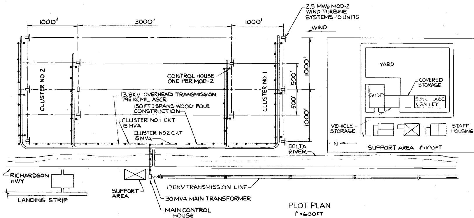
FIGURE 2.11. Large Wind Energy Conversion System Plot Plan
