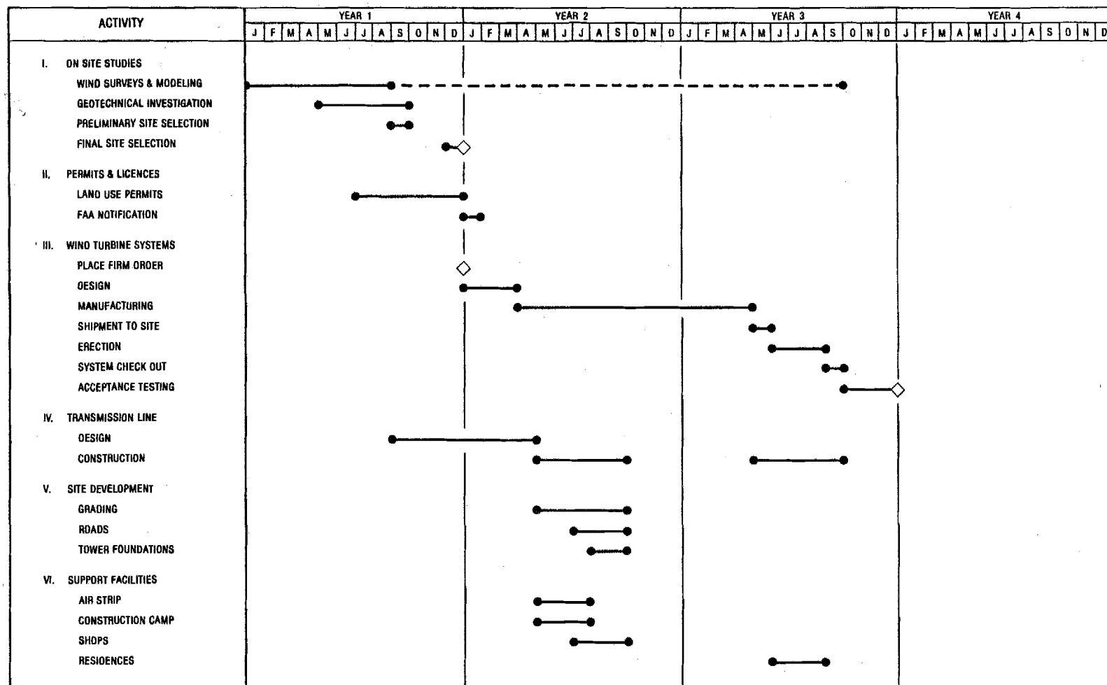
FIGURE 2.21. Project Schedule
