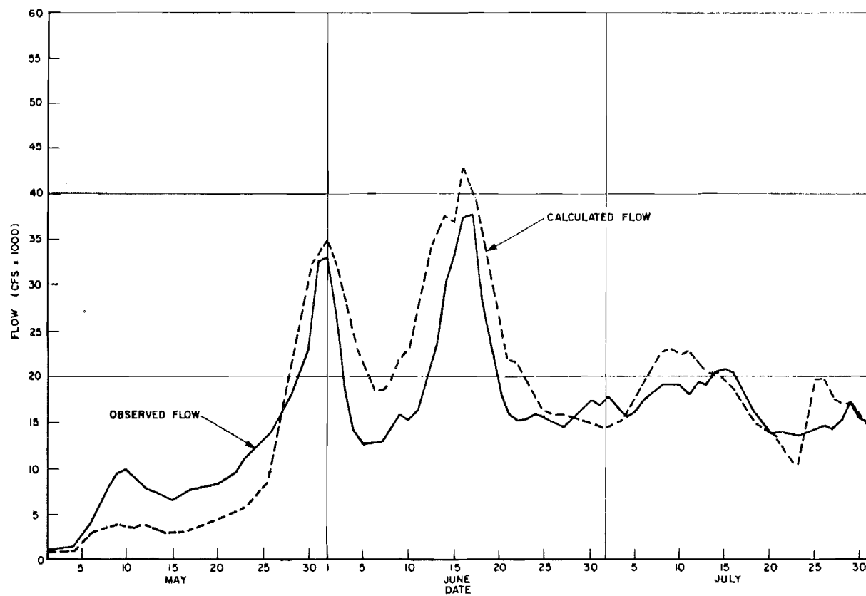
SSARR MODEL CALIBRATION SUSITNA RIVER NEAR CANTWELL 1972 FLOOD
