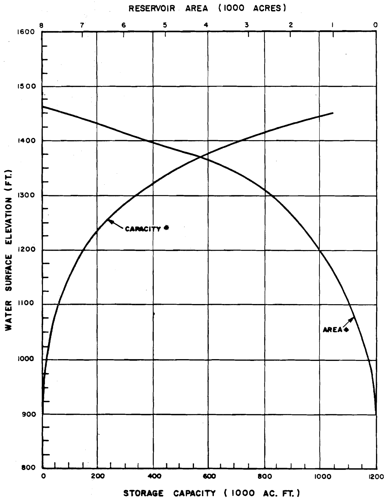
AREA AND CAPACITY CURVES DEVIL CANYON RESERVOIR
