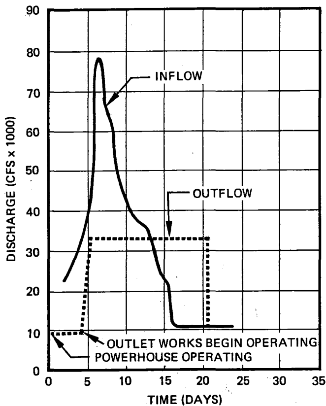
50 YEAR FLOOD (JULY-SEPT.)
