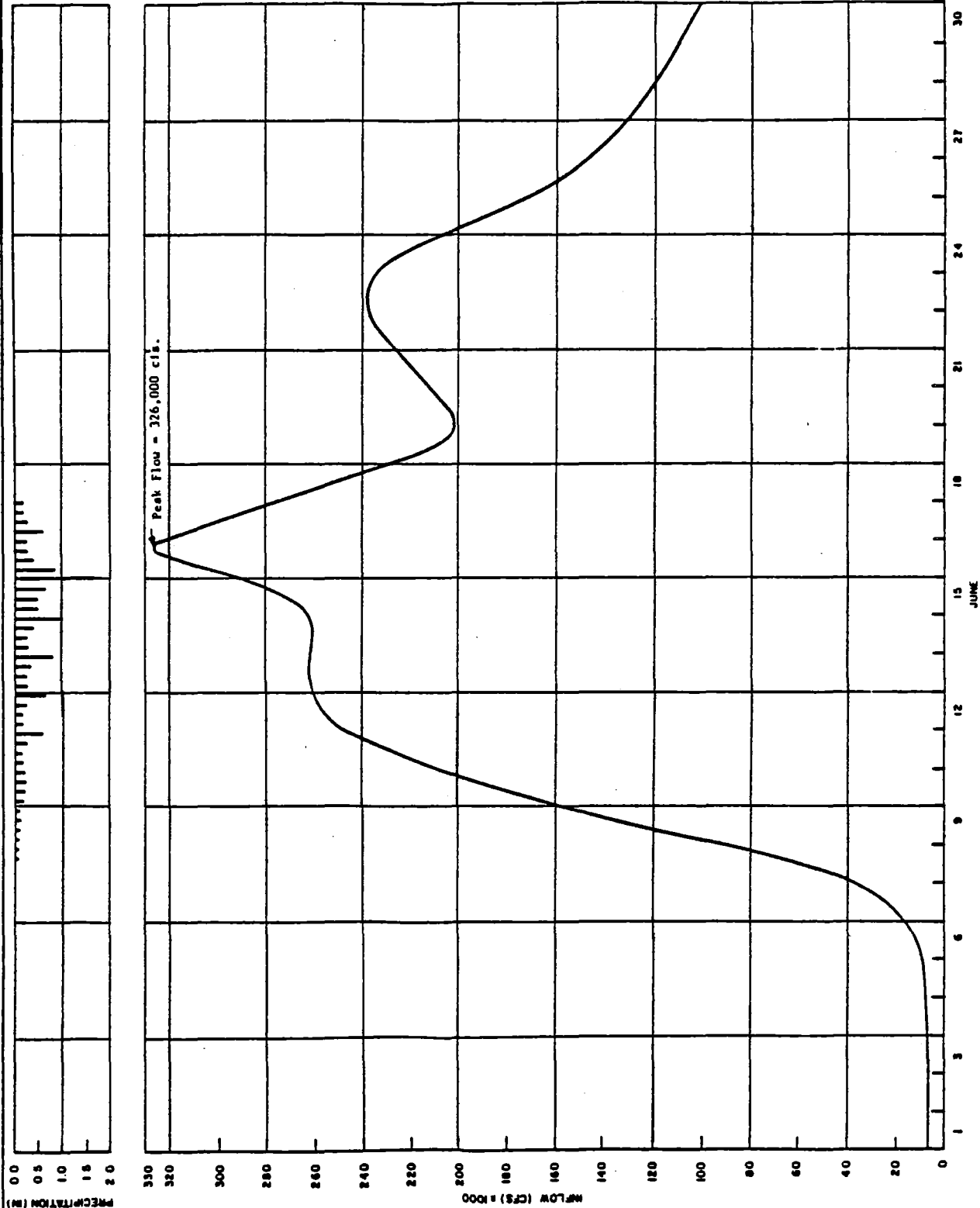
WATANA PMF INFLOW HYDROGRAPH
