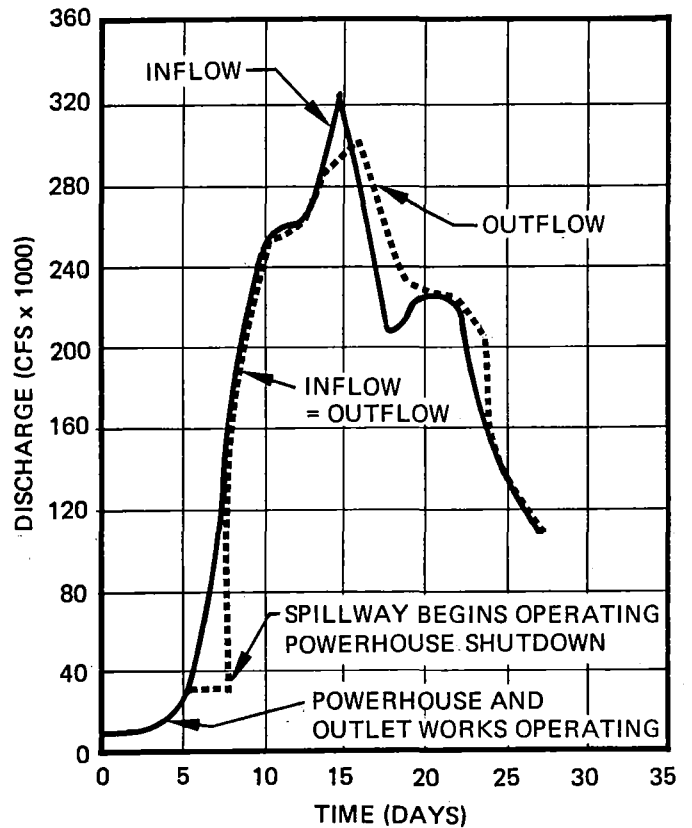
PROBABLE MAXIMUM FLOOD
