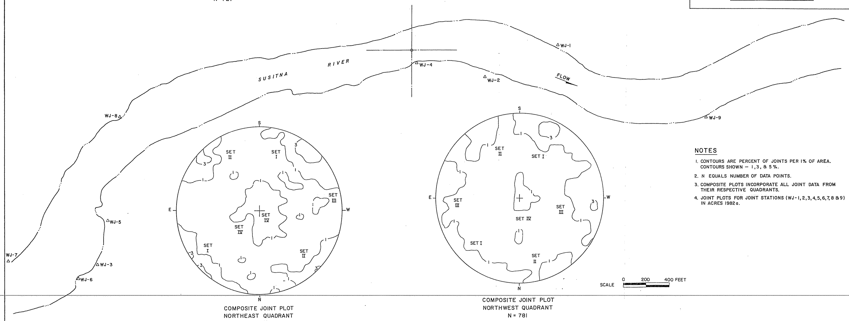
WATANA DAMSITE COMPOSITE JOINT PLOTS
