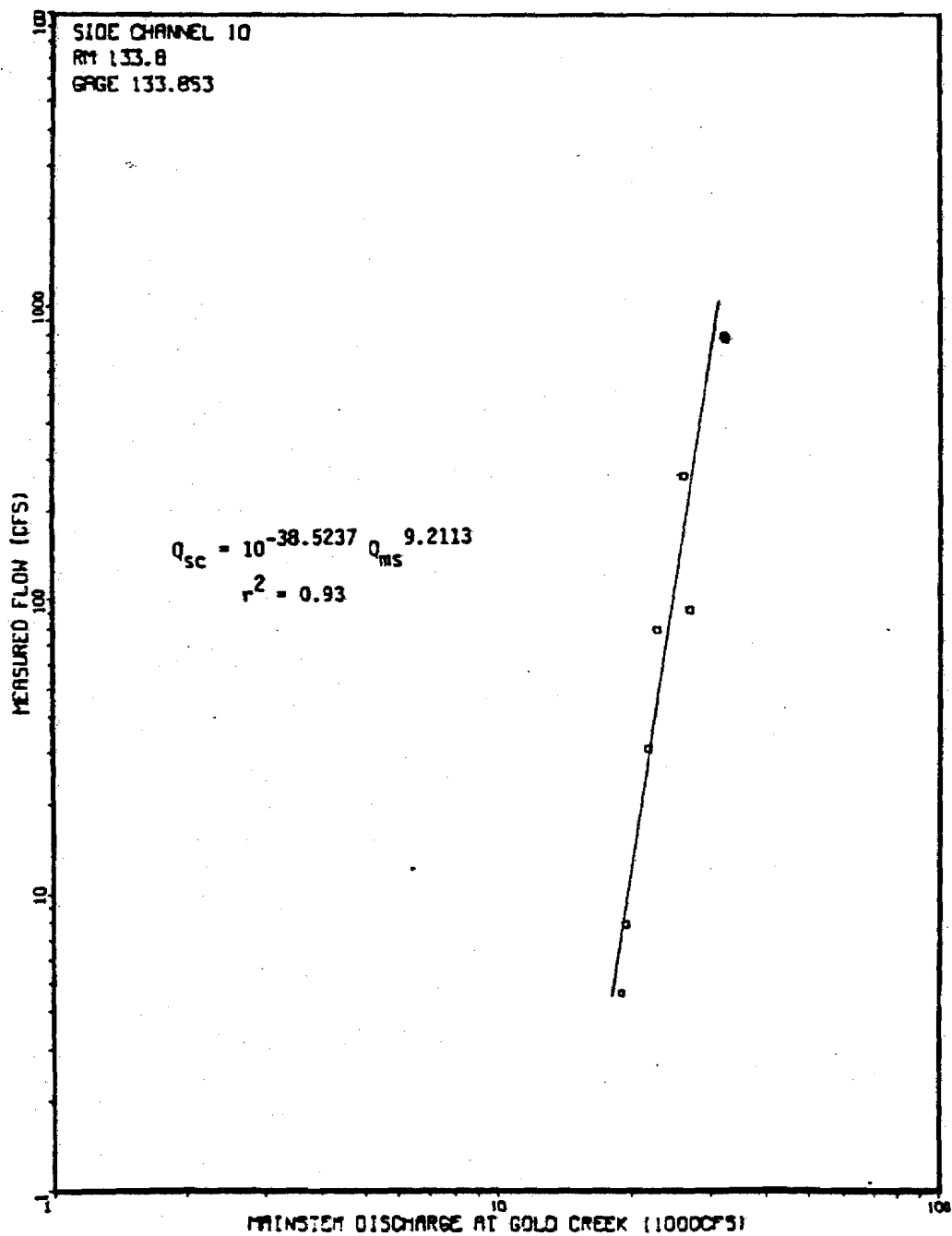
Appendix Figure A-4. Rating curve for predicting flow at Side Channel 10 at Mainstem discharges at Gold Creek between 19,000 cfs and 35,000 cfs.
