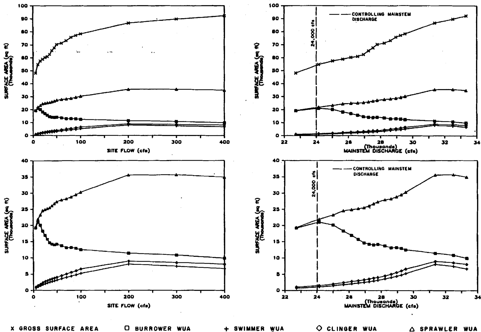
Figure 25. Projections of gross surface area and WUA of burrower, swimmer, clinger, and sprawler invertebrate habitat as a function of site flow and mainstem discharge for the Side Channel 21 modelling site.
