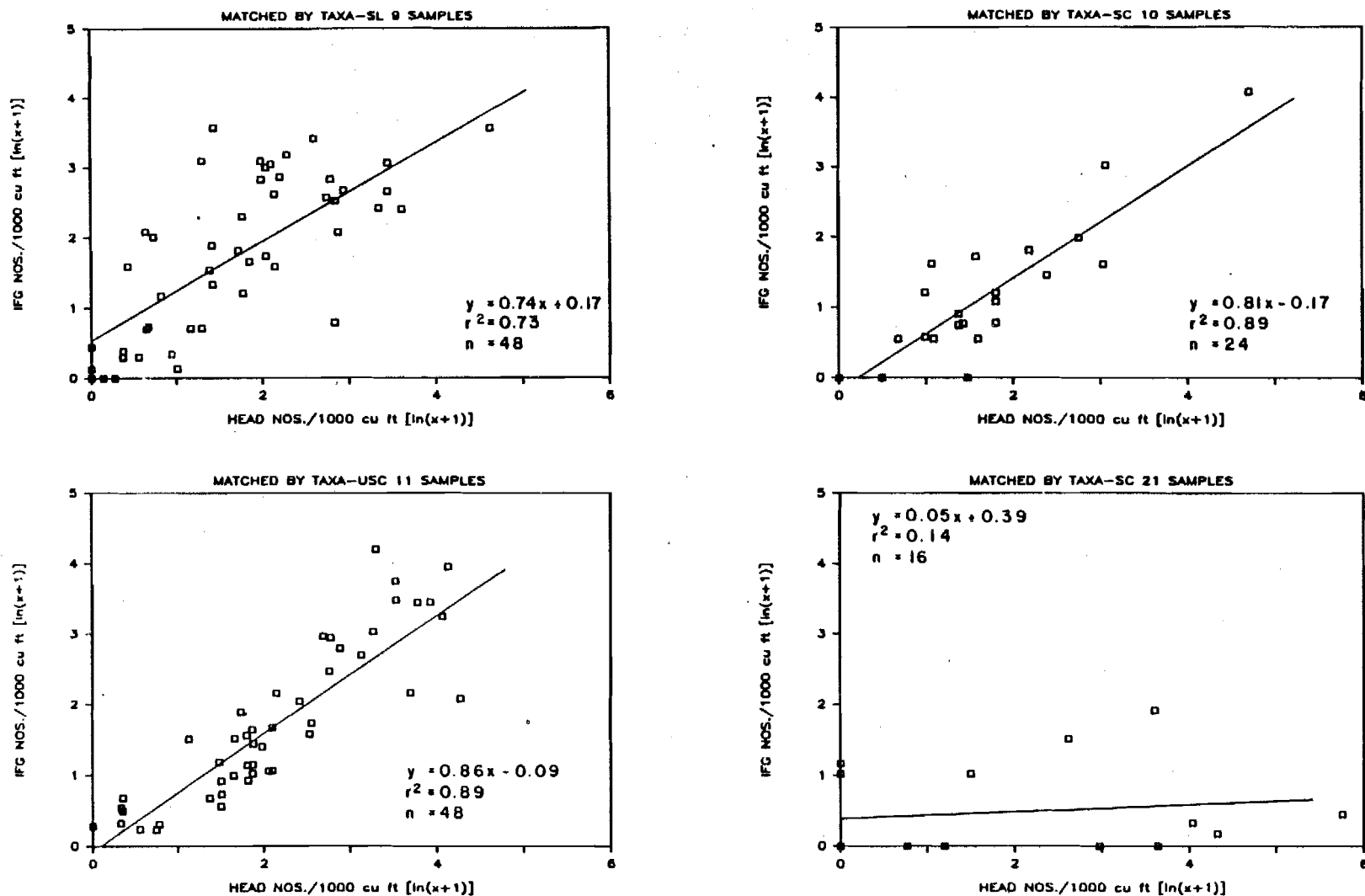
Figure 7. Scatter plots of standardized drift densities (no/1000 feet 3 of water) of eight invertebrate groups, head numbers vs. IFG-4 numbers. Densities are transformed \log_e (x+1) .
