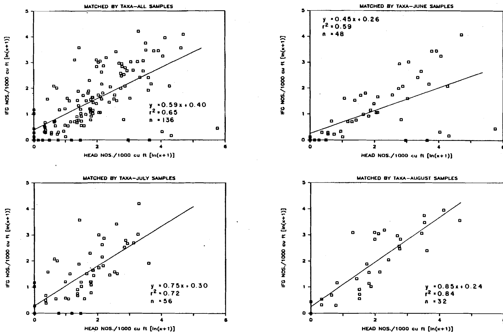
Figure 8. Scatter plots of standardized drift densities (no/1000 feet 3 of water) of eight invertebrate groups, head numbers vs. IFG-4 numbers. Densities are transformed \log_e (x+1) .
