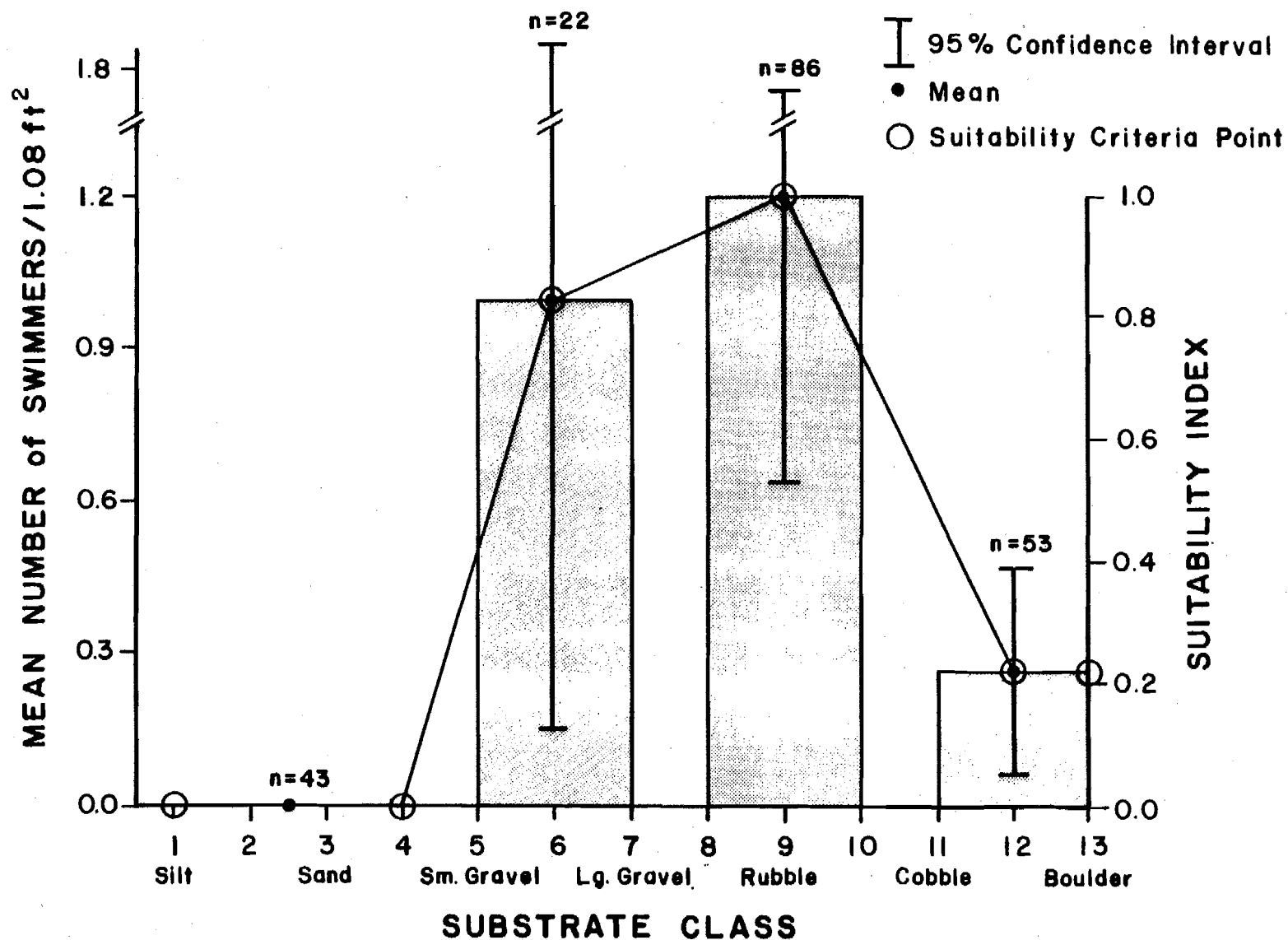
Figure 19. Average number of swimmer invertebrates per benthic sample for each substrate increment, with hand fitted suitability curve, middle Susitna River, Alaska, 1984.
