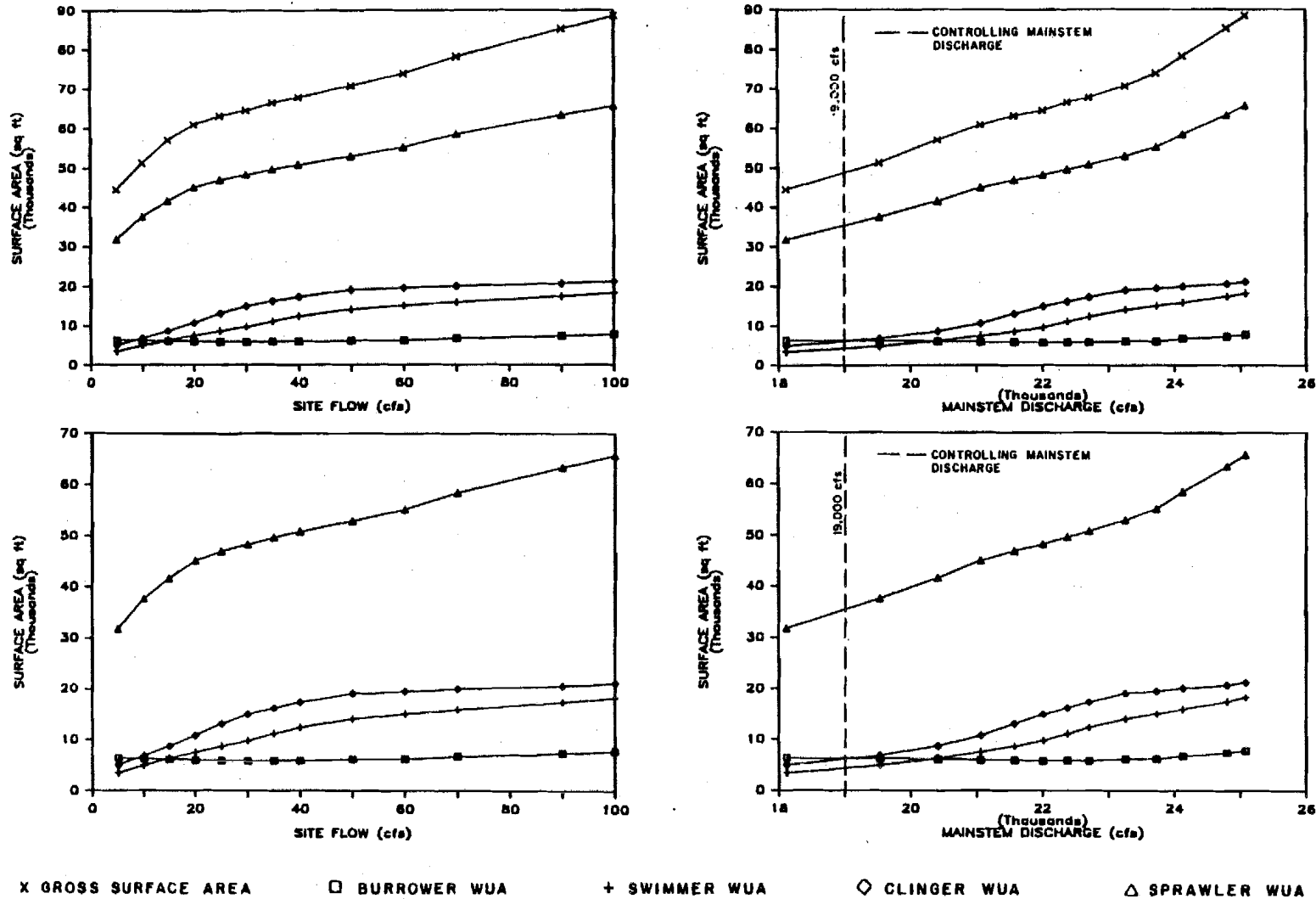
Figure 23. Projections of gross surface area and WUA of burrower, swimmer, clinger, and sprawler invertebrate habitat as a function of site flow and mainstem discharge for the Side Channel 10 modelling site.
