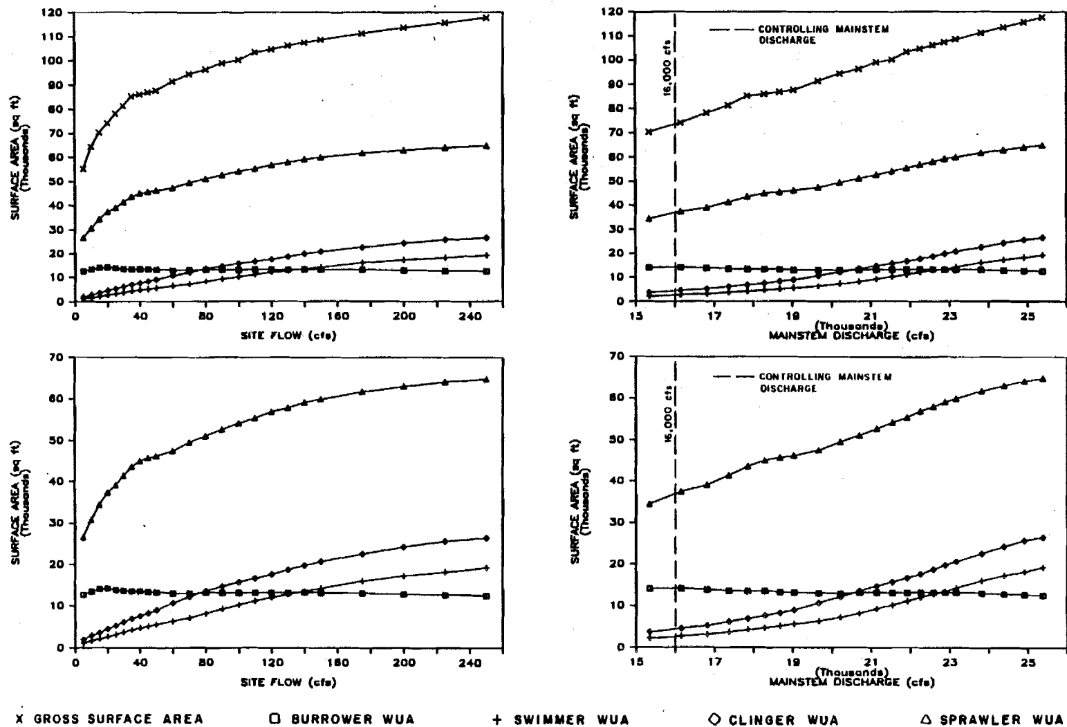
Figure 24. Projections of gross surface area and WUA of burrower, swimmer, clinger, and sprawler invertebrate habitat as a function of site flow and mainstem discharge for the Upper Side Channel 11 modelling site.
