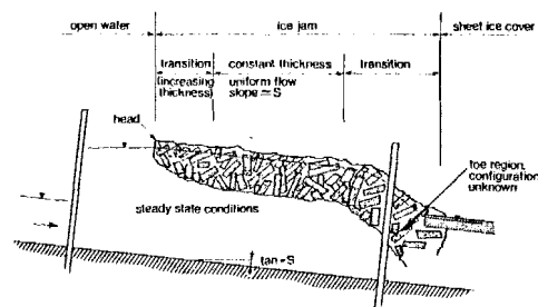
FIG. 1.—Schematic Illustration of Equilibrium Jam
