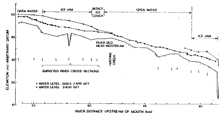
FIG. 6.—Profiles of Lower Smoky River under Open-Water and Breakup (Apr. 1977) Conditions (38-56 km above Mouth)
