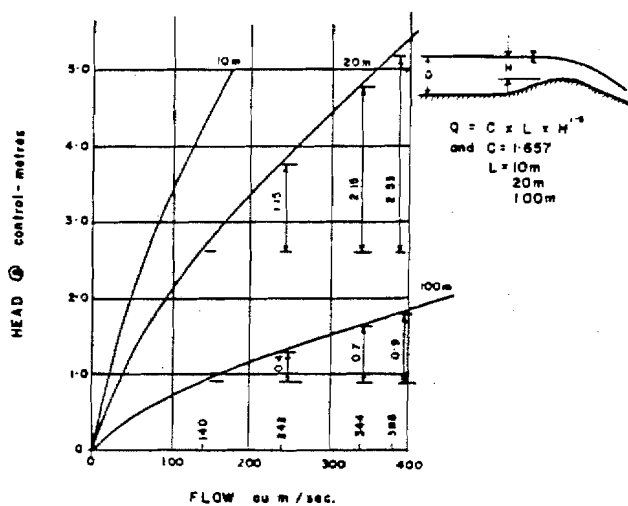
TYPICAL WATER LEVEL DISCHARGE CURVES
