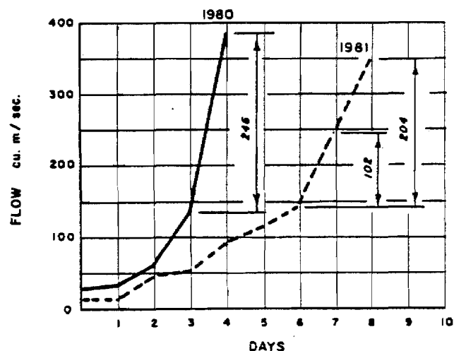
RIDEAU RIVER AT MANOTICK HYDROGRAPHS DURING ICE BREAK-UPS
