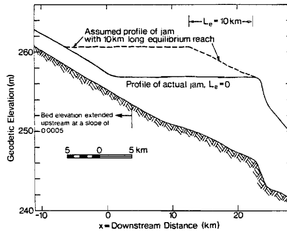
FIG. 7. Illustration of initial hypothetical jam with an equilibrium reach.
