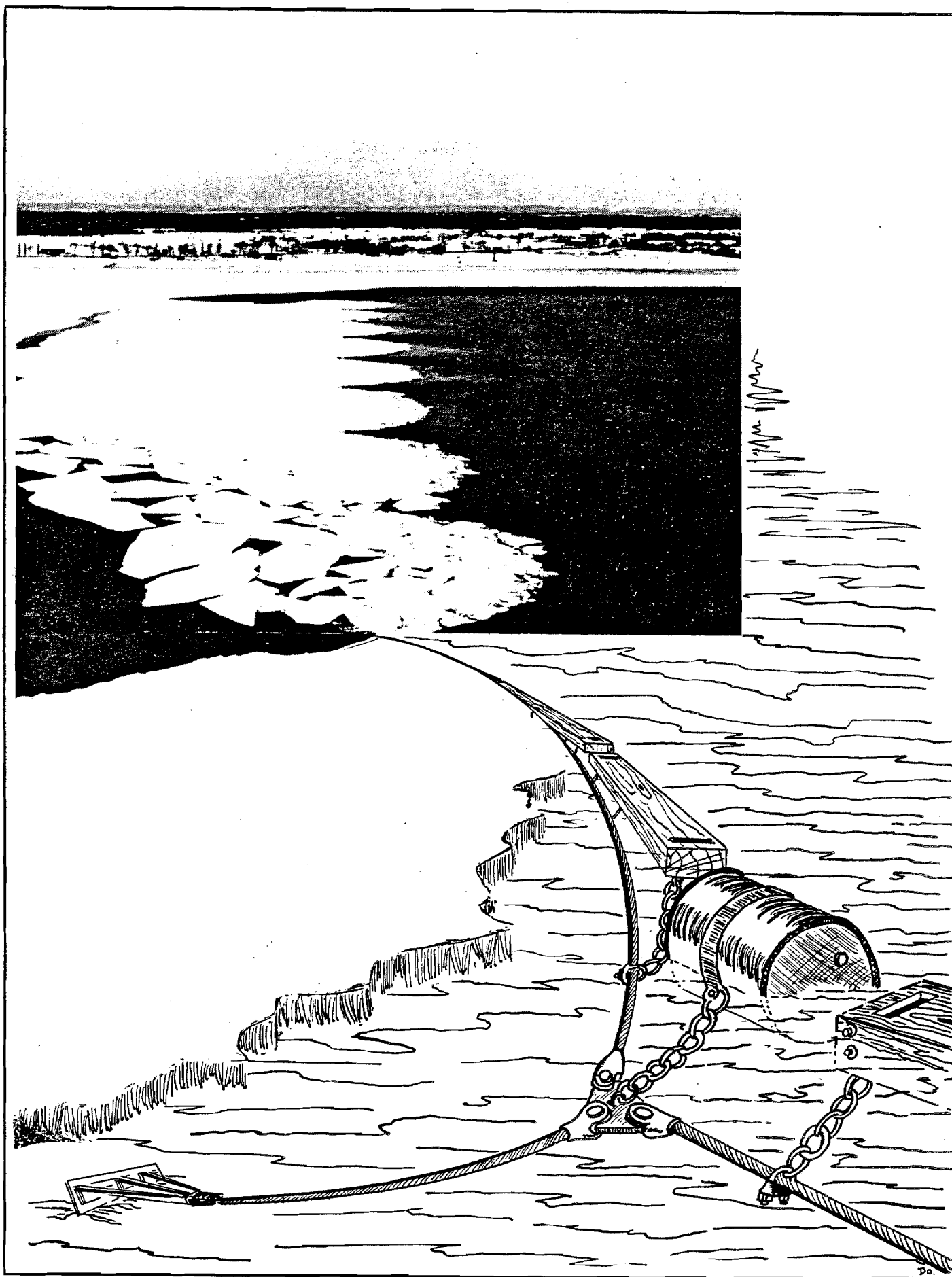
TYPICAL ICE BOOM ARRANGEMENT
