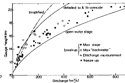
FIG. 11.—Freeze Up and Breakup Stages versus Discharges; Thames River at Thamesville ( W = 40-65 m; S = 0.00023 )
