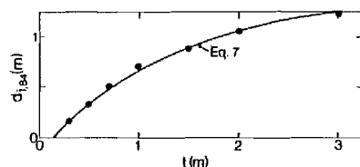
FIG. 4.—Variation of d_{i,84} with t as deduced from Nezhikovskiy's Results
