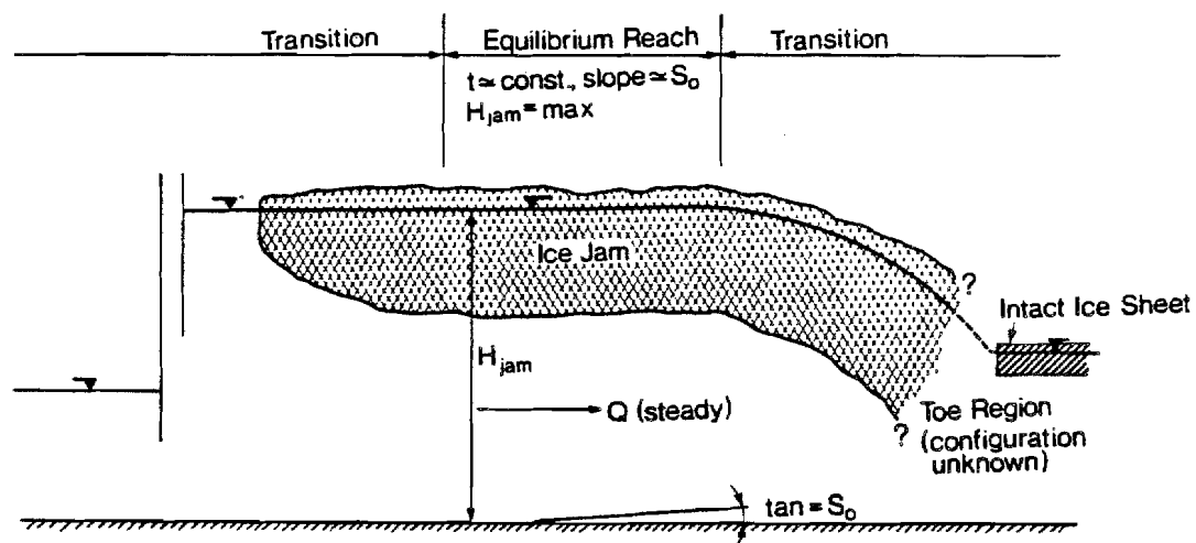
Fig. 5. Profile of a jam with an equilibrium reach
