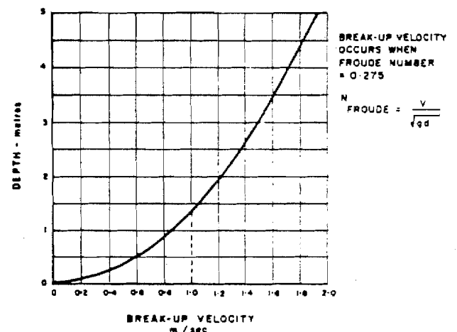
DEPTH AND BREAK-UP VELOCITY CURVE
