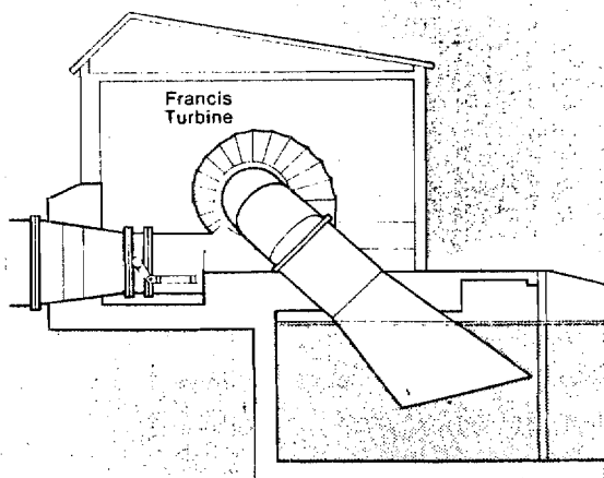
Nohab Tampella Francis turbine: Head range up to 100 m; discharge range up to 30 m 3 /s.
