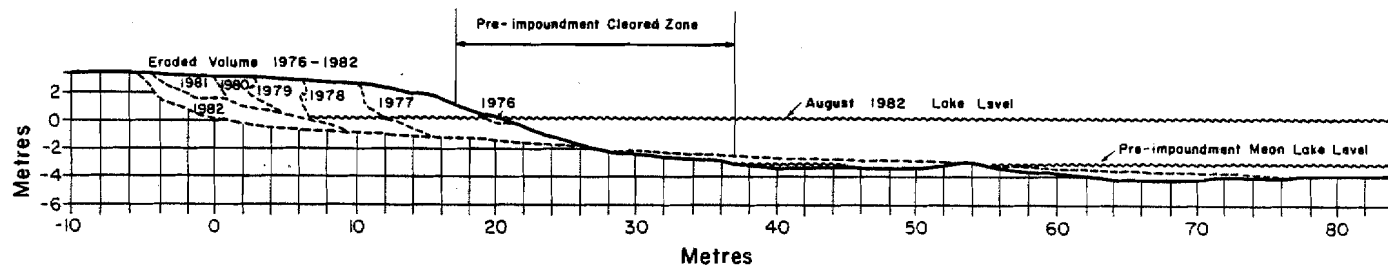
FIG. 3. Cross-section of an eroding shoreline on Southern Indian Lake that was cleared of timber before flooding. Material removed succeeding years is indicated by broken line on bank cross-section. Material deposited nearshore is indicated by broken line under the new water level. Note that the shoreline zone cleared of timber was eroded away within 1 yr of flooding.
