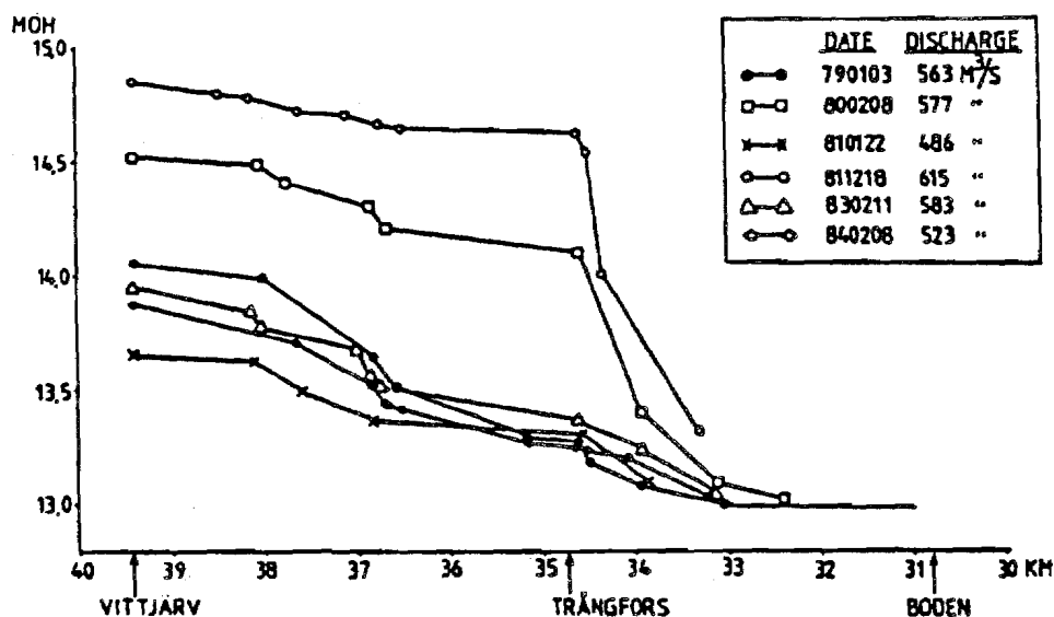
Figure 3. Measured water surface profiles for winters after 1978.
