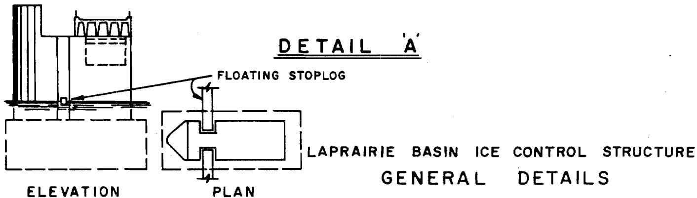
TYPICAL PIER
