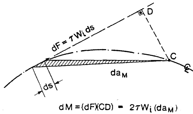
(b) ELEMENTARY FORCE ( dF ) AND BENDING MOMENT ( dM )
