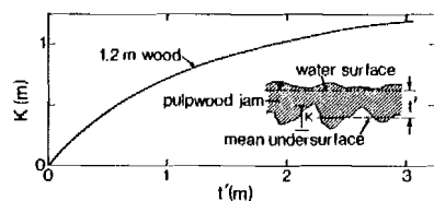
FIG. 3.—Kennedy's Roughness-Thickness Relationship for Log Jams (Note t' = s_w t ; s_w = Specific Gravity of Wood)
