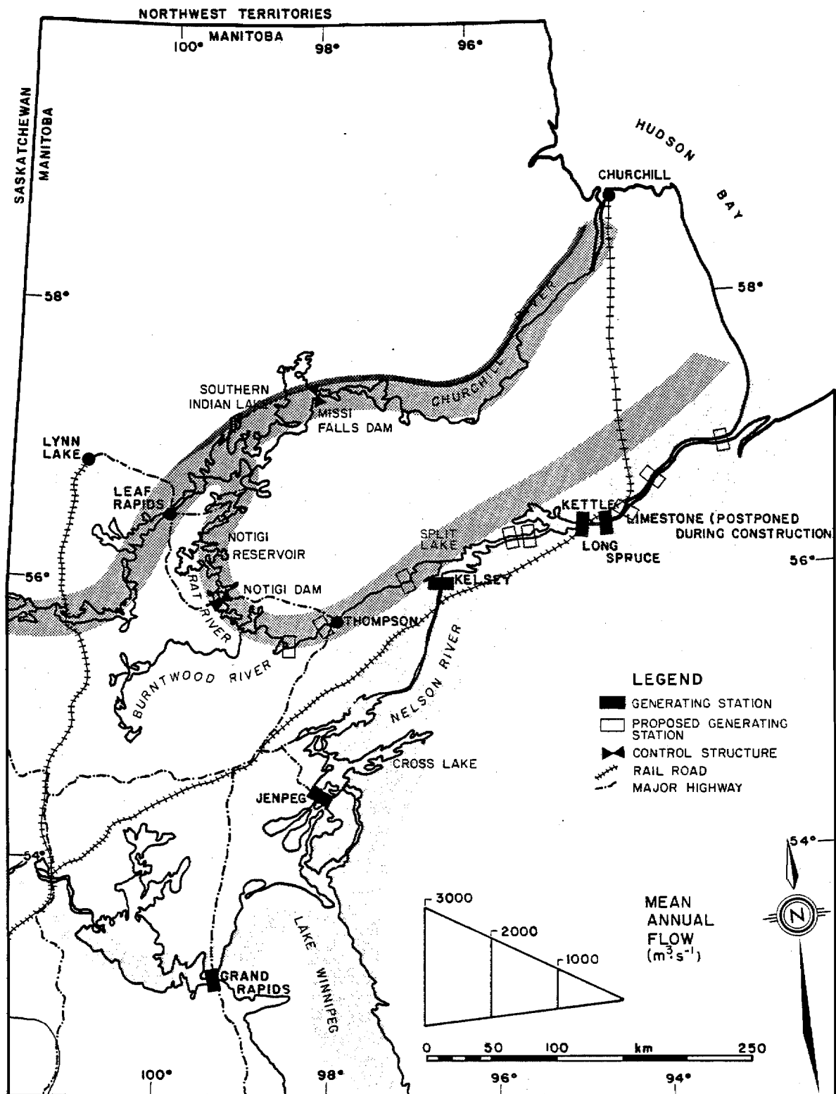
FIG. 2. Churchill and Nelson rivers hydroelectric development, indicating the altered flow regime of the rivers. Dark tone indicates relative magnitude of lower Churchill River discharge remaining after diversion; mid-tone indicates portion of Churchill River discharge diverted at Southern Indian Lake; light tone indicates Nelson River discharge.
