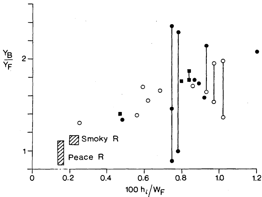
Fig. 9. Test of Eq. 9, Y_B/Y_F versus h_i/W_F ; legend same as for Fig. 8.
