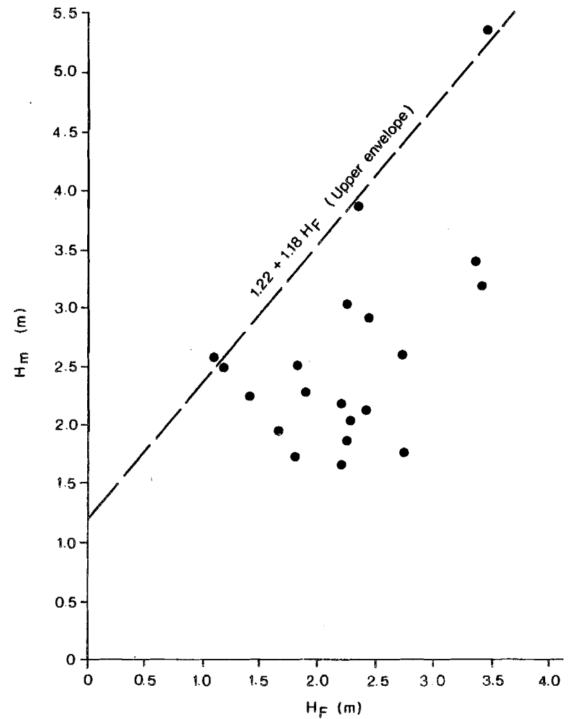
Fig. 6. Maximum stage during breakup versus H_F .
