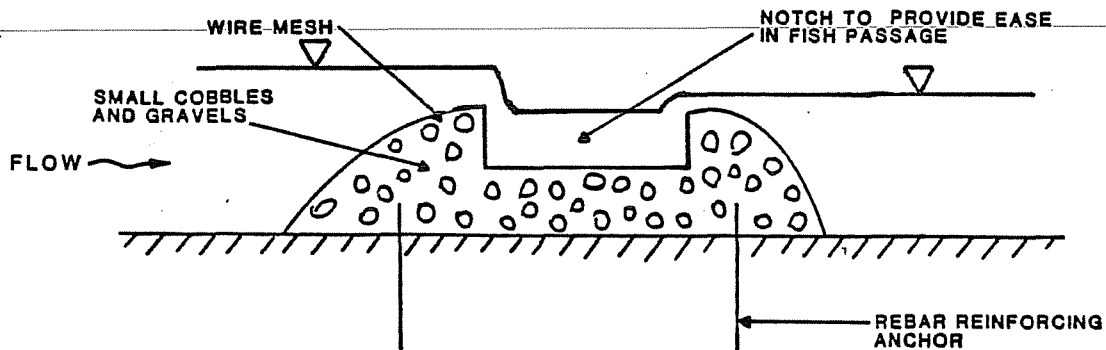
GABION BARRIER
