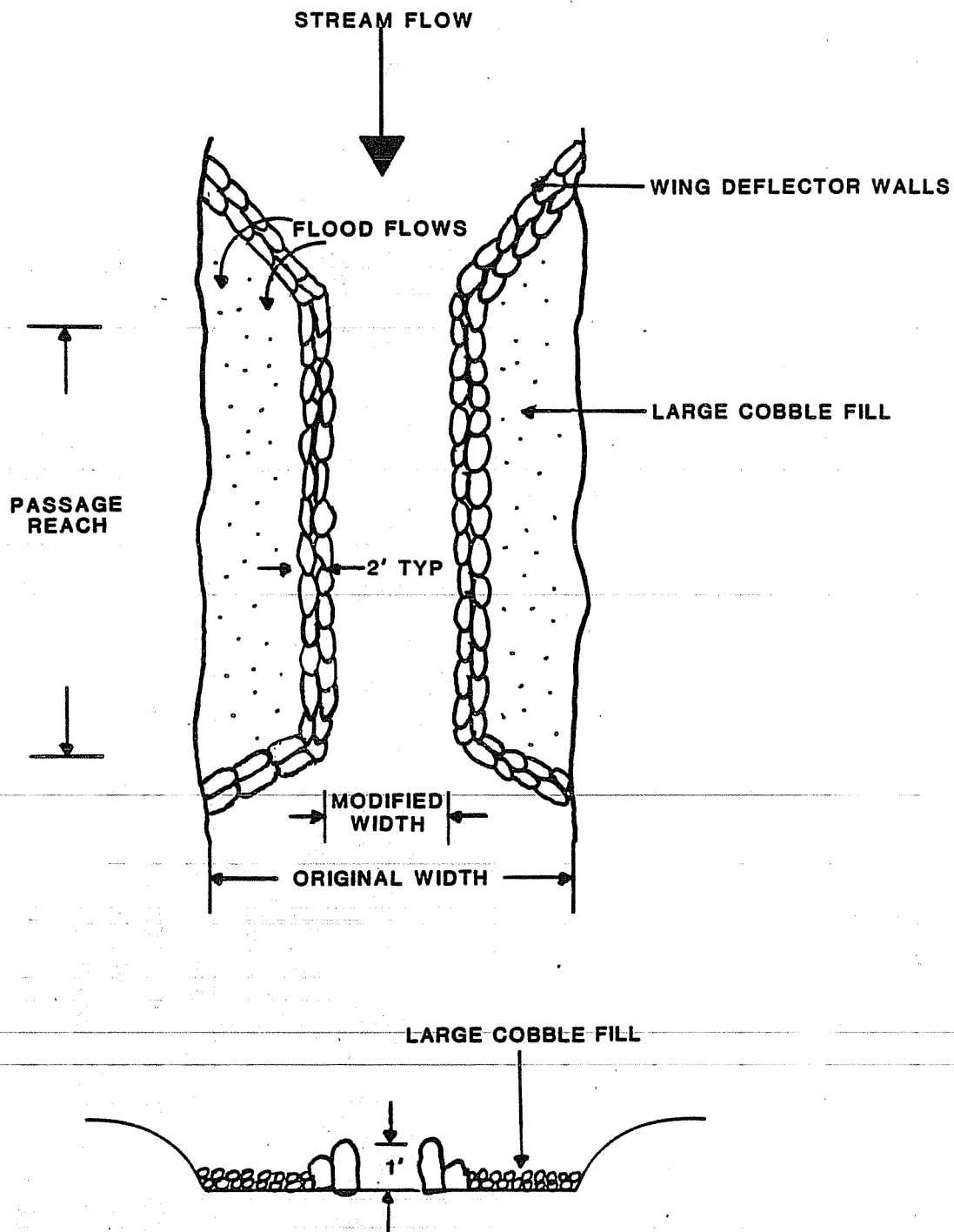
FIGURE 16 WING DEFLECTOR
