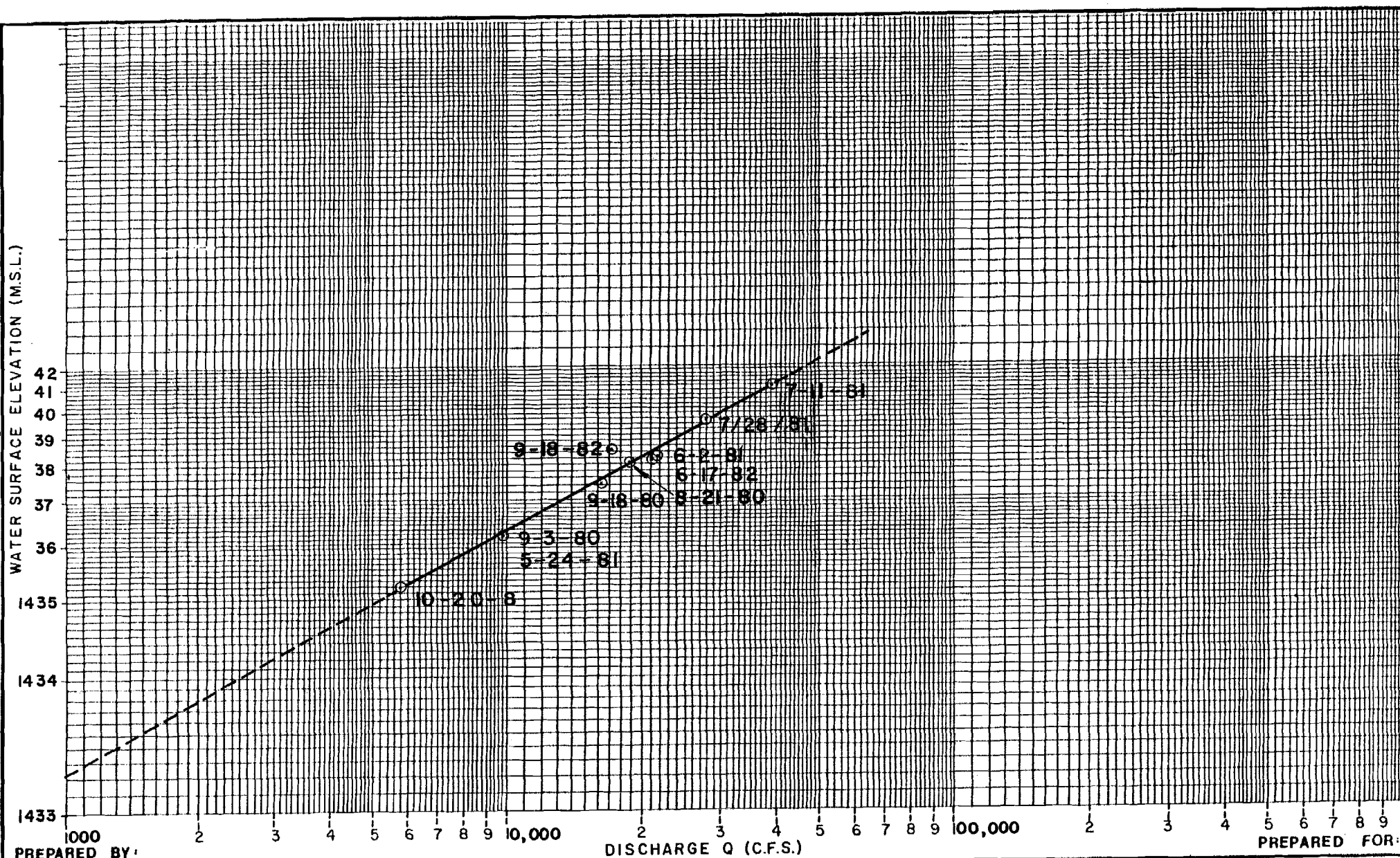
STAGE DISCHARGE RATING CURVE SUSITNA RIVER NEAR WATANA
