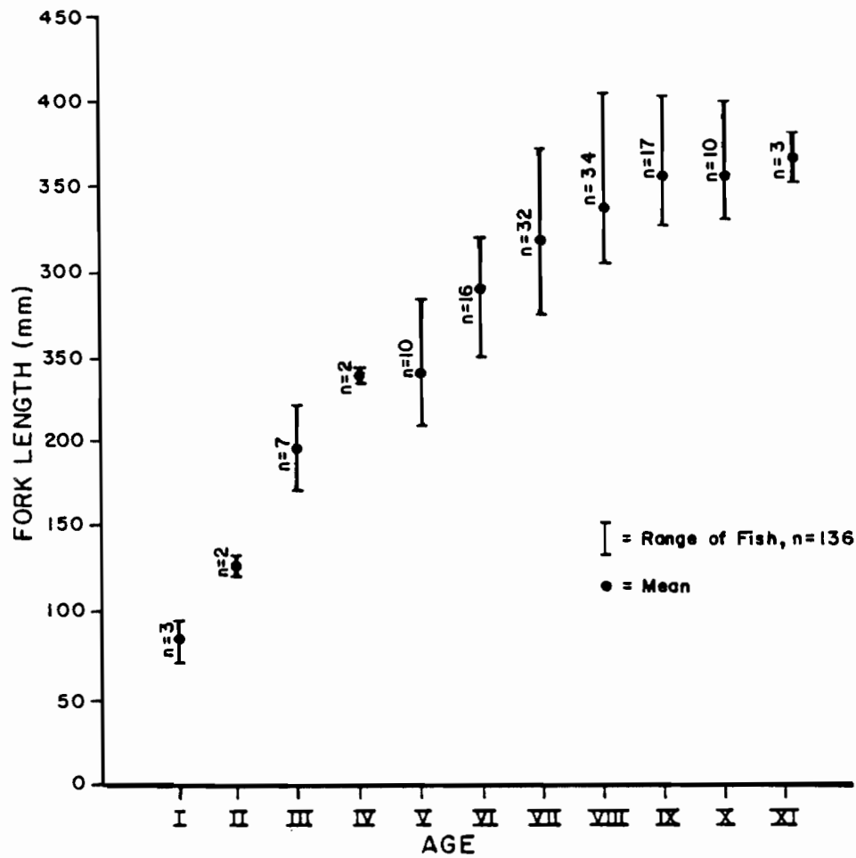
Appendix Figure E-19. Age and length relationship for longnose suckers captured in the Susitna River between the Chulitna River confluence and Devil Canyon, May to October 1983.
