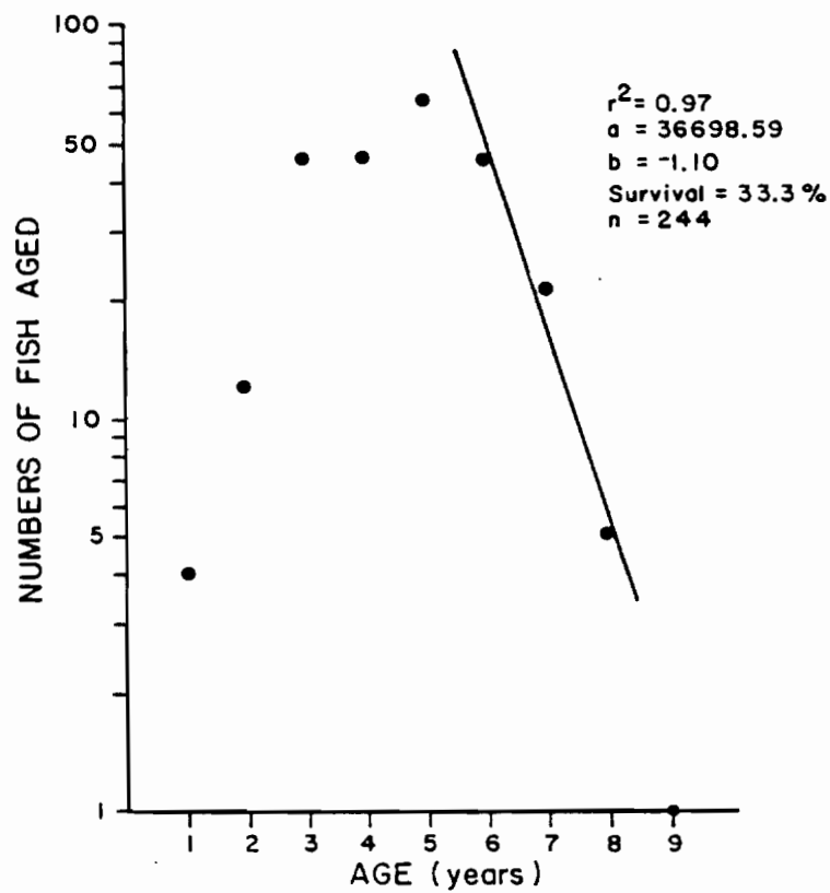
Appendix Figure E-4. Instantaneous survival rate curves calculated for rainbow trout captured in the Susitna River between the Chulitna River confluence and Devil Canyon, 1983.
