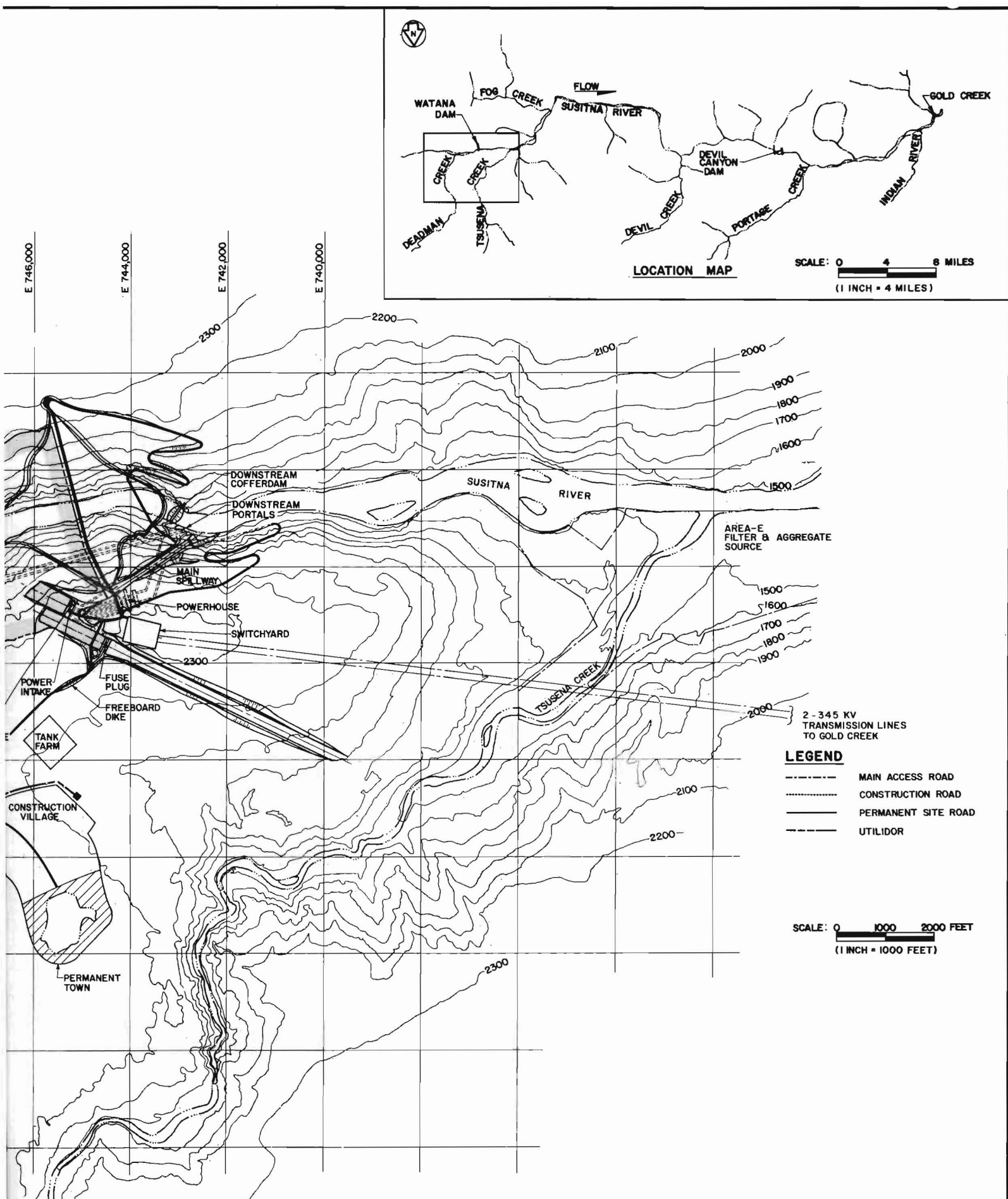
LAYOUT SITE FACILITIES
