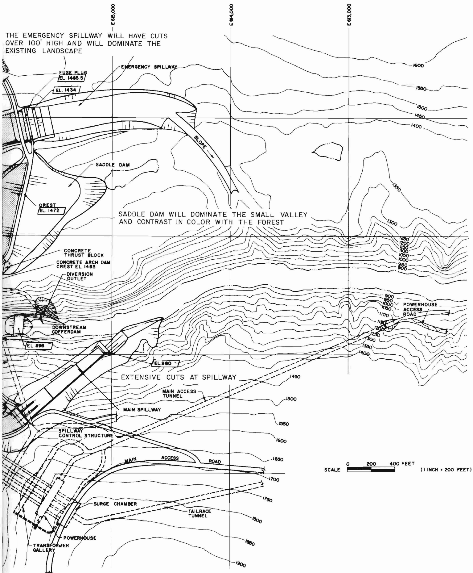
GENERAL ARRANGEMENT
