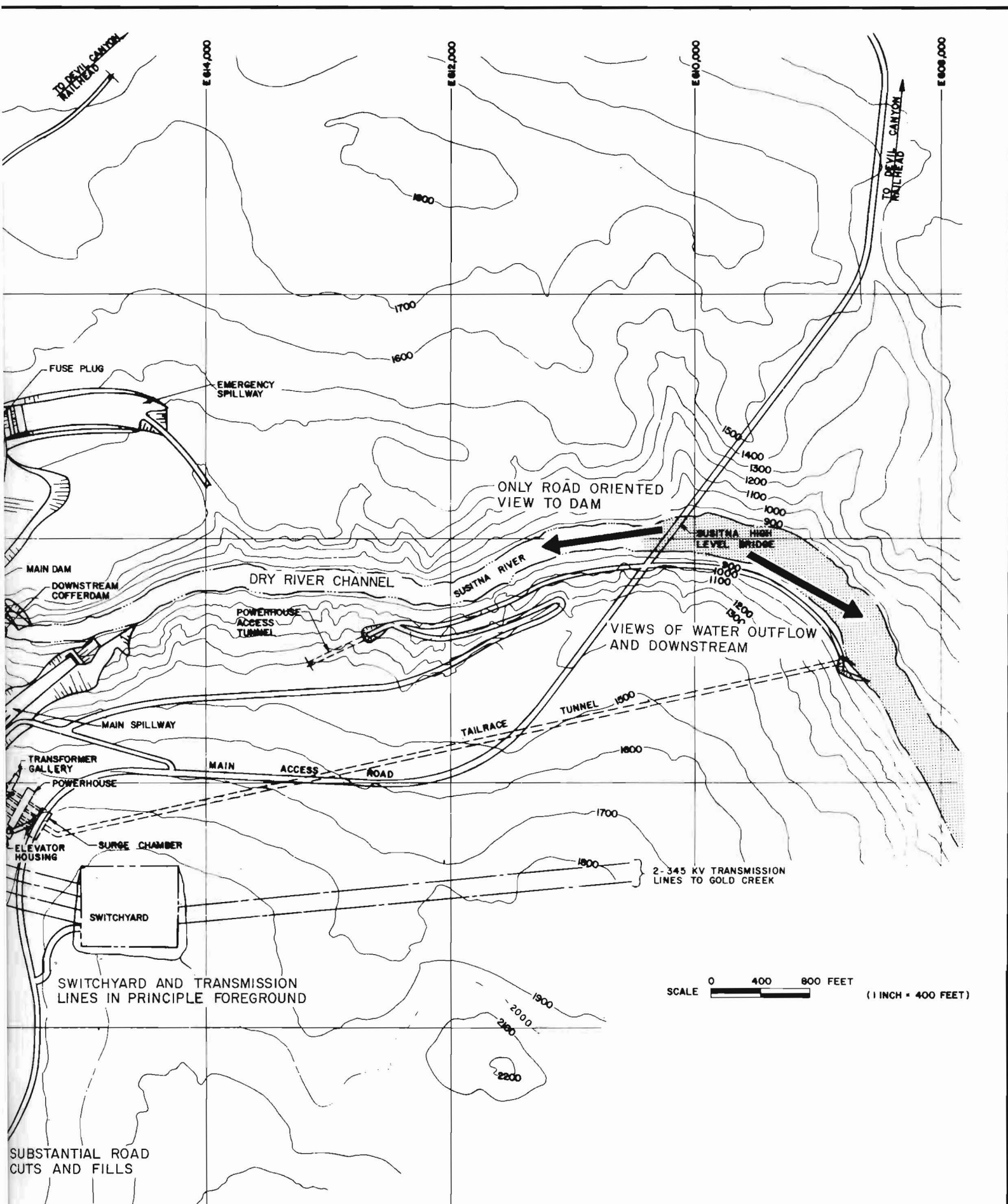
YON SITE LAYOUT
