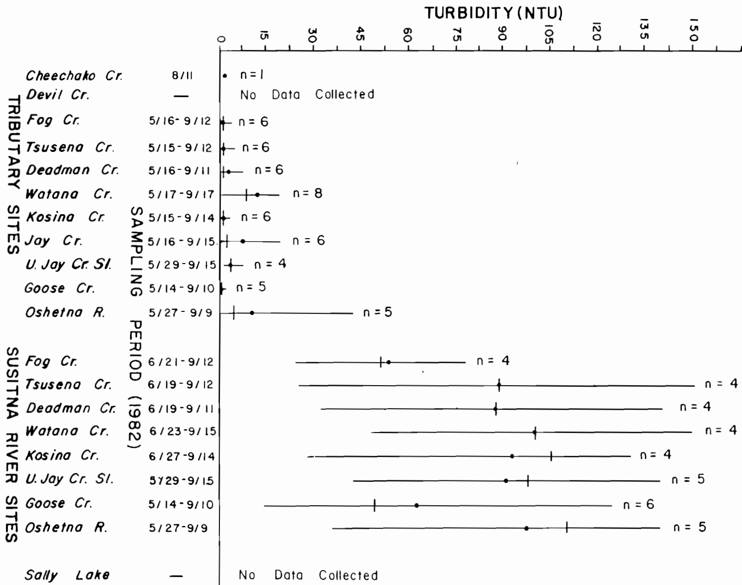
Figure 3-5-7 Mean (•), range (|) and median (—) turbidity values recorded at selected habitat evaluation sites within the proposed impoundment areas during the 1982 open water field season (n = the number of observations).
