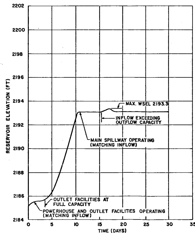
1:10,000 YEAR FLOOD
