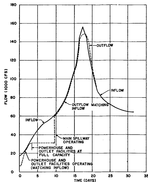
1:10,000 YEAR FLOOD
