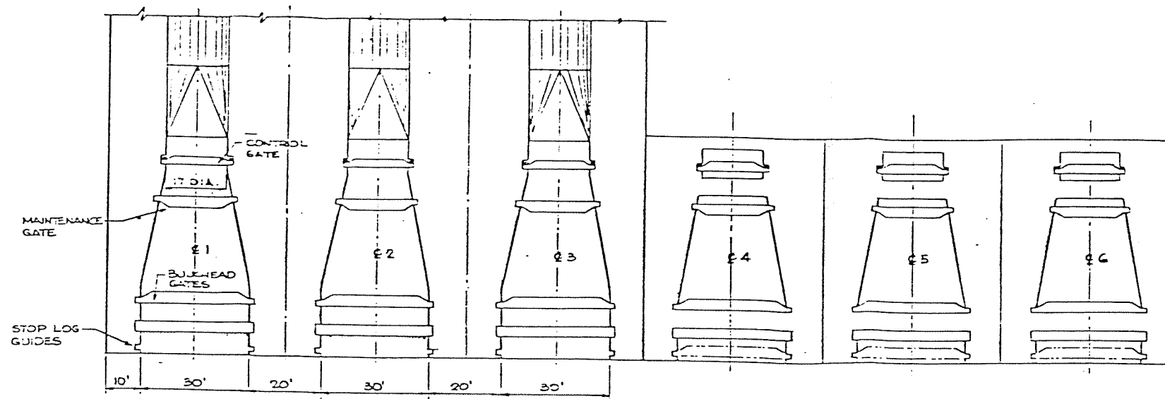
PLAN AT EL. 2021
