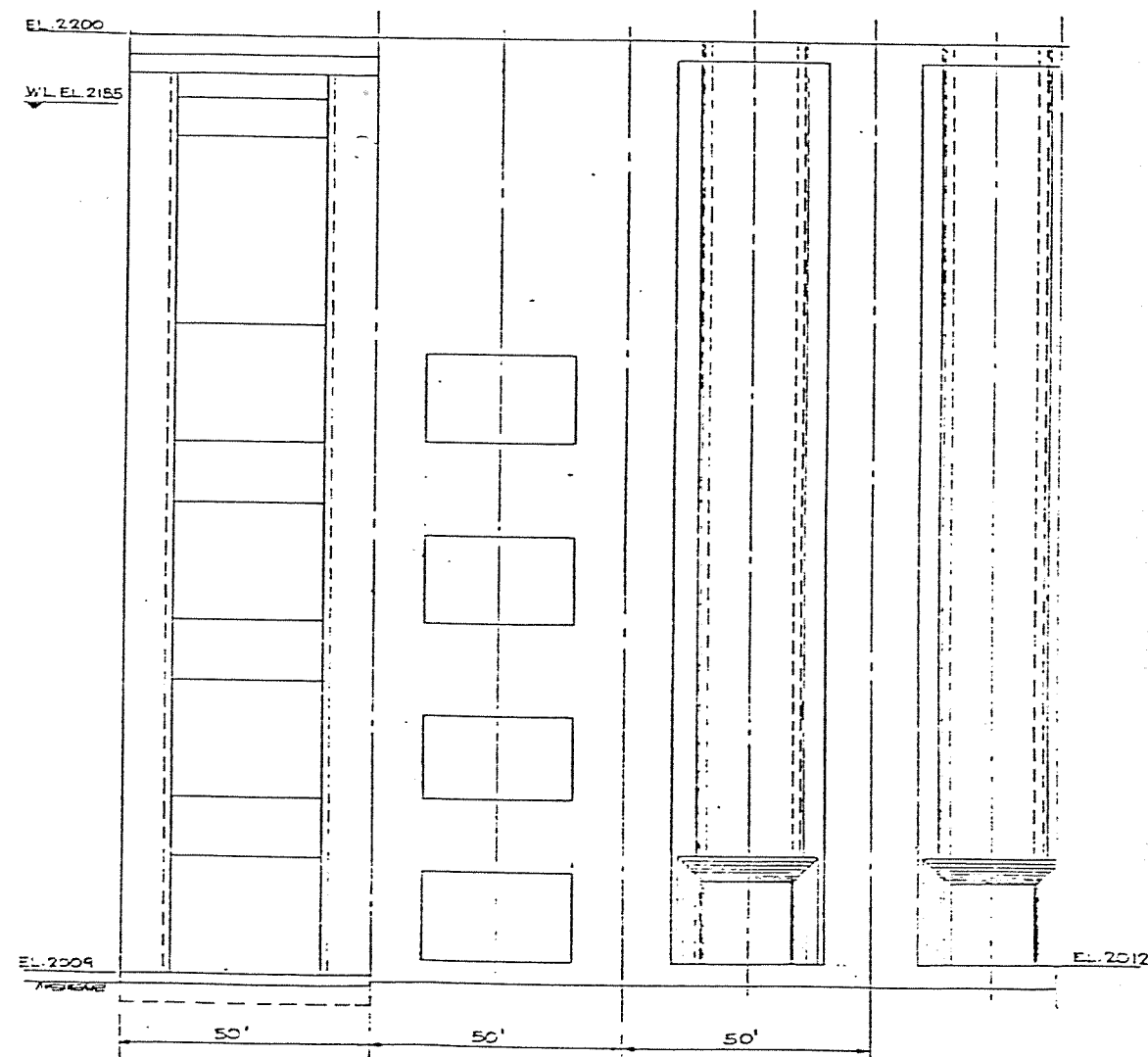
FRONT ELEVATION
