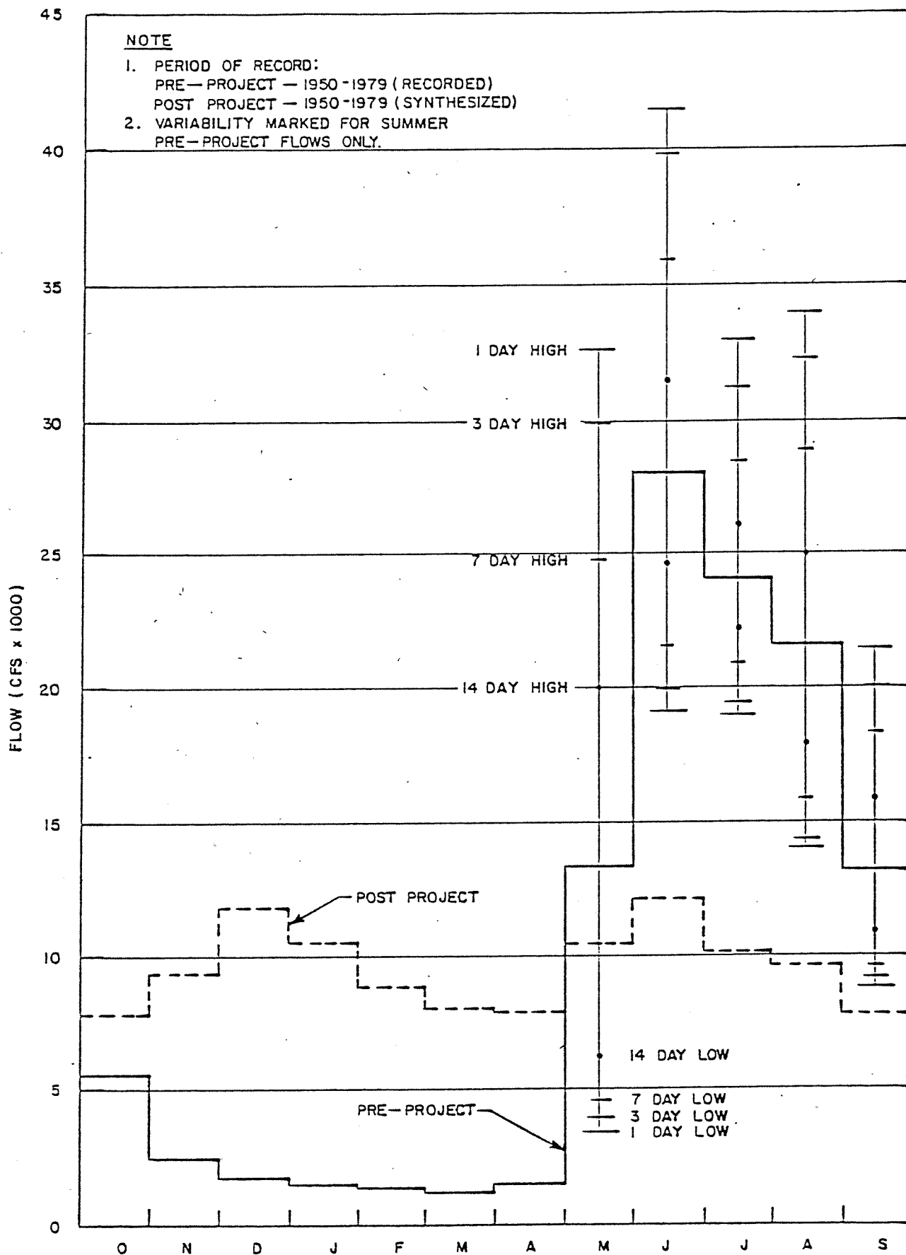
PRE AND POST PROJECT FLOWS SUSITNA RIVER AT GOLD CREEK
