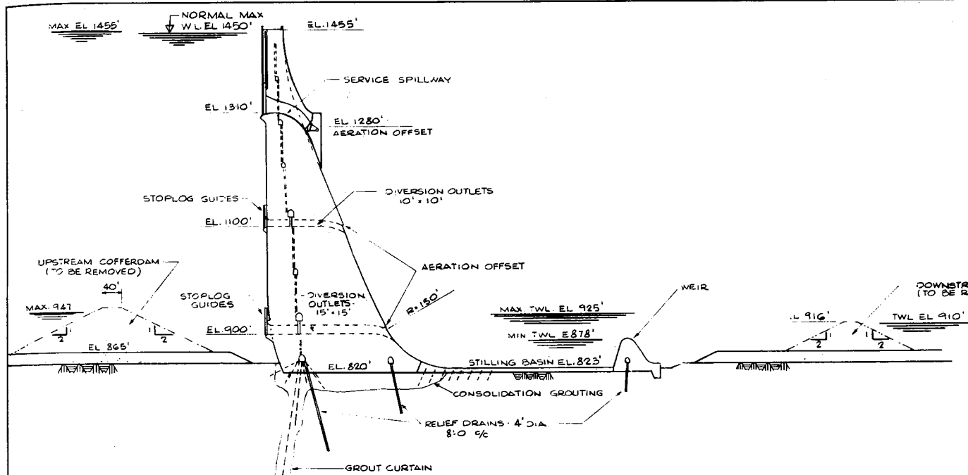
ARCH-GRAVITY DAM LAYOUT
