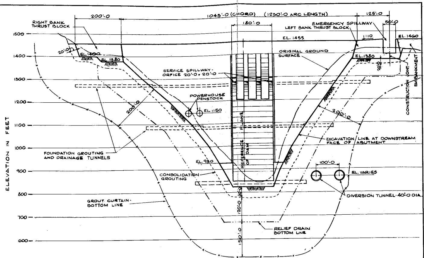
DOWNSTREAM ELEVATION OF DAM
