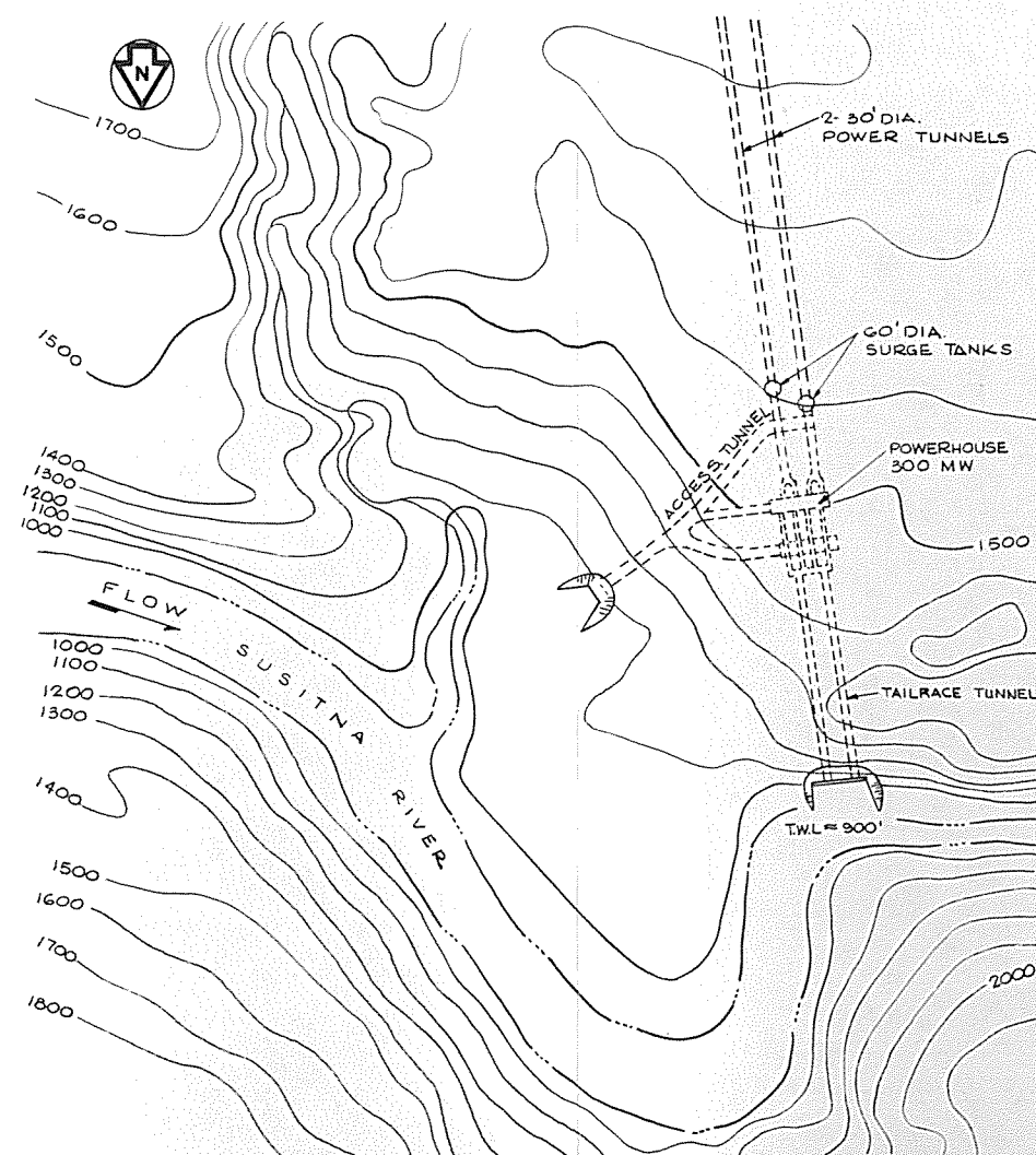
GENERAL ARRANGEMENT DEVIL CANYON POWERHOUSE
