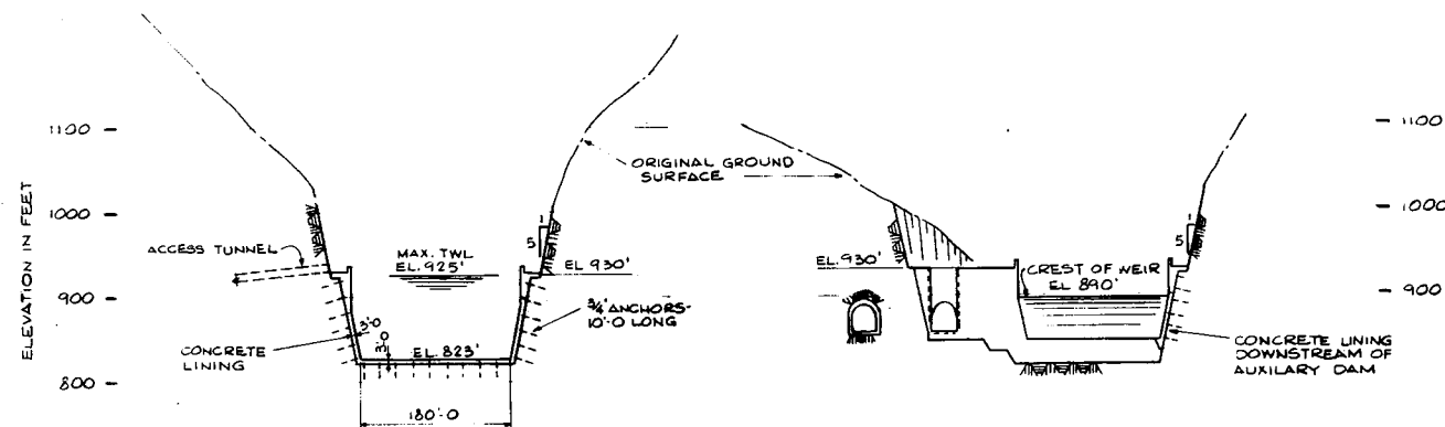
SECTION AT WEIR
