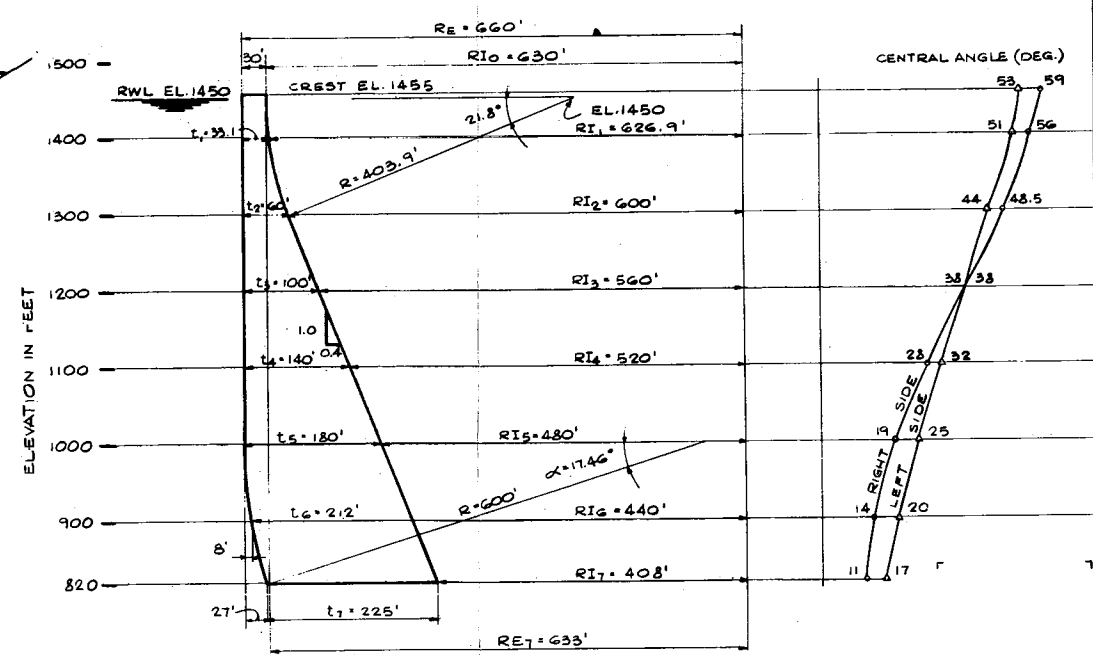
ARCH GRAVITY DAM GEOMETRY
