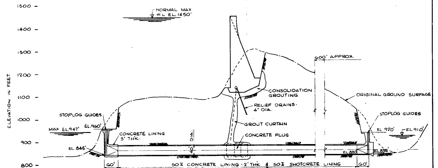
SECTION THRU DIVERSION TUNNEL
