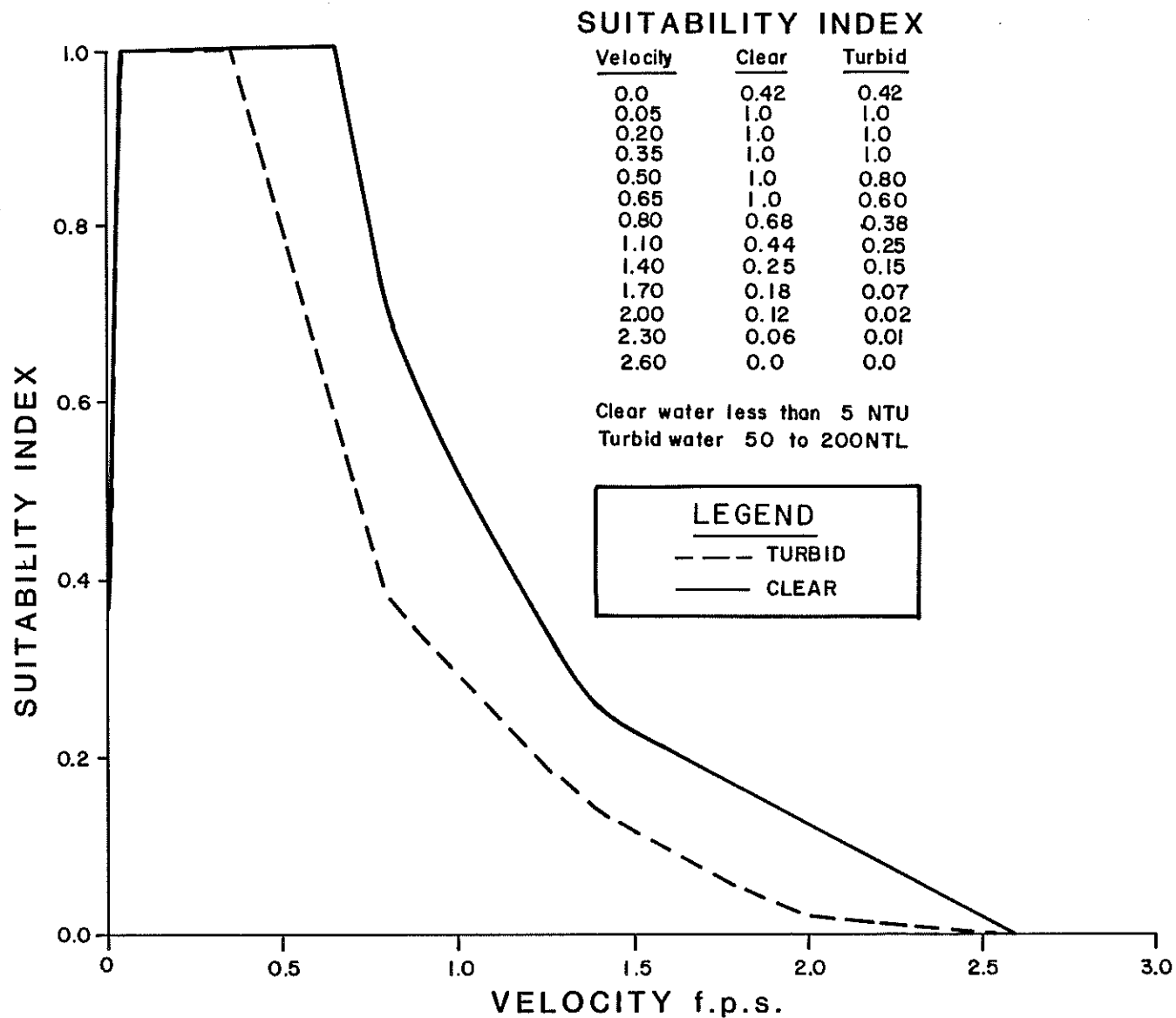
JUVENILE CHINOOK SALMON SUITABILITY CRITERIA FOR VELOCITY APPLICABLE TO CLEAR AND TURBID WATER HABITATS.
