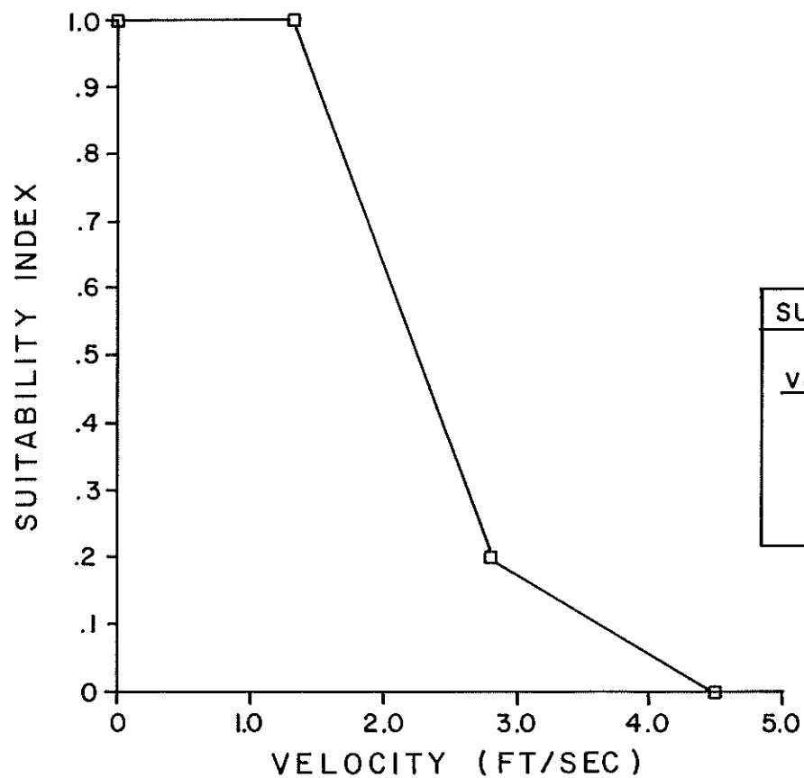
VELOCITY SUITABILITY CURVE FOR CHUM SALMON SPAWNING.
