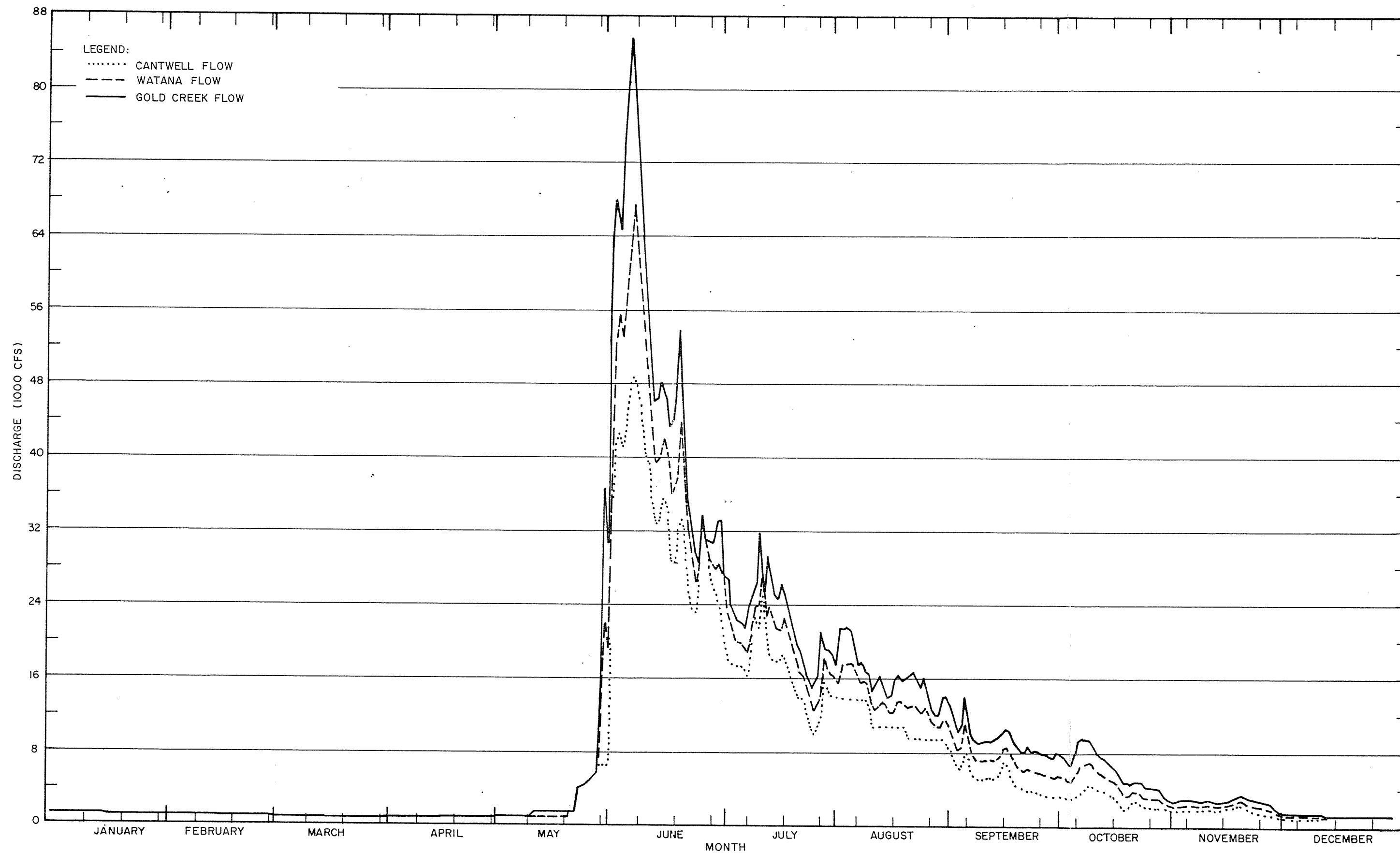
1964 NATURAL FLOWS CANTWELL, WATANA AND GOLD CREEK
