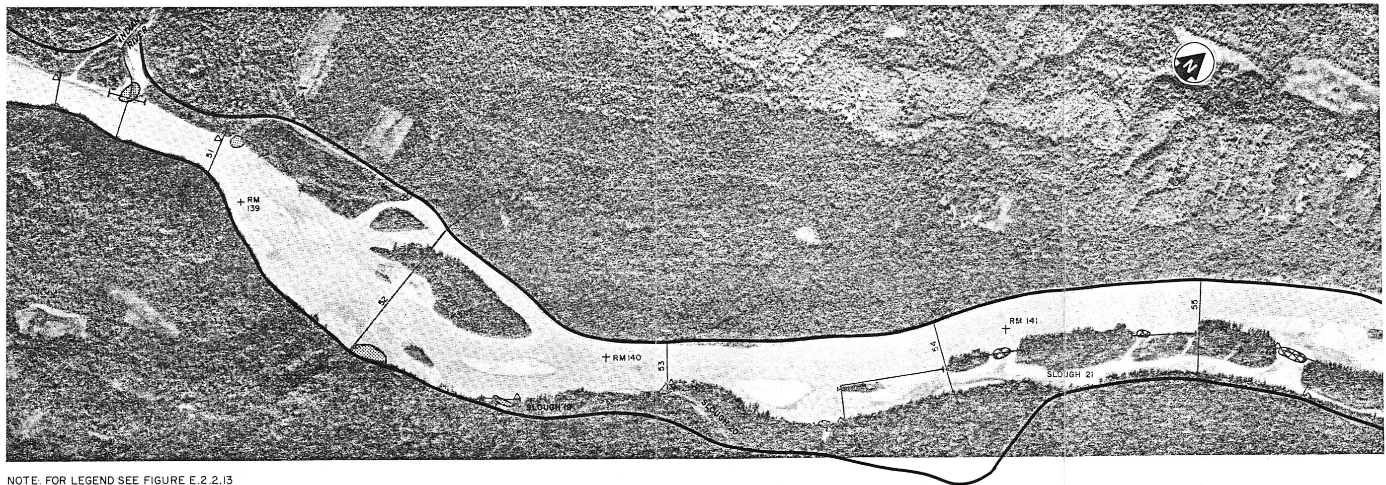
SUSITNA RIVER PLAN RM 145 TO RM 139
