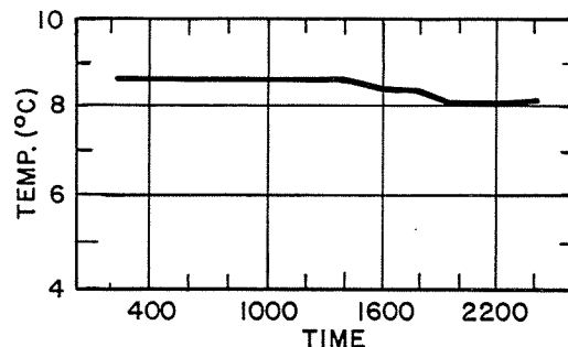
SUSITNA RIVER AT PORTAGE CREEK (RM 149)
