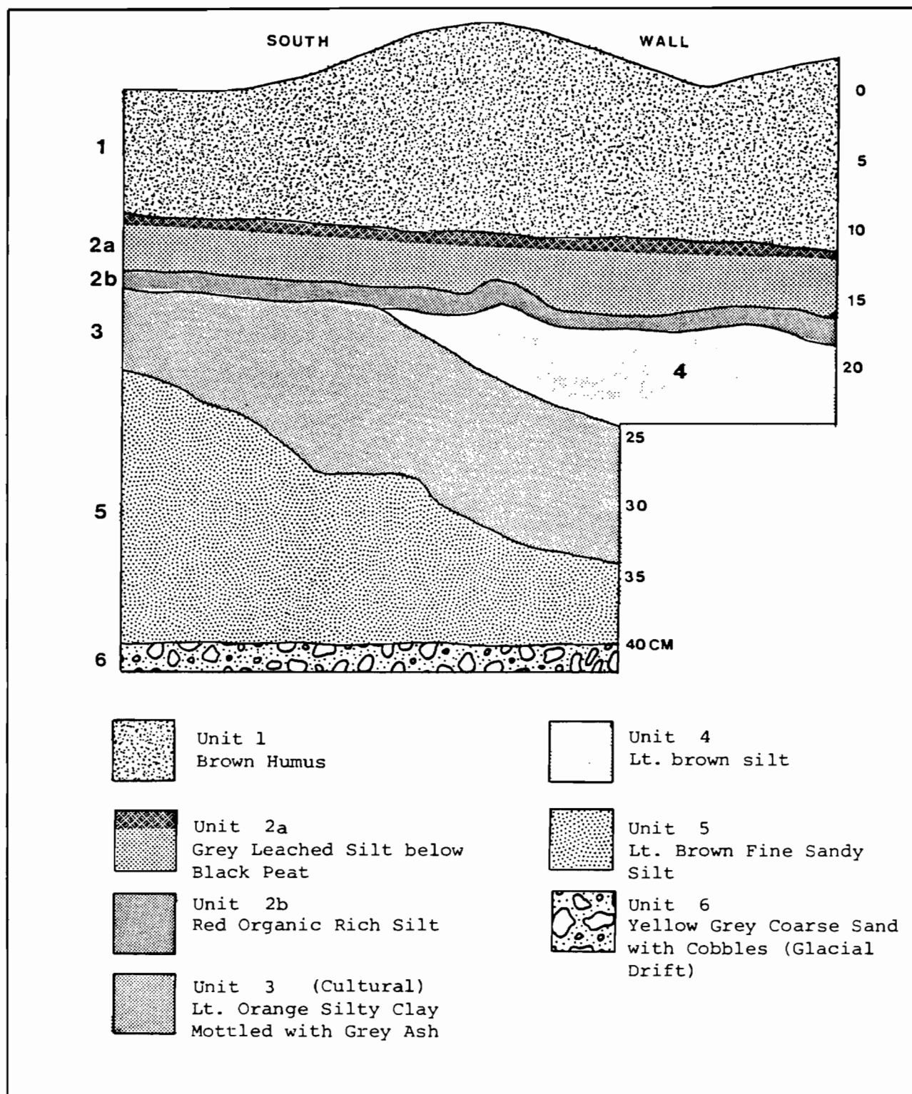
Figure 23 Soil profile UA80-76 (TLM 029), test 1.
