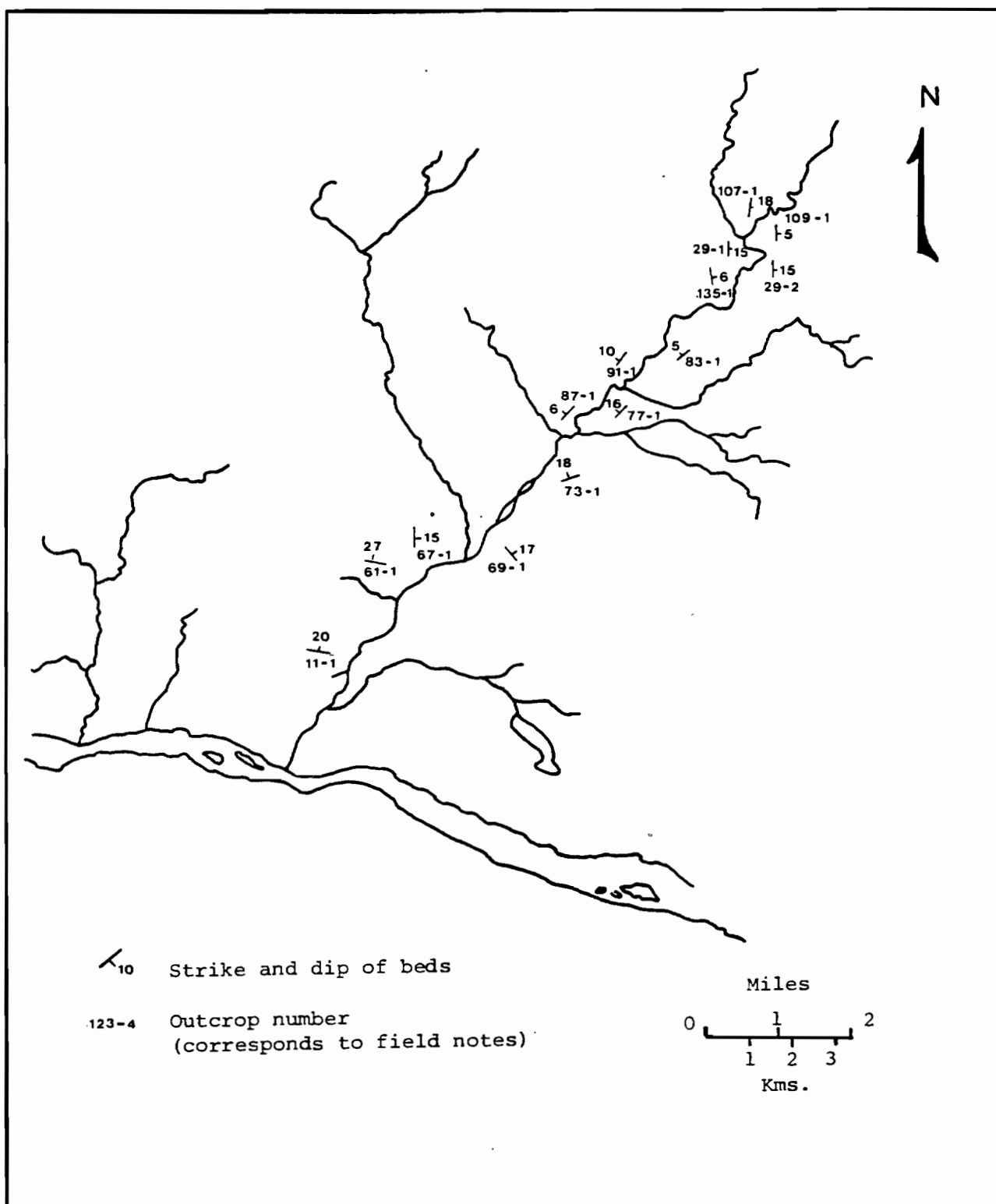
Figure 93. Location of outcrops. 251
