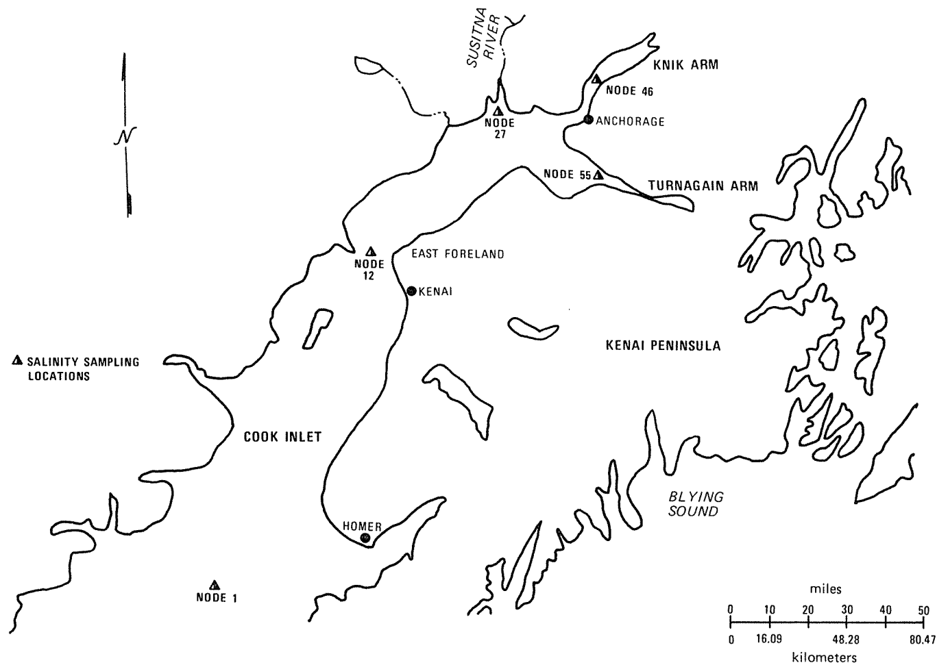
Figure H.5 -1. Locations of sampling stations for salinity in Cook Inlet (Exhibit E, Chapter 2).
