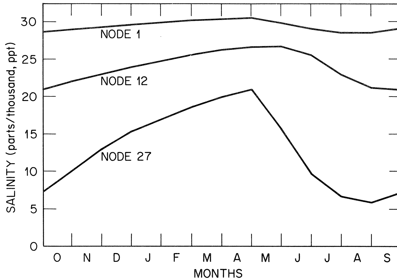
Figure H.5-2. Seasonal pattern in the salinity of water in Cook Inlet at nodes 1, 12, and 27. The location of the sampling stations (nodes) is illustrated in Figure H.5 -1 (Exhibit E, Table E.2.31).
