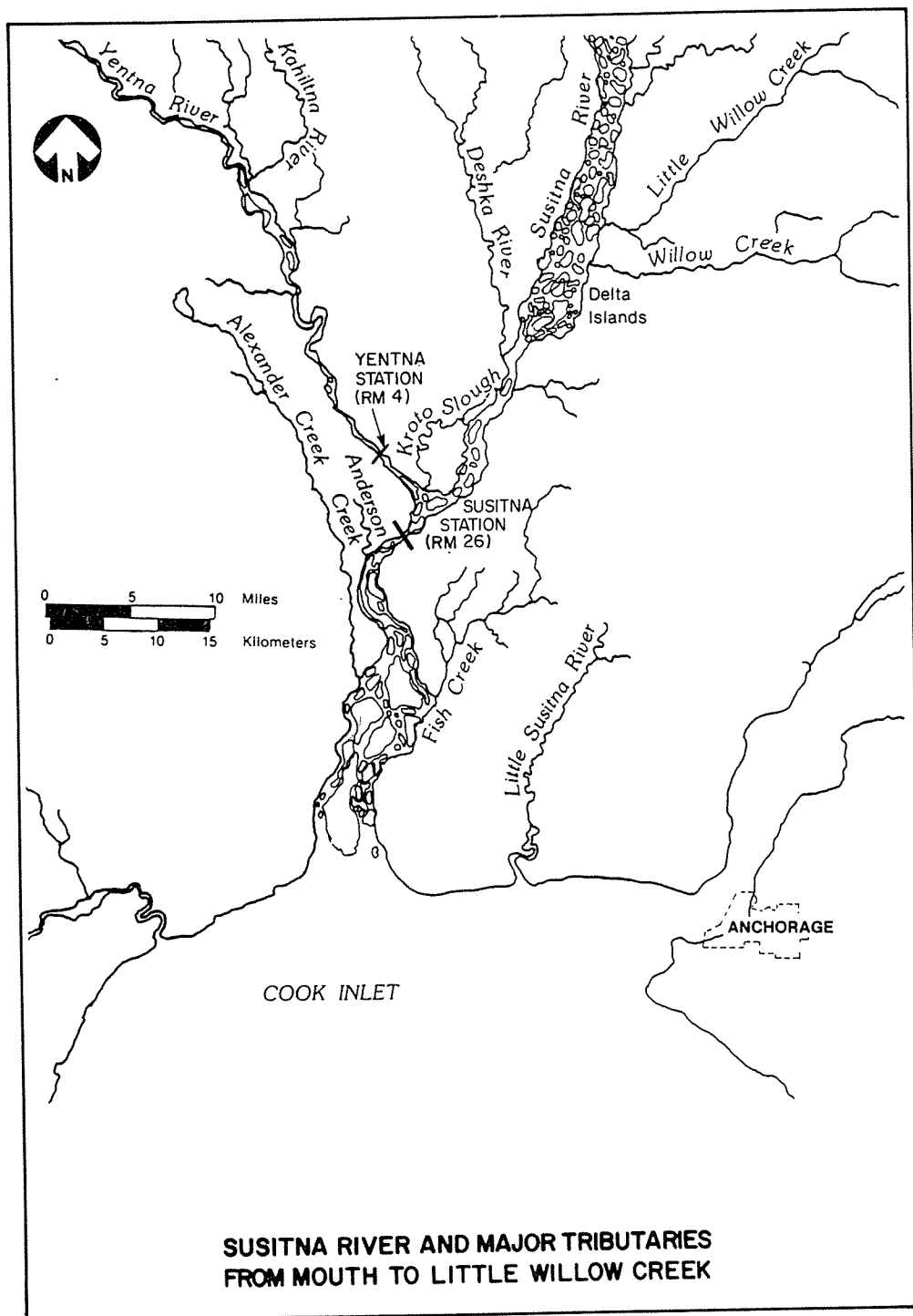
Figure I.1-11. Susitna River and Major Tributaries from Mouth to Little Willow Creek. Source: Exhibit E, Figure E.3.4.
