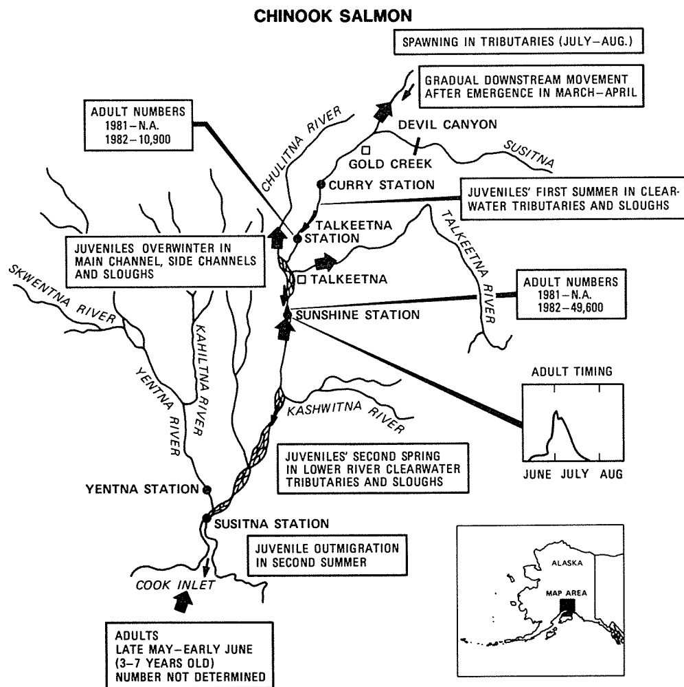
Figure I.1-3. Chinook Salmon ( Oncorhynchus tshawytscha ) - Generalized Life Cycle and Habitat Suitability in the Susitna River Drainage.
