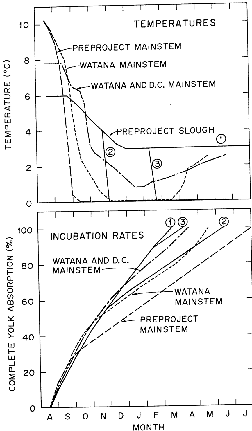
Figure I.2-2. Incubation rates for chum salmon spawned on August 15 under different temperature scenarios. (a) preproject mainstem at Sherman, (b) Sherman mainstem with Watana Dam alone, (c) Sherman mainstem with Watana and Devil Canyon dams, (d) intergravel in a preproject slough, (e) and slough intergravel at two overtopping dates, November and February. Mainstem temperatures were developed by the staff from the application. Slough temperatures and regression equations for incubation rate modeling were those of Wangaard and Berger (1983).
