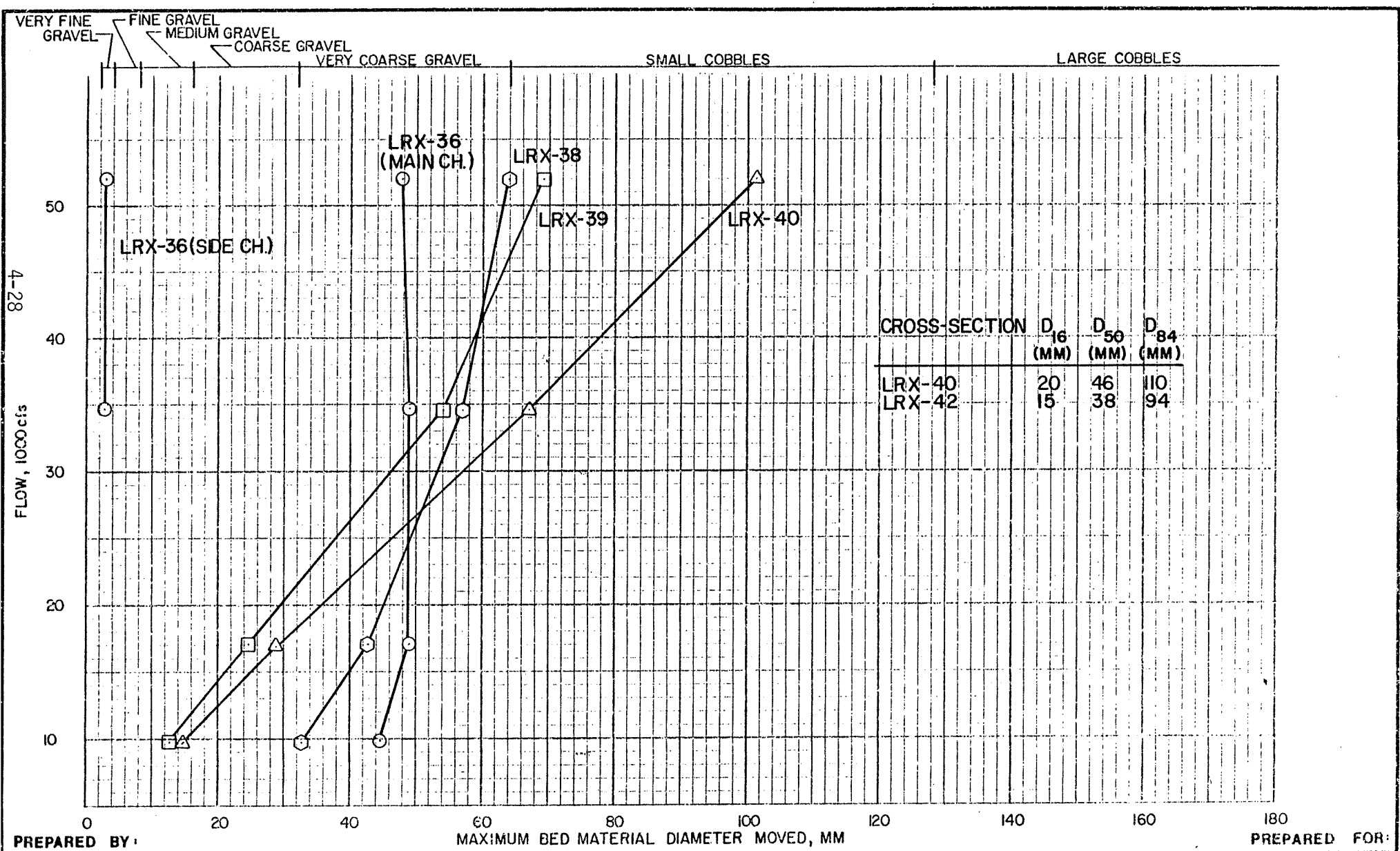
BED MATERIAL MOVEMENT CURVES LRX - 36, -38, -39, -40
