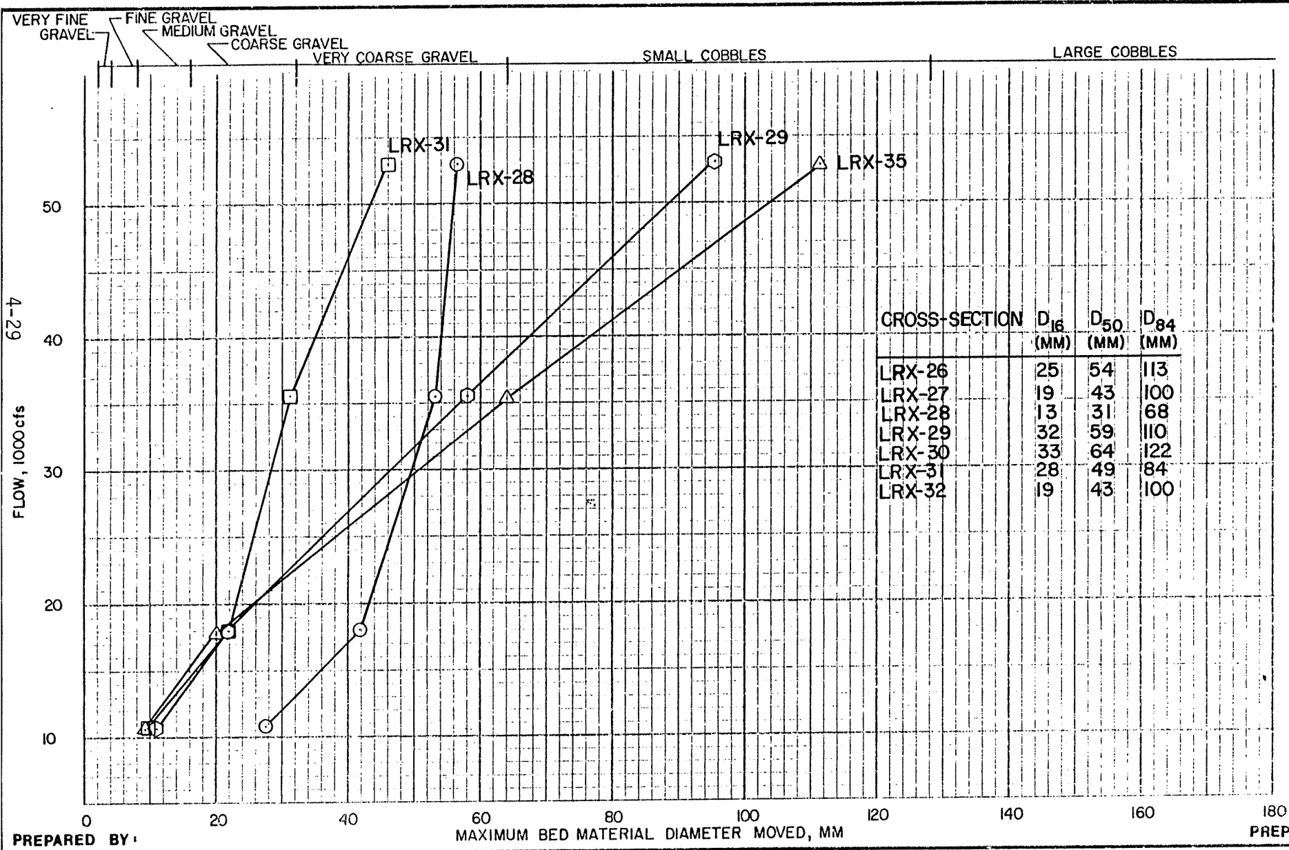
BED MATERIAL MOVEMENT CURVES LRX-28,-29,-31,-35
