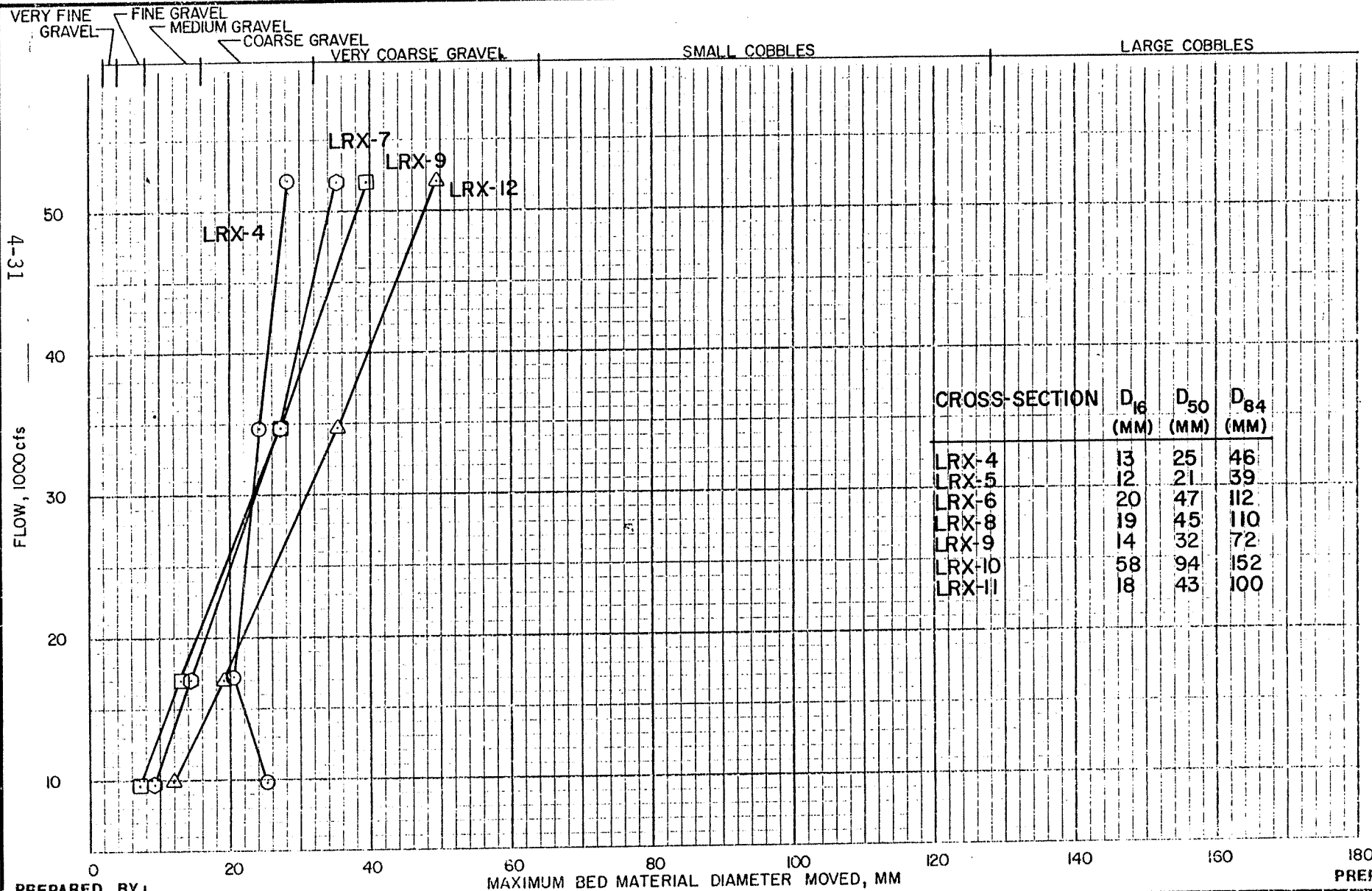
BED MATERIAL MOVEMENT CURVES LRX -4, -7, -9, -12
