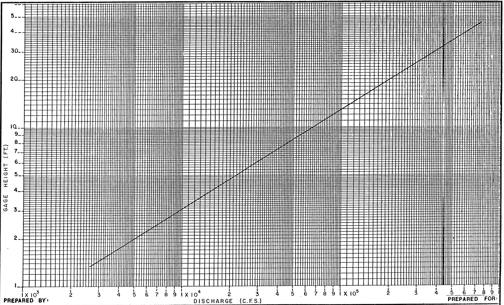
RATING CURVE FOR SUSITNA RIVER AT SUNSHINE
