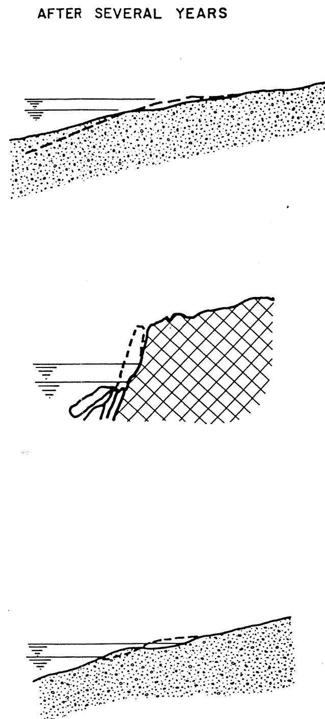
SLOPE MODELS FOR THE WATANA AND DEVIL CANYON RESERVOIRS
