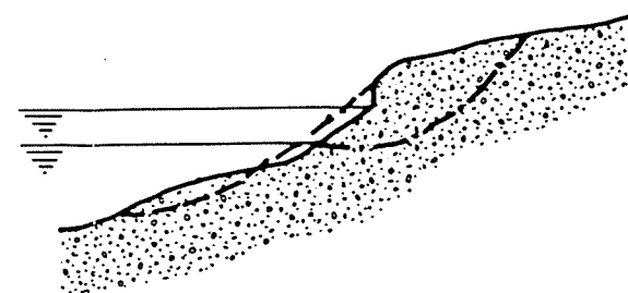
SLOPE MODELS FOR THE WATANA AND DEVIL CANYON RESERVOIRS
