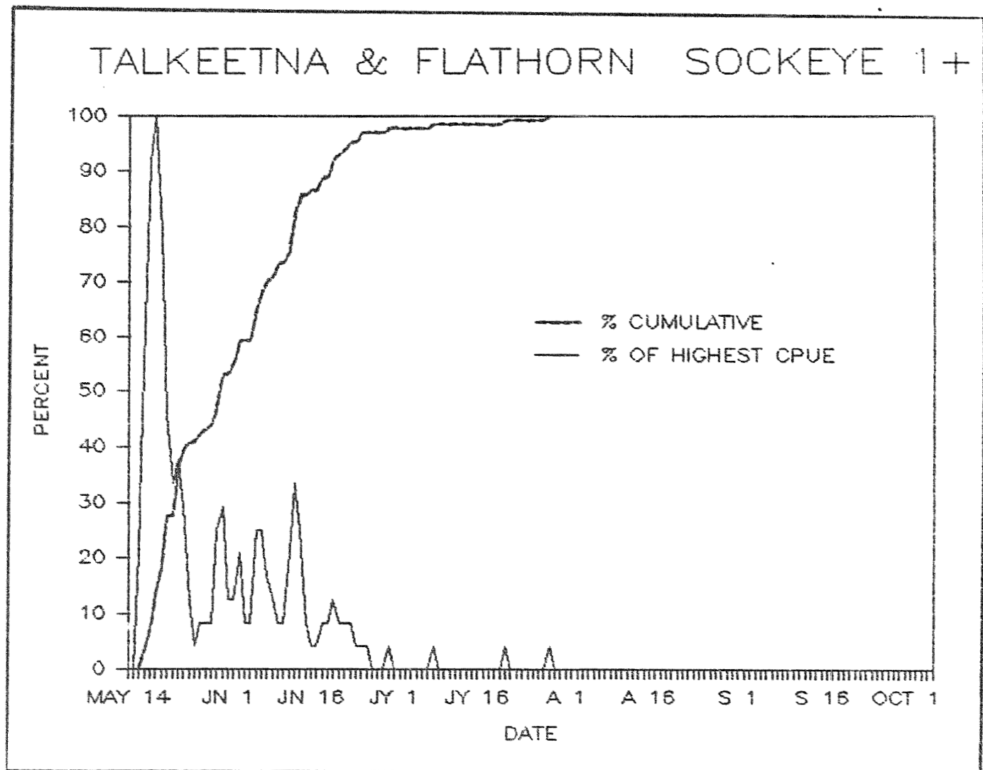
Figure 30. Sockeye salmon (age 1+) smoothed daily catch per unit effort and adjusted cumulative catch recorded at the Flathorn and Talkeetna stationary outmigrant traps, May 14 through October 6, 1984.
