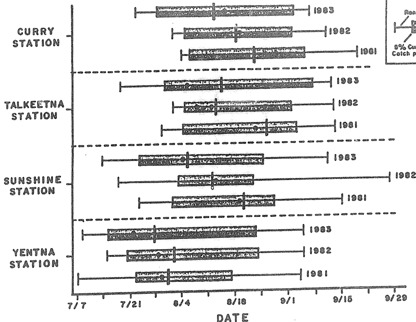
MIGRATIONAL TIMING OF COHO SALMON BASED ON FISHWHEEL CATCH PER UNIT EFFORT AT SELECTED LOCATIONS ON THE SUSITNA RIVER IN 1981, 1982 AND 1983. (SOURCE: ADF6G-1984a).
