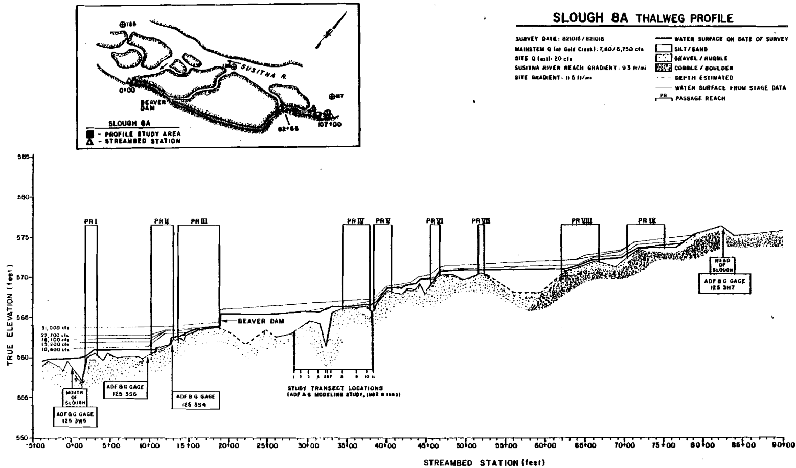
Figure 6-E-3. Thalweg profile of Slough 8A.
