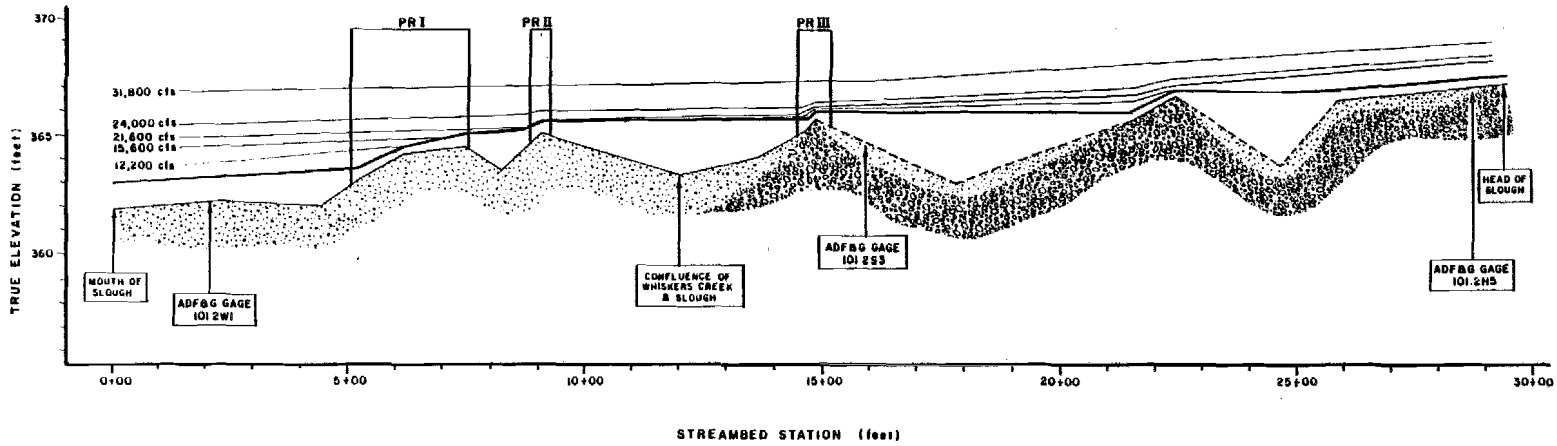
Figure 6-E-1. Thalweg profile of Whiskers Creek Slough.
