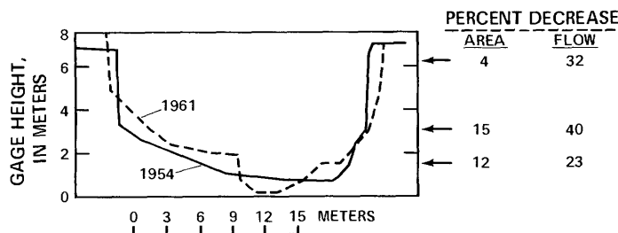
FIGURE 23.—Changes in channel cross section of Sandstone Creek, Oklahoma, at the streamflow-gaging station, 1954-61, caused by many upstream flood-detention dams (modified from Bergman and Sullivan, 1963).
