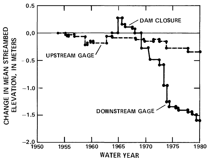
FIGURE 42.—Changes in mean streambed elevation with time at streamflow-gaging station on Republican River 2.7 kilometers downstream from Milford Dam, Kansas, and at control station at Clay Center 49 kilometers upstream from dam. Plotted points represent elevation corresponding to a discharge of 1.2 cubic meters per second downstream from dam and 3.4 cubic meters per second upstream from dam, as determined from rating tables.
