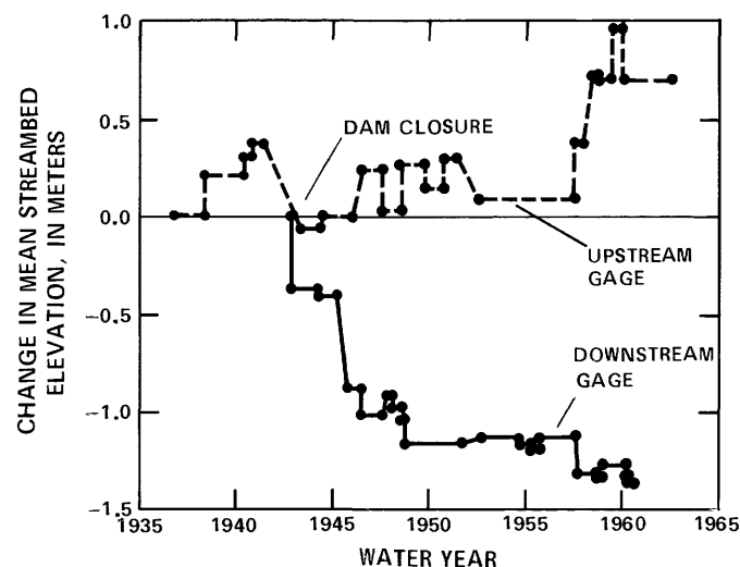
FIGURE 44.—Changes in mean streambed elevation with time at streamflow-gaging station on Red River 4.5 kilometers downstream from Denison Dam, Oklahoma, and at the control station near Gainesville, Texas, 106 kilometers upstream from dam. Plotted points represent elevation corresponding to a discharge of 3.7 cubic meters per second downstream from dam and 4.2 cubic meters per second upstream from dam, as determined from rating tables.
