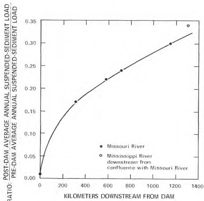
FIGURE 4.—Post-dam/pre-dam ratio of annual suspended-sediment loads versus distance downstream from Gavins Point Dam, Missouri River, South Dakota.
