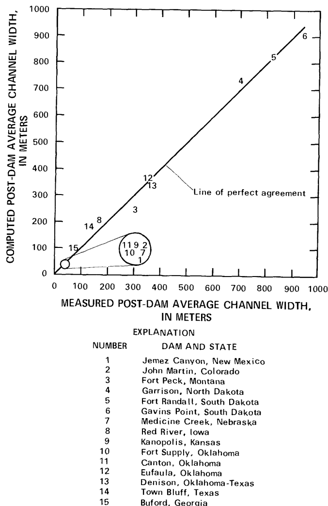
FIGURE 29.—Computed (by the equation W_2 = 13 + 0.5Q_m + 0.1Q_p ) versus measured values of post-dam average channel widths.
