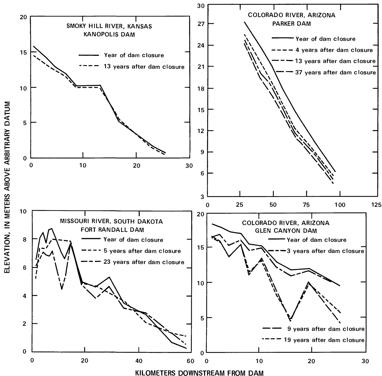
FIGURE 12.—Longitudinal-profile changes downstream from four dams.
