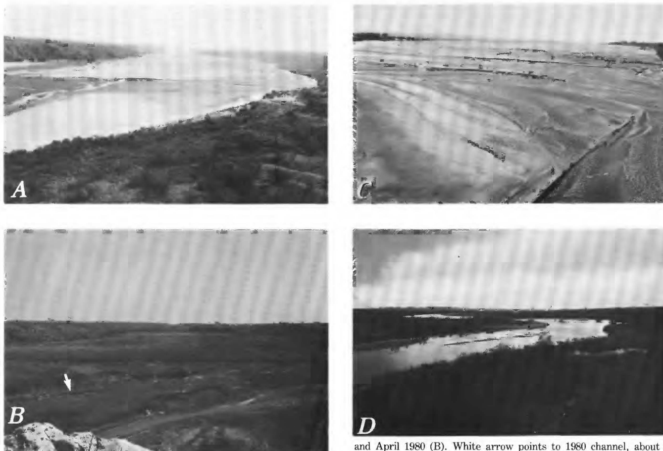
FIGURE 33.—Canadian River downstream from Sanford Dam, Texas. Dam was closed in 1964. Looking downstream from about 400 meters downstream from damsite, October 1960 (A, prior to dam)
