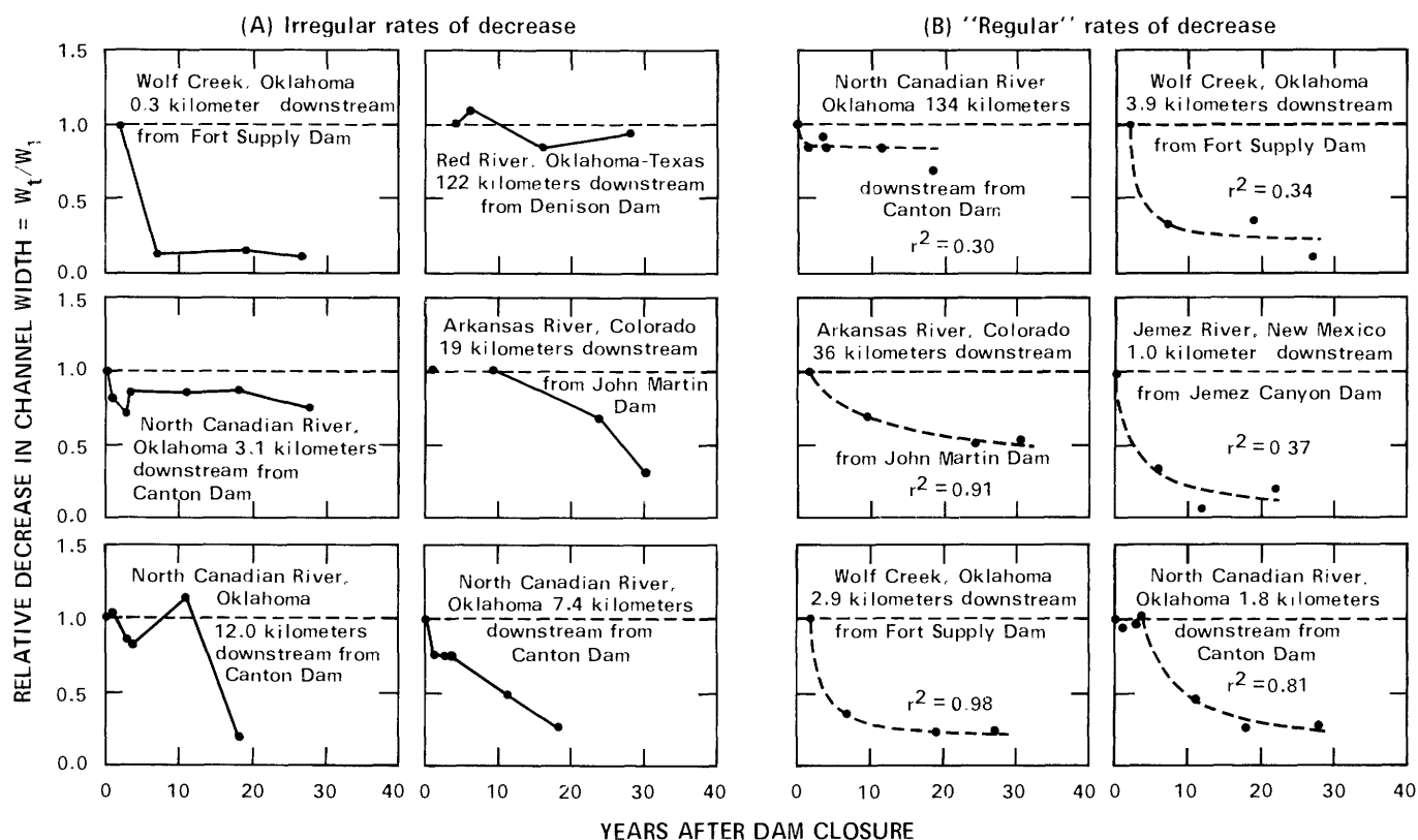
FIGURE 27.—Examples of relative decrease in channel width with time: A, irregular rates; B, regular rates with fitted regression curves (dashed lines). Data from table 13.
