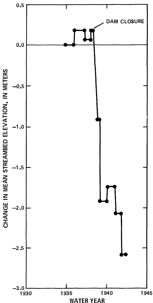
FIGURE 36.—Changes in mean streambed elevation with time at streamflow-gaging station on Colorado River 6.4 kilometers downstream from Parker Dam, Arizona. Plotted points represent elevation corresponding to a discharge of 90.6 cubic meters per second, as determined from rating tables. No upstream control station available.
