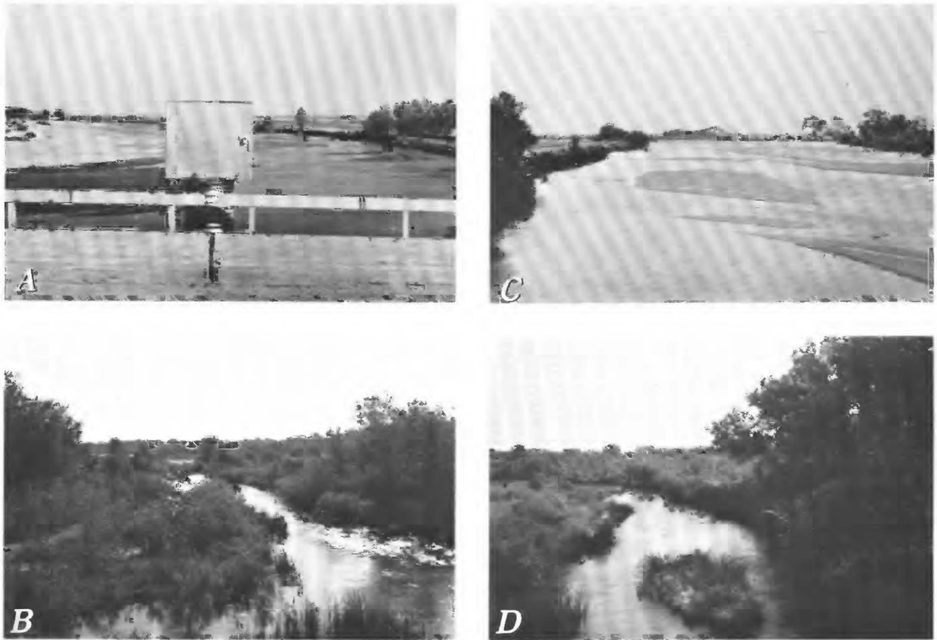
FIGURE 31.—Republican River downstream from Trenton Dam, Nebraska. Dam was closed in 1953. Looking downstream from bridge at Trenton (4 kilometers downstream from the dam), about 1949 (A) and July 1980 (B). Looking downstream from bridge at Culbertson (19 kilometers downstream from dam), July 1932 (C) and July 1980 (D).
