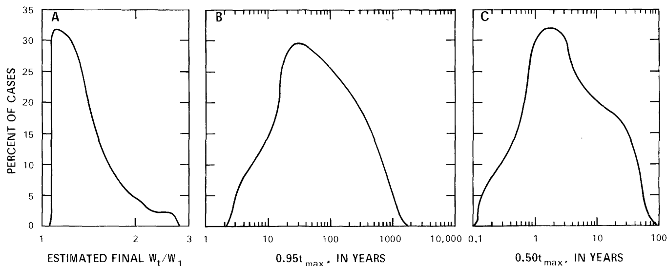
FIGURE 25.—Frequency distributions of estimated eventual increases in channel width, based on 44 measured cross sections on various rivers: A, final values of W_t/W_1 ; B, years needed to widen to 95 percent of final W_t/W_1 ; C, years needed to widen to 50 percent of final W_t/W_1 .
