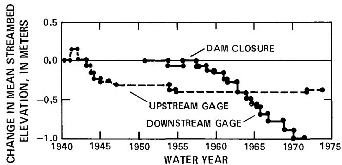
FIGURE 46.—Changes in mean streambed elevation with time at streamflow-gaging station on Chattahoochee River 4 kilometers downstream from Buford Dam, Georgia, and at the control station on the Chestatee River near Dahlonega 73 kilometers upstream from dam. Plotted points represent elevation corresponding to a discharge of 12.2 cubic meters per second downstream from dam and 3.4 cubic meters per second upstream from dam, as determined from rating tables.
