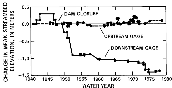
FIGURE 41.—Changes in mean streambed elevation with time at streamflow-gaging station on Smoky Hill River 1.3 kilometers downstream from Kanopolis Dam, Kansas, and at the control station at Ellsworth 48 kilometers upstream from dam. Plotted points represent elevation corresponding to a discharge of 0.51 cubic meter per second downstream from dam and 0.43 cubic meter per second upstream from dam, as determined from rating tables.
