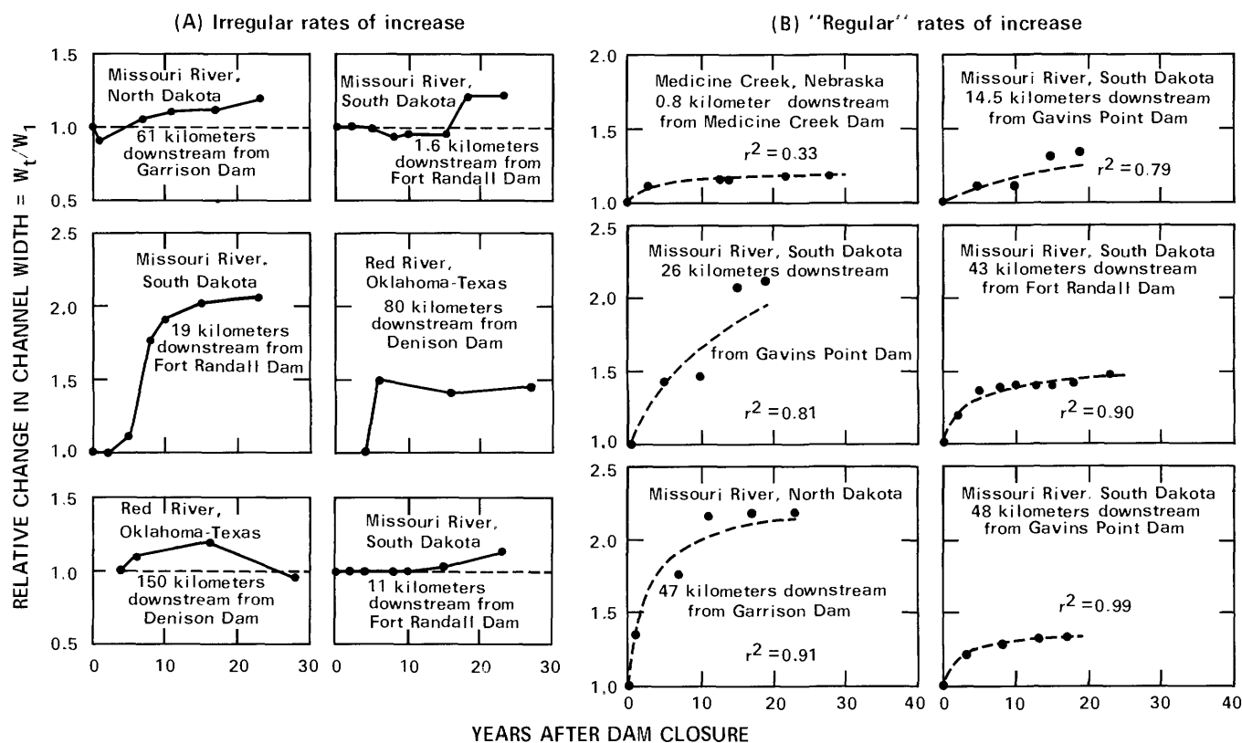
FIGURE 24.—Examples of relative increase of channel width with time: A, irregular rates; B, regular rates with fitted regression curves (dashed lines). Data from table 13.
