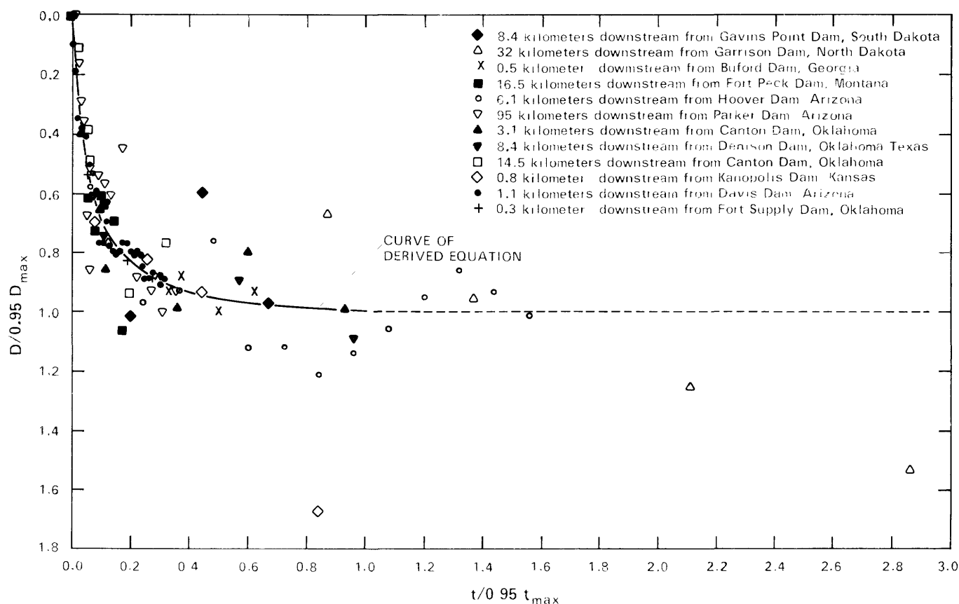
FIGURE 11.—Standardized degradation-time dimensionless plot of degradation curves in figure 9.
