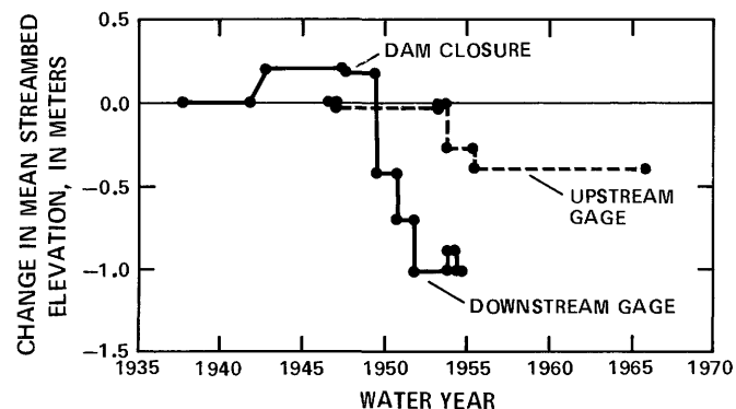
FIGURE 43.—Changes in mean streambed elevation with time at streamflow-gaging station on North Canadian River 4.8 kilometers downstream from Canton Dam, Oklahoma, and at the control station near Seiling 45 kilometers upstream from dam. Plotted points represent elevation corresponding to a discharge of 0.031 cubic meter per second downstream from dam and 0.00057 cubic meter per second upstream from dam, as determined from rating tables.
