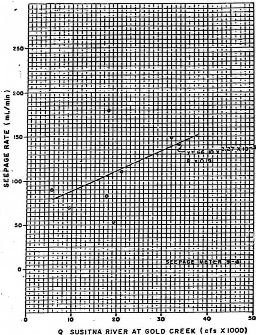
EXHIBIT 25. SEEPAGE RATE VS. MAINSTEM DISCHARGE, SEEPAGE METER 9-3.
