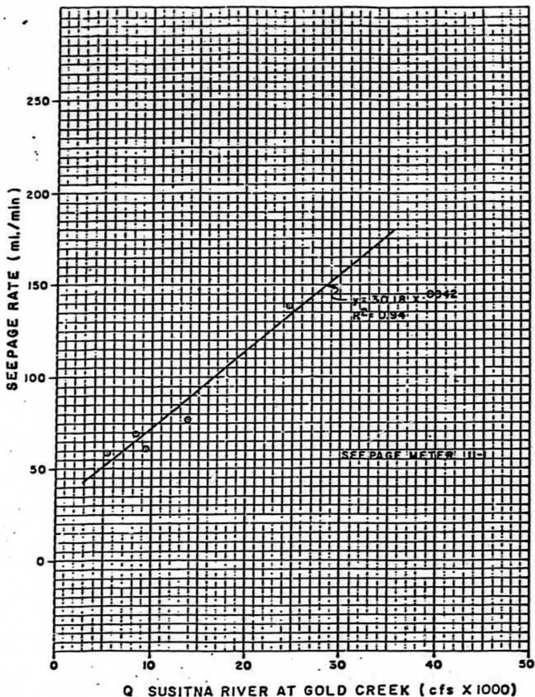
EXHIBIT 26. SEEPAGE RATE VS. MAINSTEM DISCHARGE, SEEPAGE METER 11-1.
