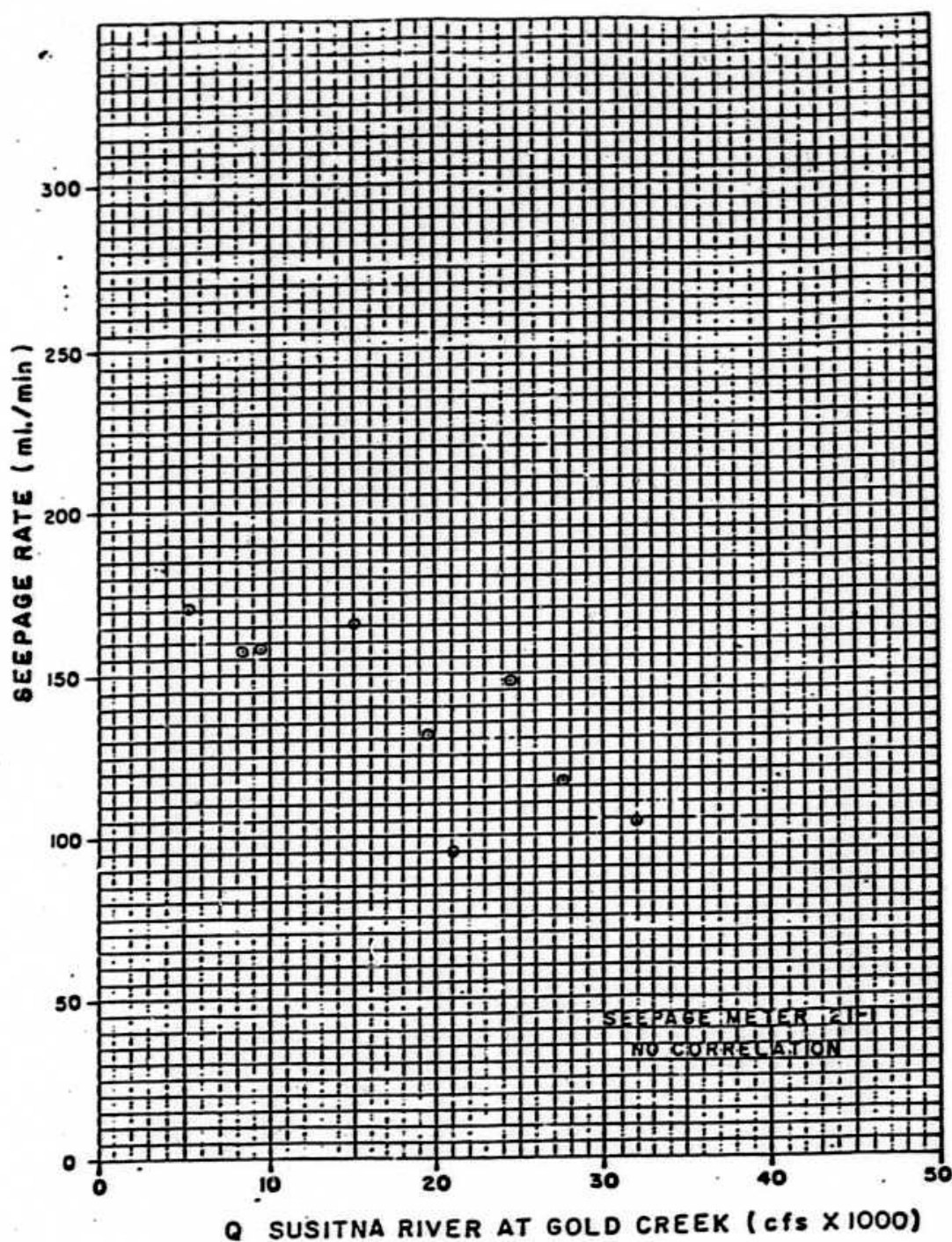
EXHIBIT 28. SEEPAGE RATE VS. MAINSTEM DISCHARGE, SEEPAGE METER 21-1.
