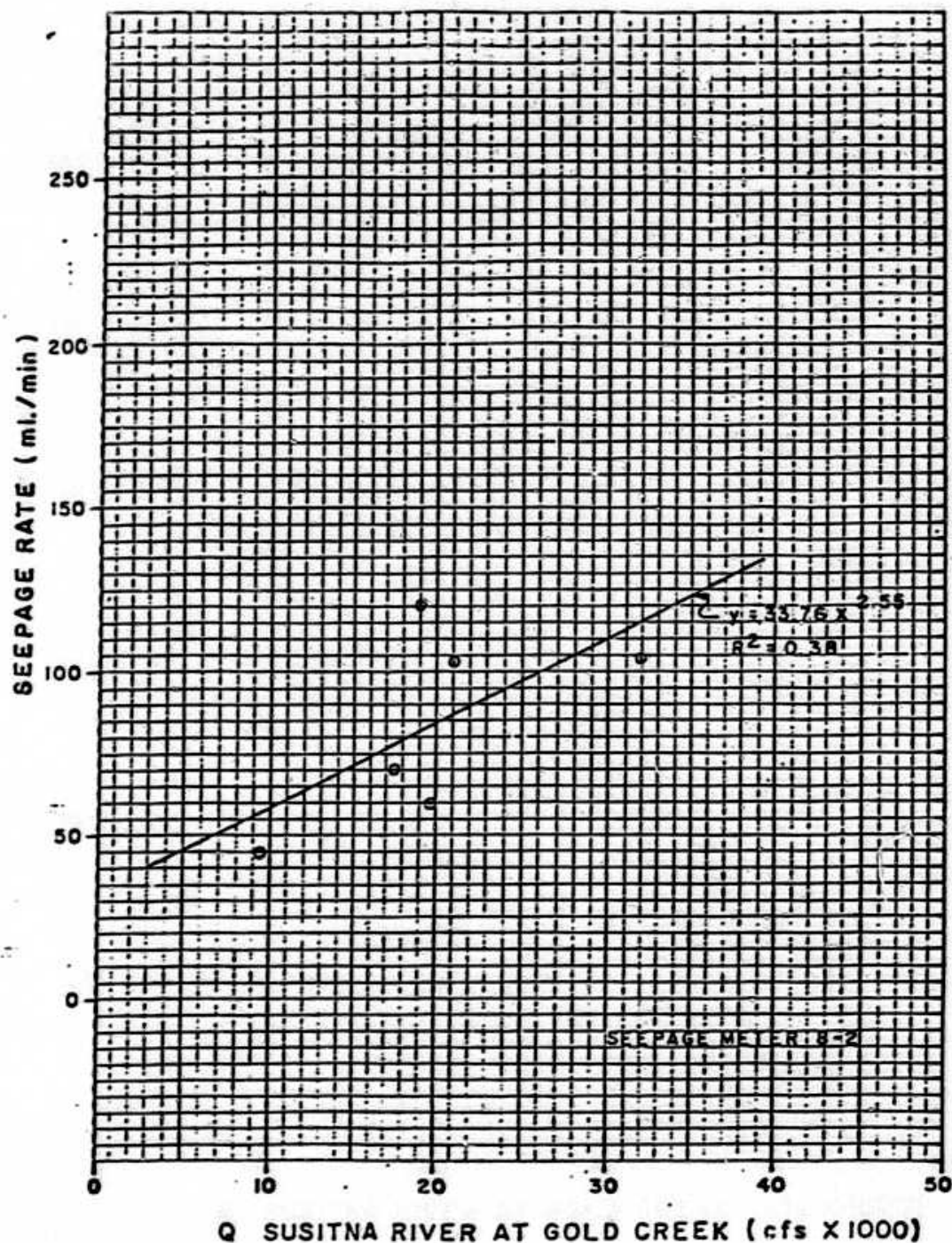
EXHIBIT 22. SEEPAGE RATE VS. MAINSTEM DISCHARGE, SEEPAGE METER 8-2.
