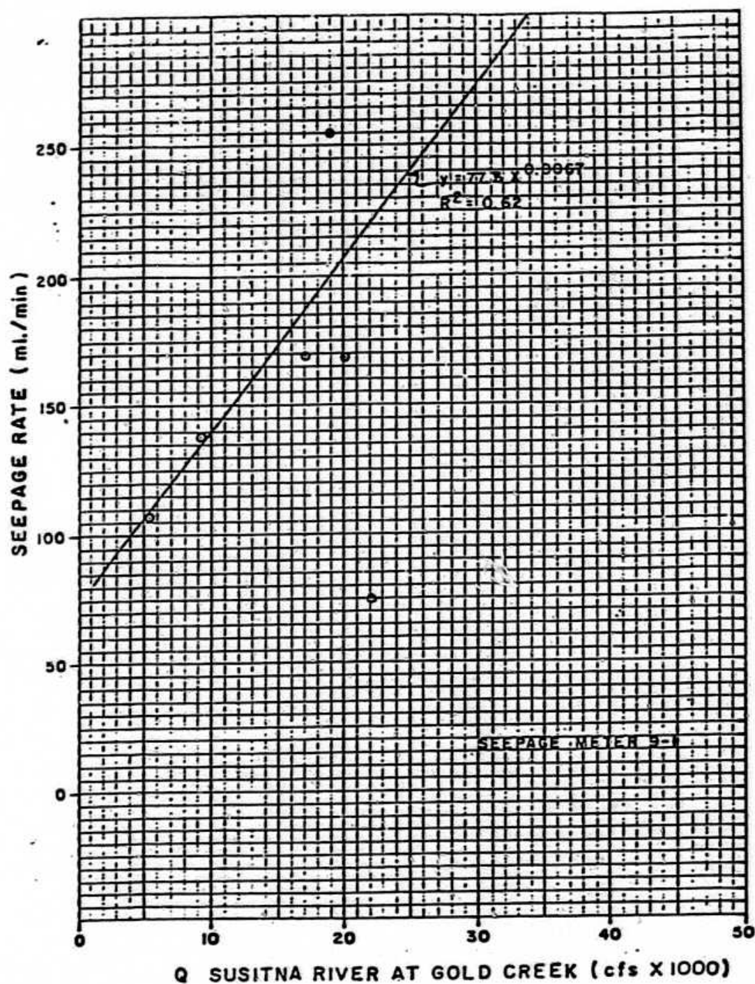
EXHIBIT 23. SEEPAGE RATE VS. MAINSTEM DISCHARGE, SEEPAGE METER 9-1.
