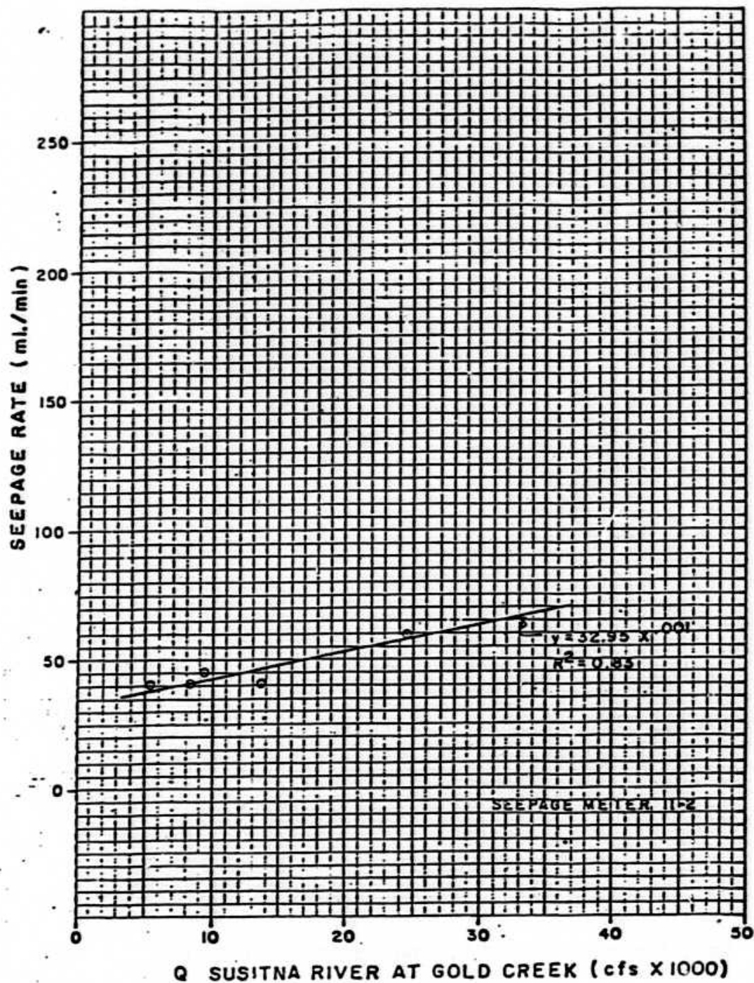
EXHIBIT 27. SEEPAGE RATE VS. MAINSTEM DISCHARGE, SEEPAGE METER 11-2.
