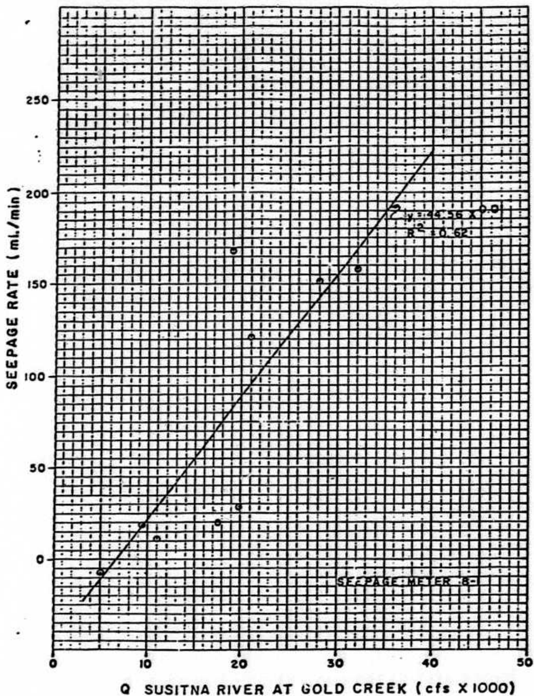
EXHIBIT 21. SEEPAGE RATE VS. MAINSTEM DISCHARGE, SEEPAGE METER 8-1.
