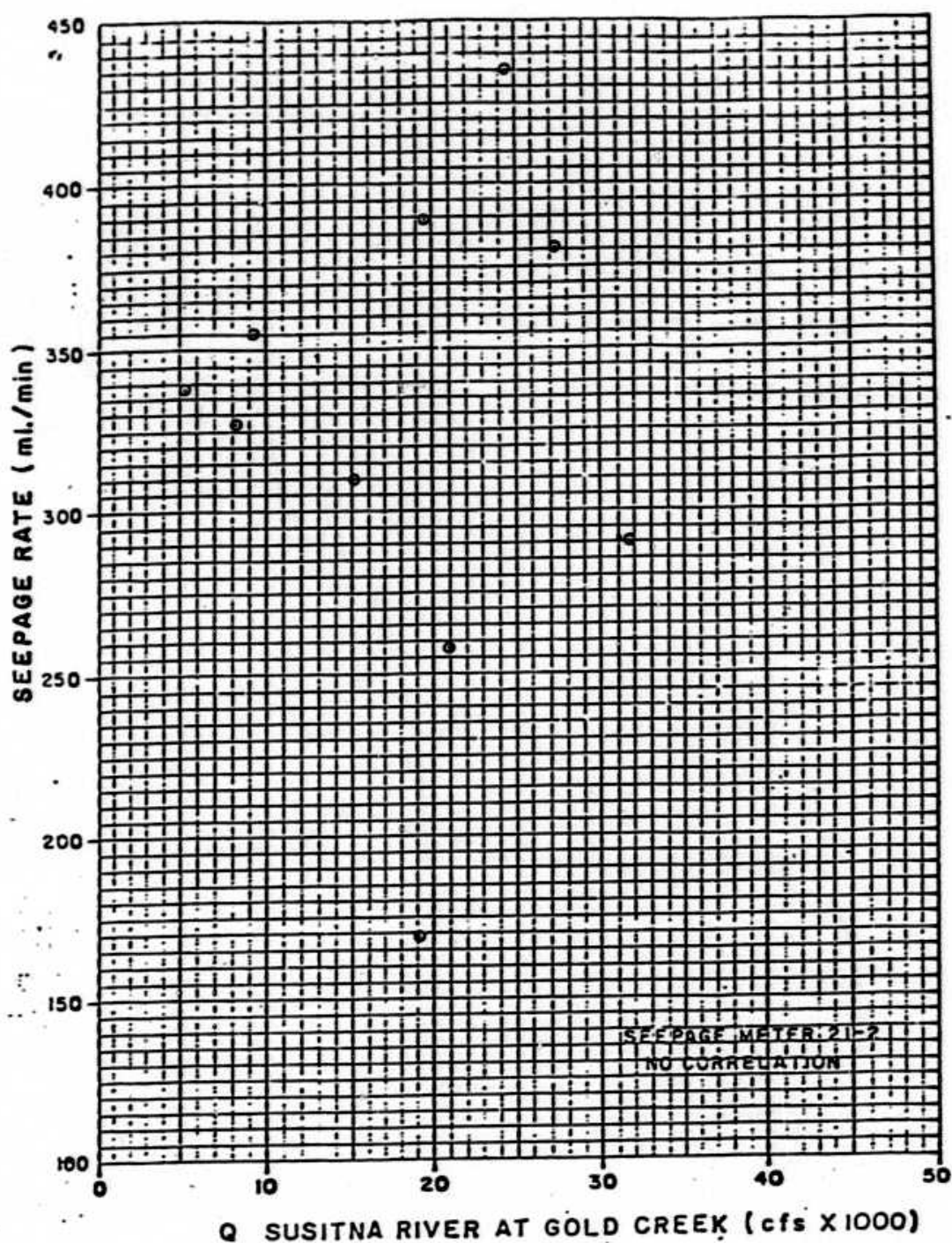
EXHIBIT 29. SEEPAGE RATE VS. MAINSTEM DISCHARGE, SEEPAGE METER 21-2.
