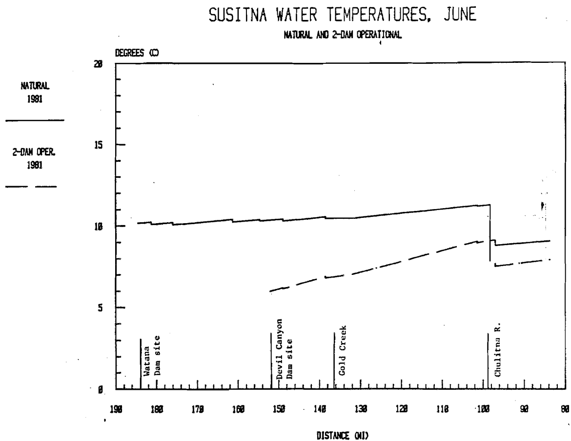
Figure 10. River temperature profiles for natural and 2-dam operational conditions.
