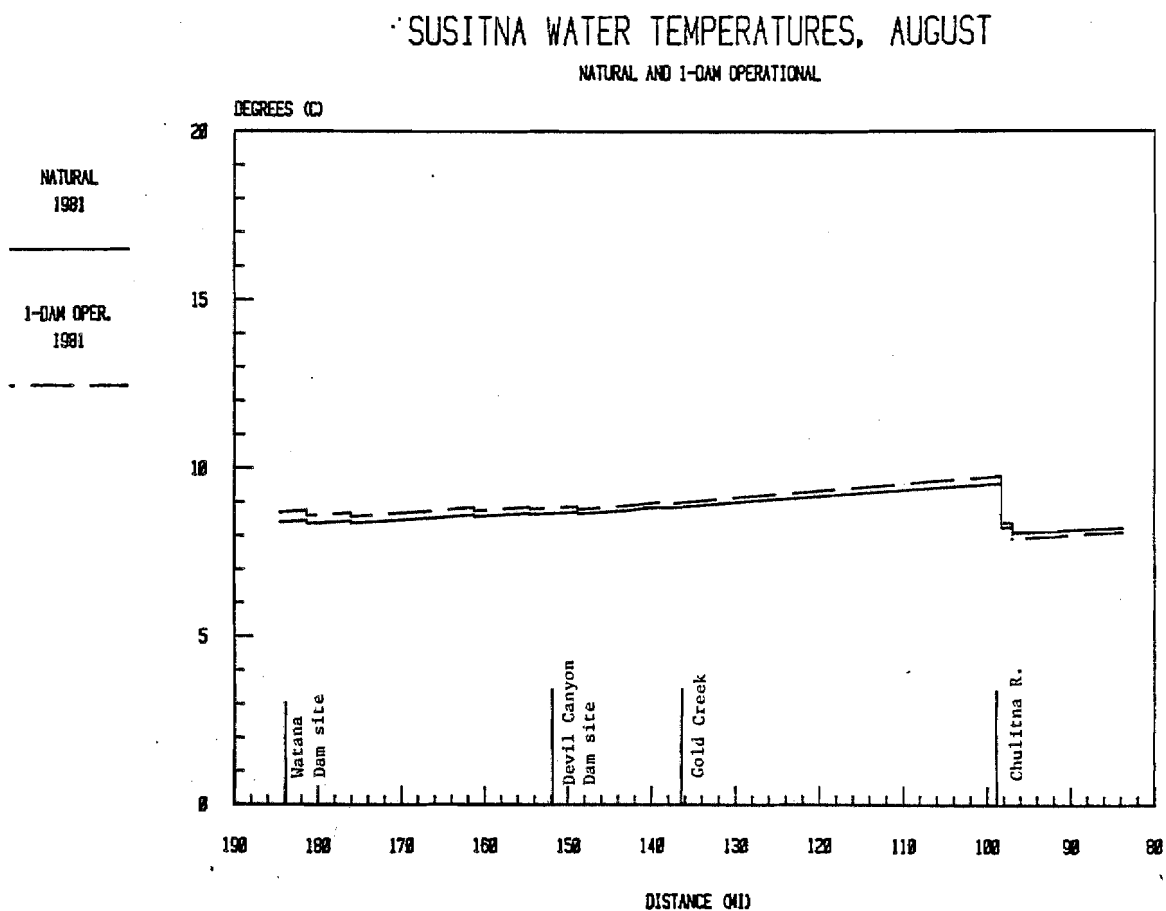
Figure 9 (Continued). River temperature profiles for natural and 1-dam operational conditions.
