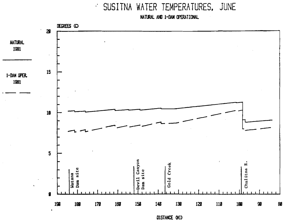
Figure 9. River temperature profiles for natural and 1-dam operational conditions.
