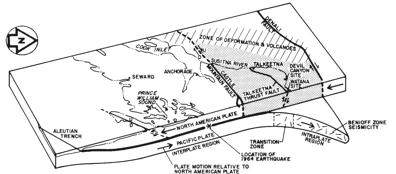
SCHEMATIC TALKEETNA TERRAIN SECTION
