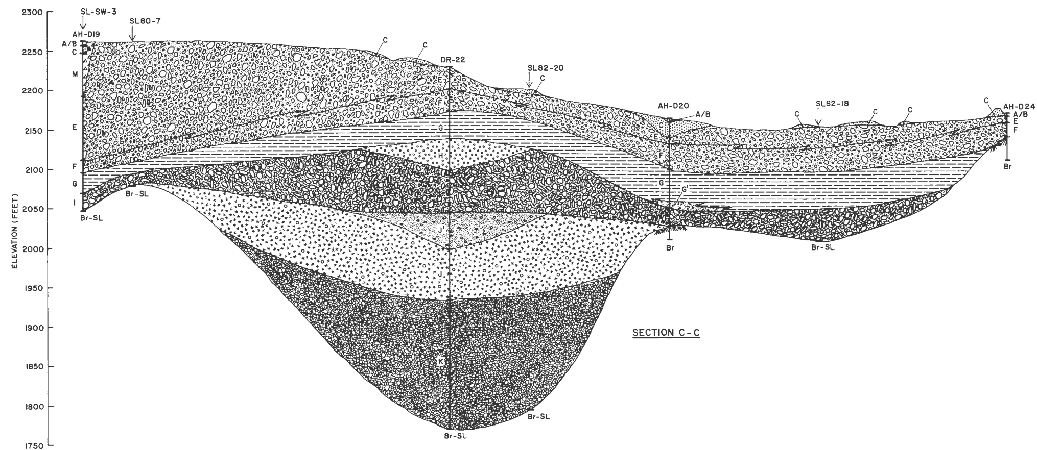
WATANA RELICT CHANNEL CROSS SECTIONS SHEET 1 OF 3
