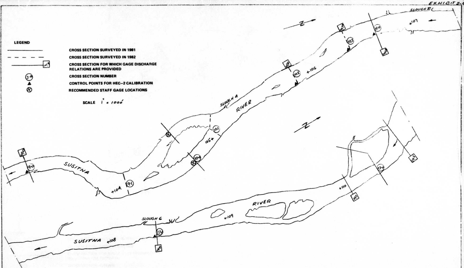
SUSITNA HYDROELECTRIC PROJECT LOCATIONS OF RIVER CROSS SECTIONS, STAFF GAGES AND SLOUGHS
