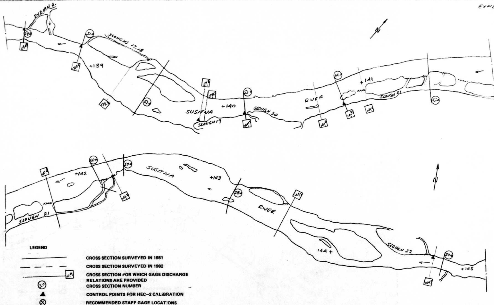
SUSITNA HYDROELECTRIC PROJECT LOCATIONS OF RIVER CROSS SECTIONS, STAFF GAGES AND SLOUGHS
