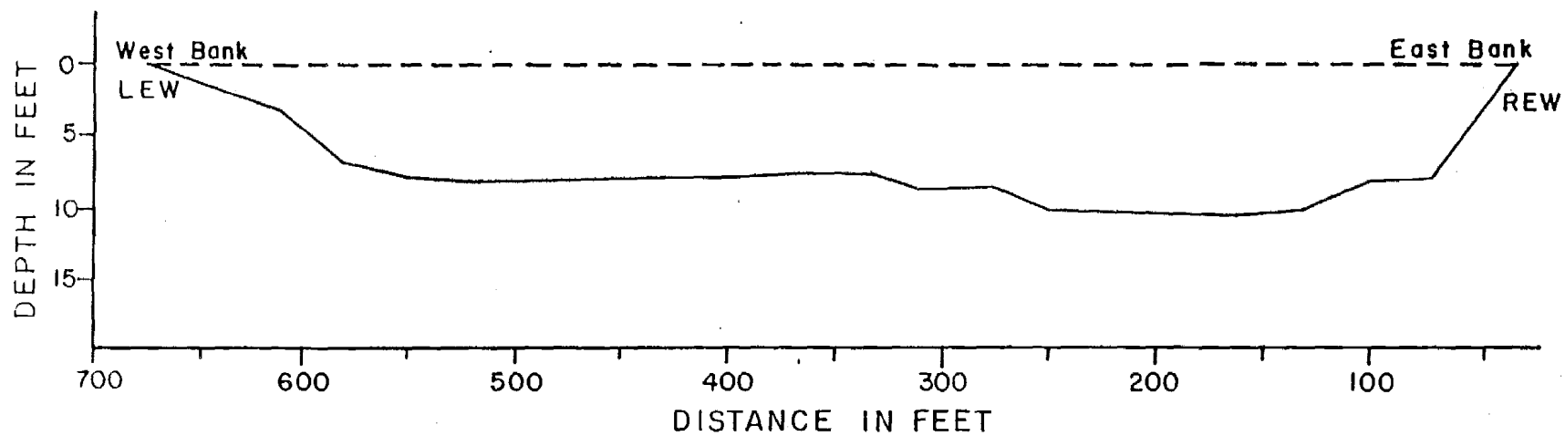
Appendix Figure 3-F-4. Bottom profile of Susitna River at RM 103.3. USGS preliminary data - 37,348 cfs discharge on June 22, 1982.
