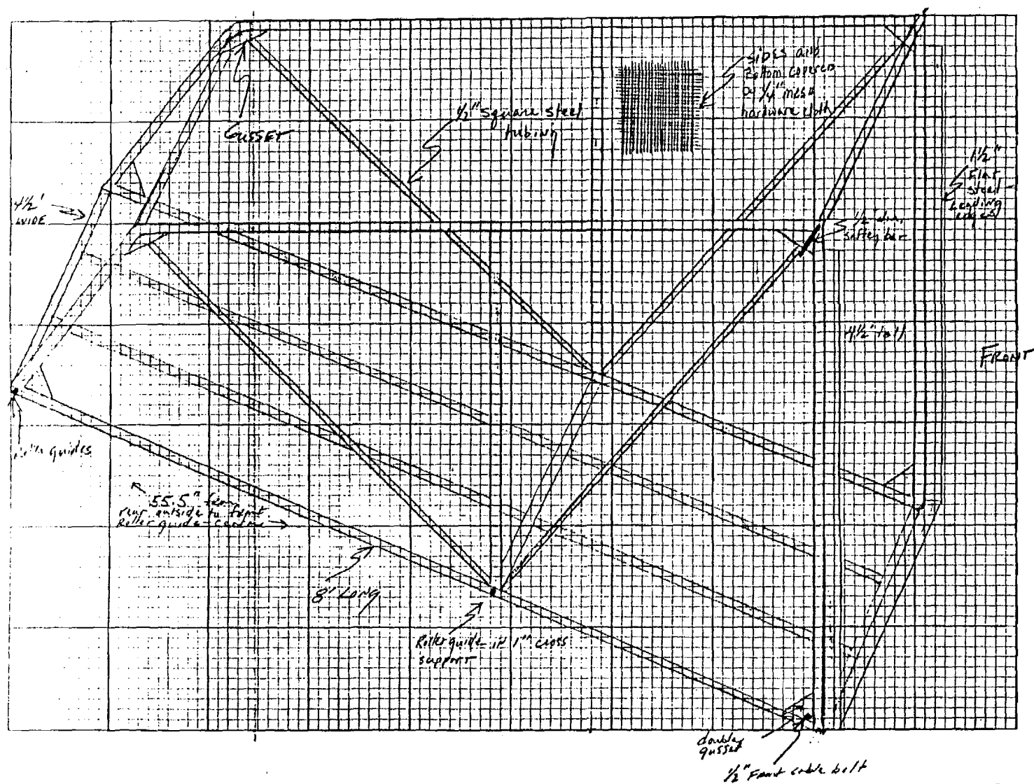
Appendix Figure 3-F-3. Side view of the incline plane on the downstream migrant trap, 1982.
