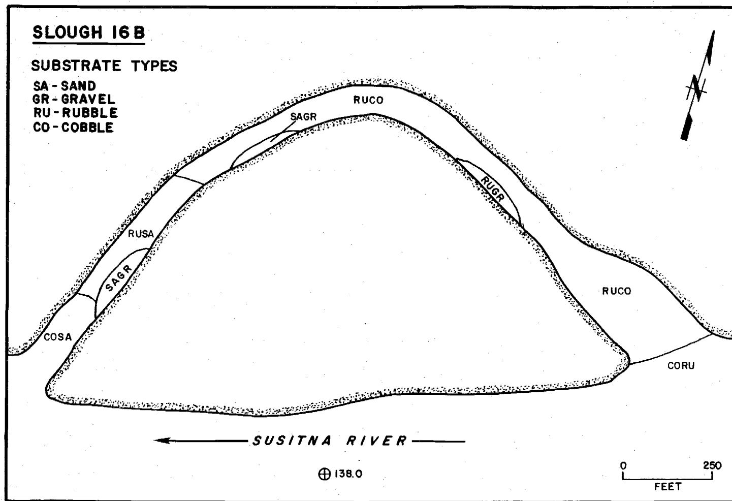
Figure 4-F-50. Slough 16B substrate, 1982.
