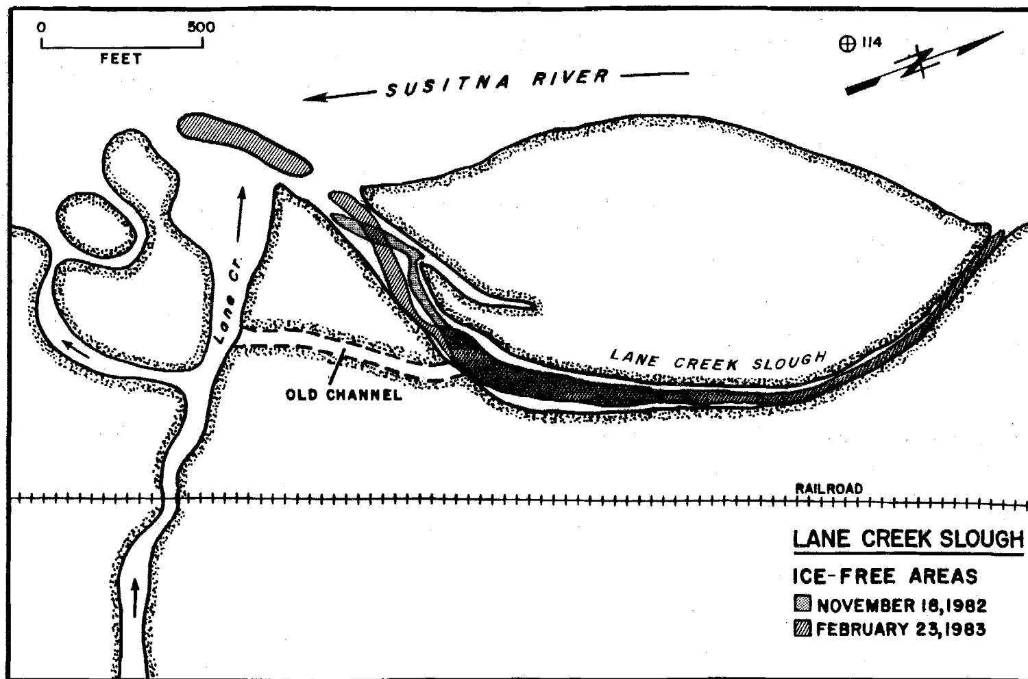
Figure 4-F-23. Lane Creek Slough ice-free areas, winter 1982-83.
