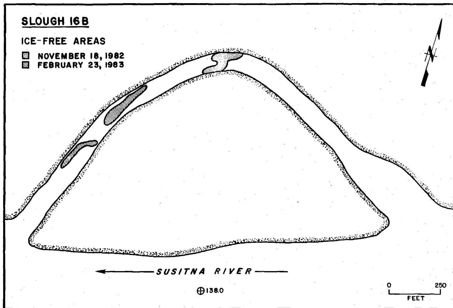
Figure 4-F-51. Slough 16B ice-free areas, winter 1982-83.
