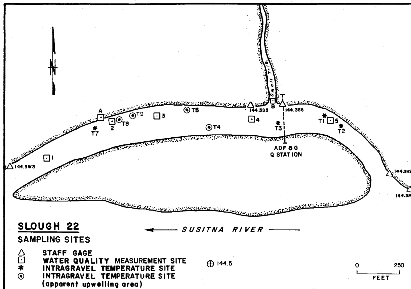
Figure 4-F-66. Slough 22 sampling sites, 1982.
