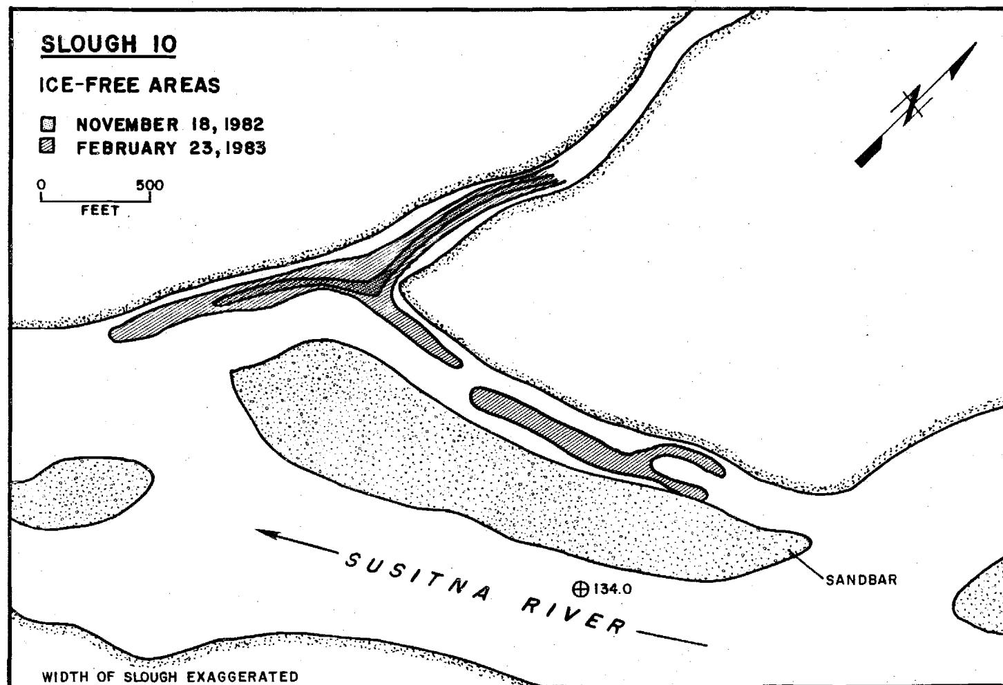
Figure 4-F-42. Slough 10 ice-free areas, winter 1982-83.
