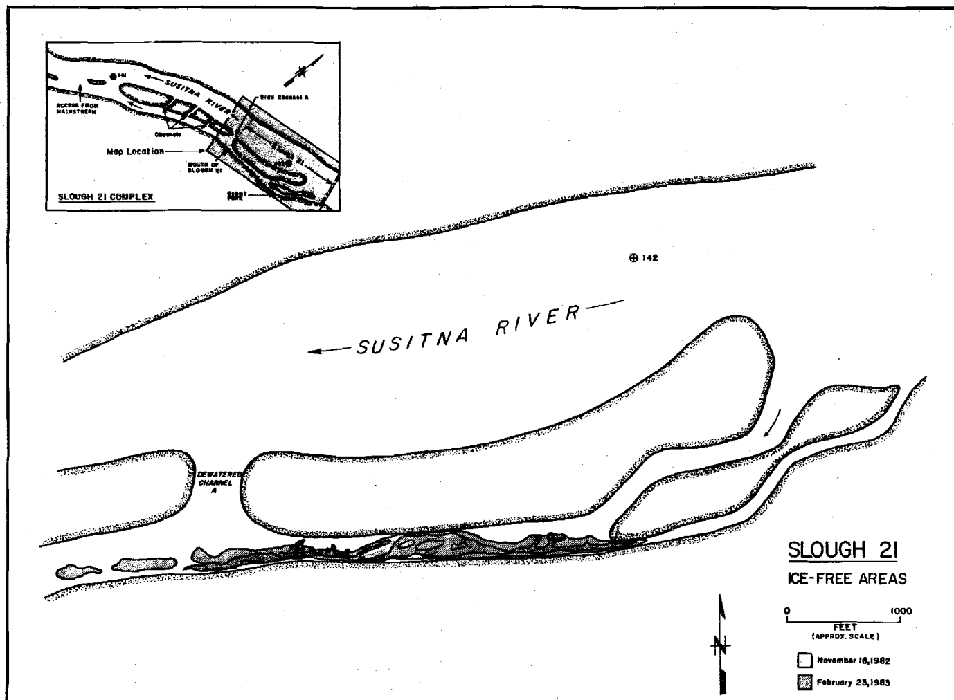
Figure 4-F-62. Slough 21 ice-free areas, winter 1982-83.
