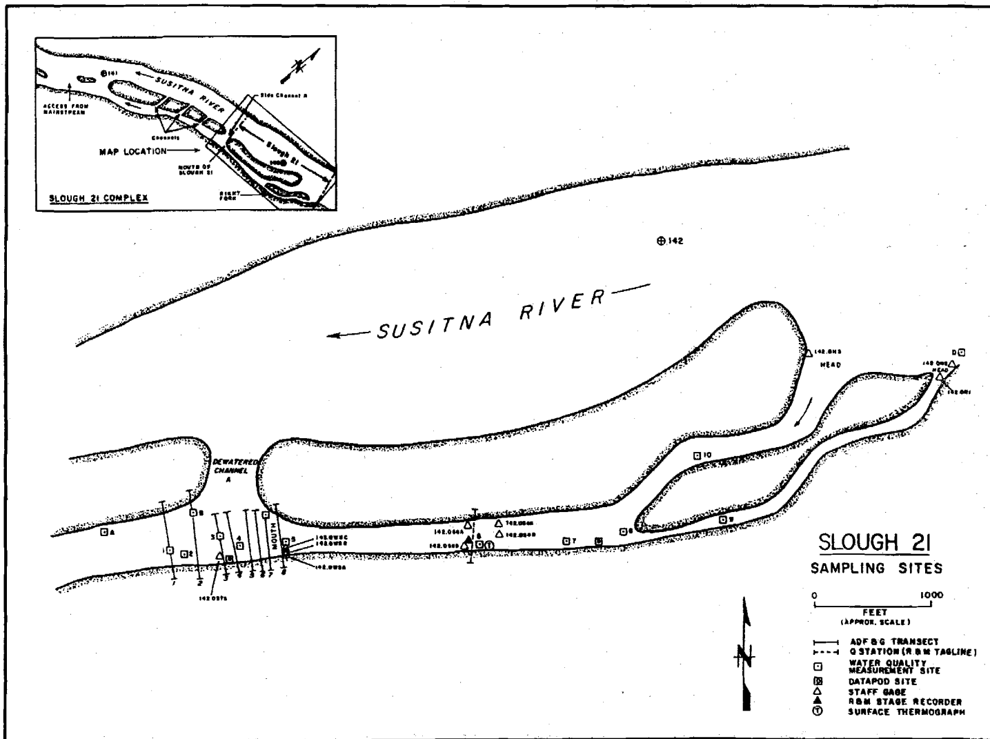
Figure 4-F-59. Slough 21 sampling sites, 1982.
