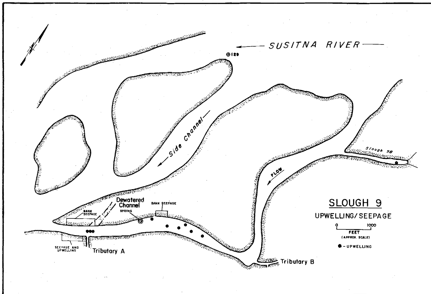
Figure 4-F-32. Slough 9 upwelling/seepage, 1982.
