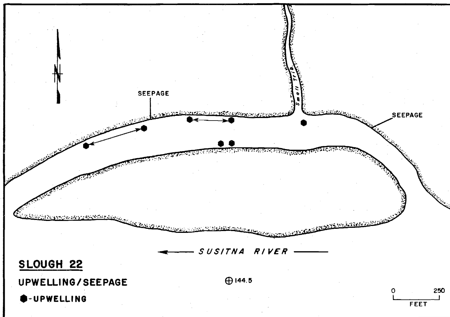
Figure 4-F-68. Slough 22 upwelling/seepage, 1982.
