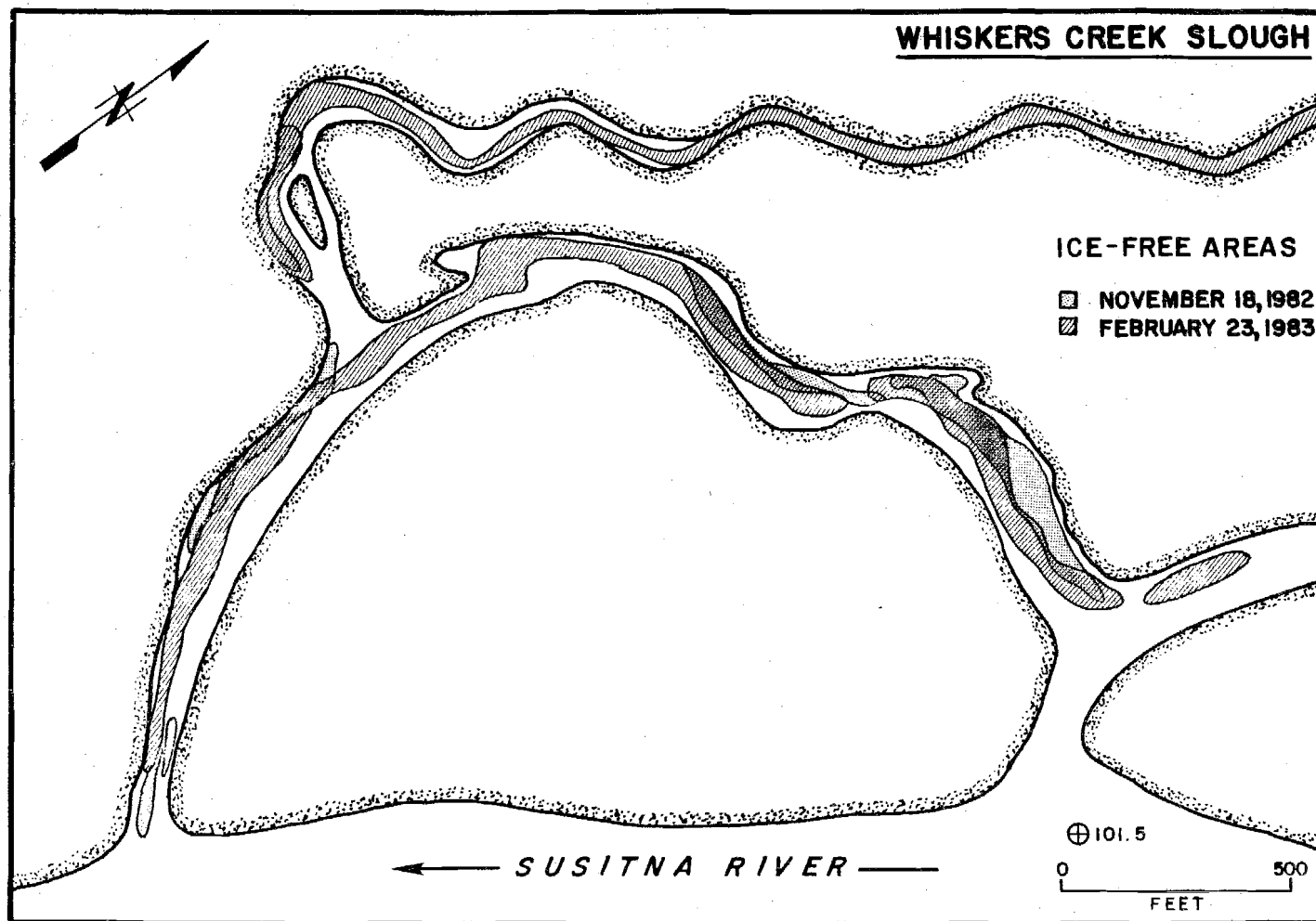
Figure 4-F-16. Whiskers Creek Slough ice-free areas, winter 1982-83.
