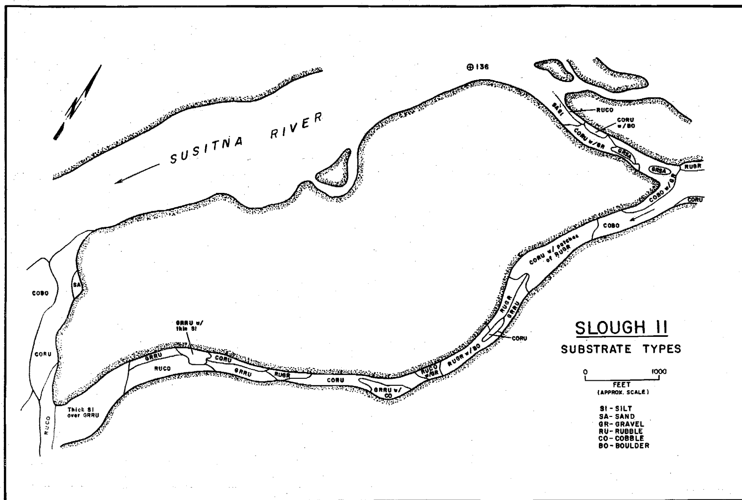
Figure 4-F-44. Slough 11 substrate, 1982.
