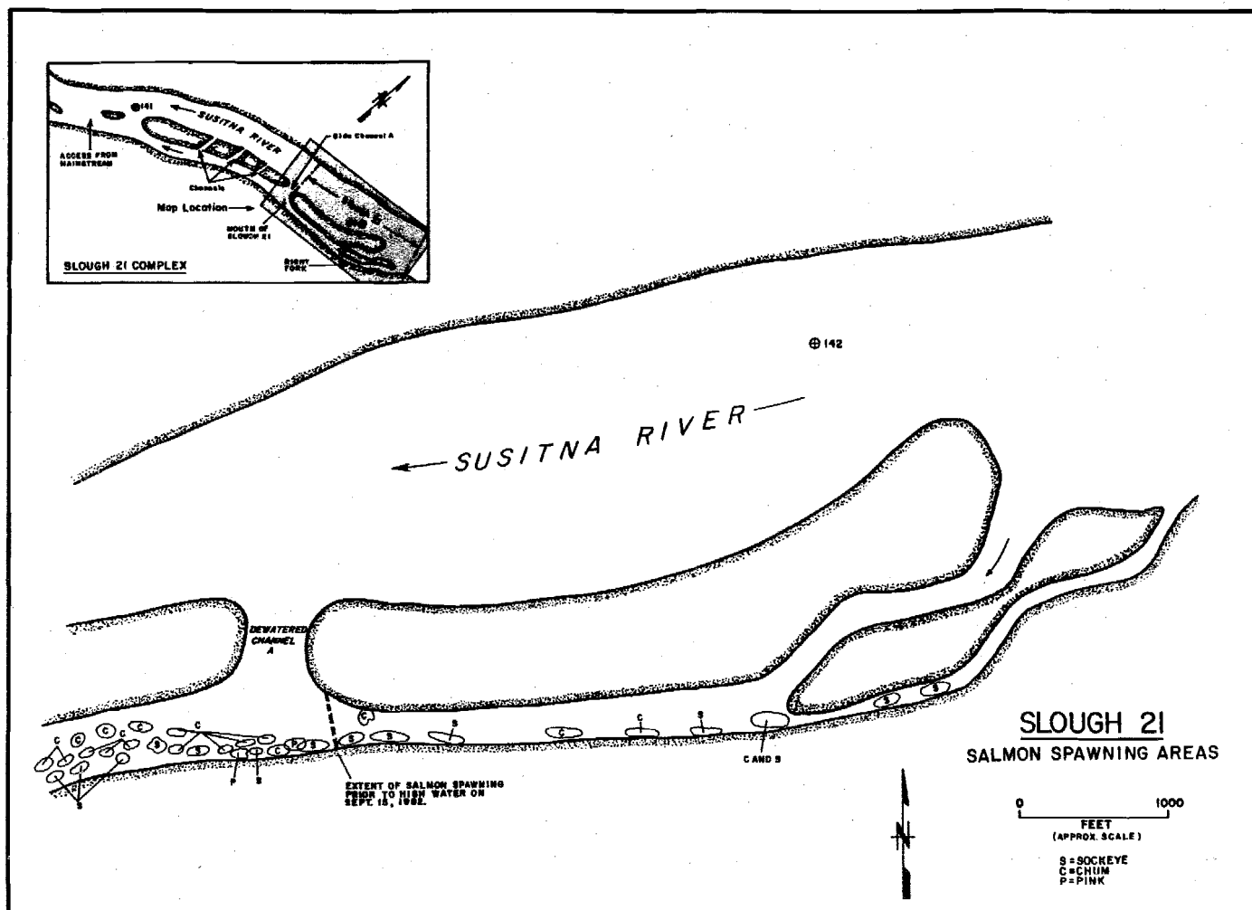
Figure 4-F-64. Slough 21 spawning areas, 1982.
