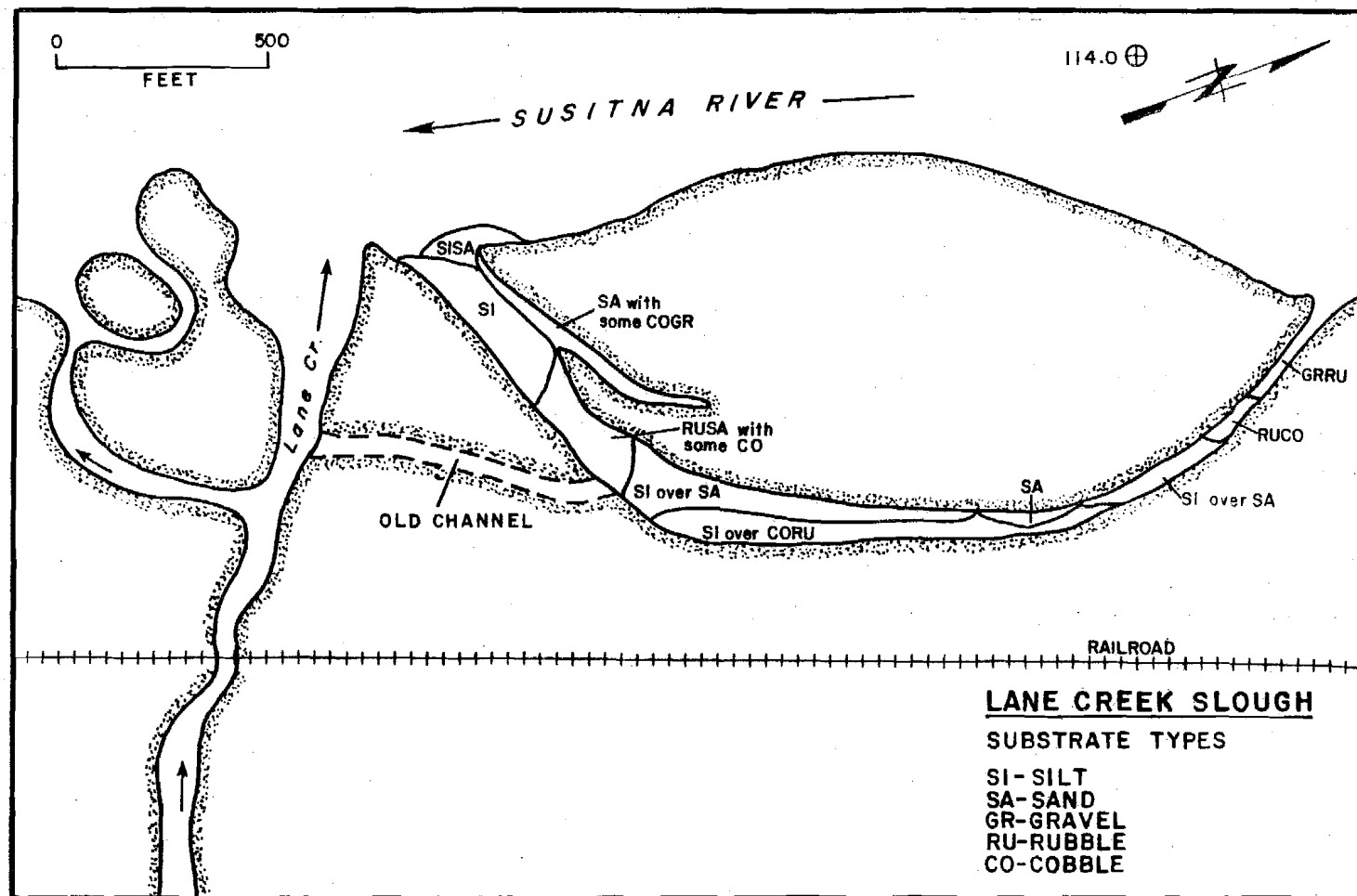
Figure 4-F-21. Lane Creek Slough substrate, 1982.
