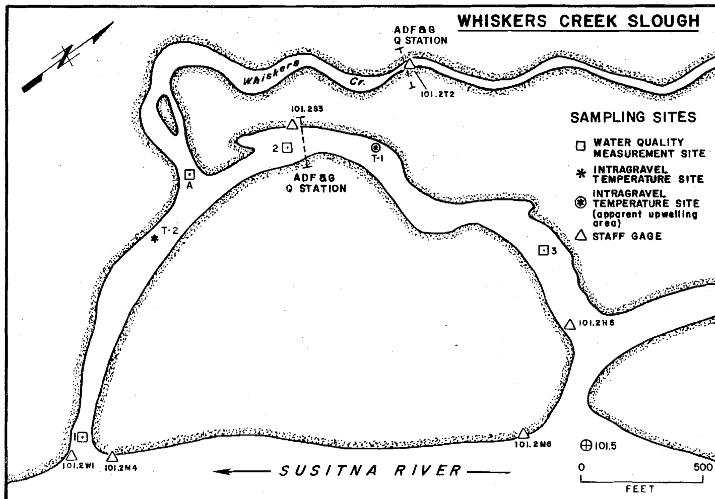
Figure 4-F-14. Whiskers Creek Slough sampling sites, 1982.
