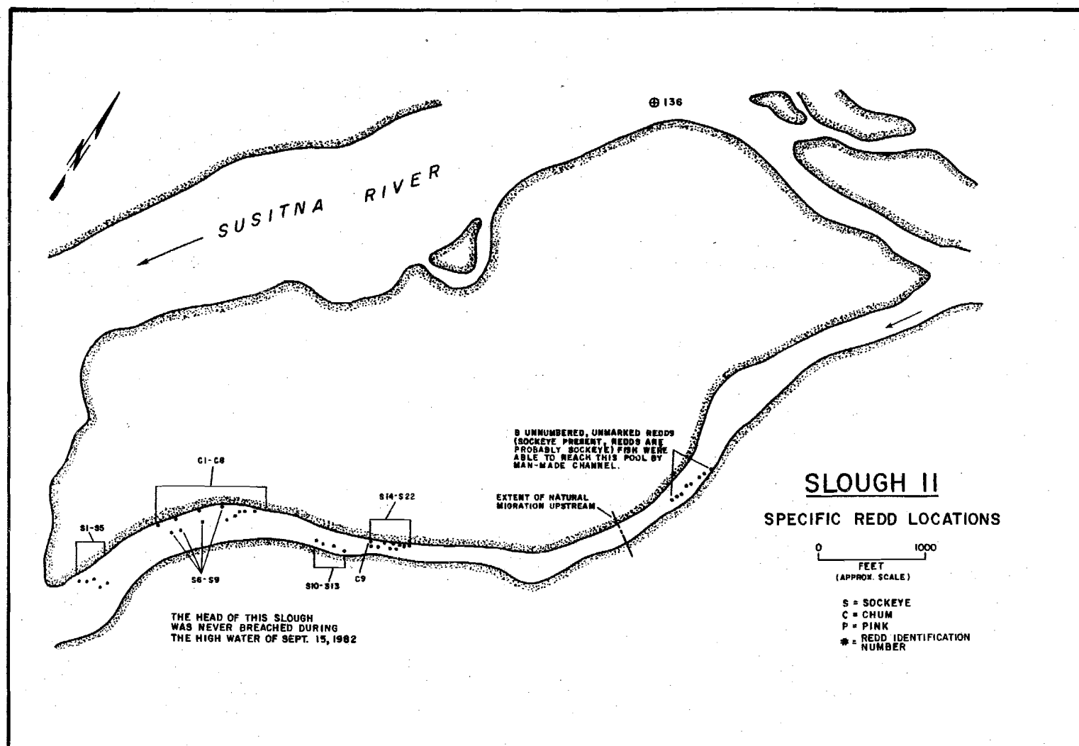
Figure 4-F-48. Slough II redd locations, 1982.
