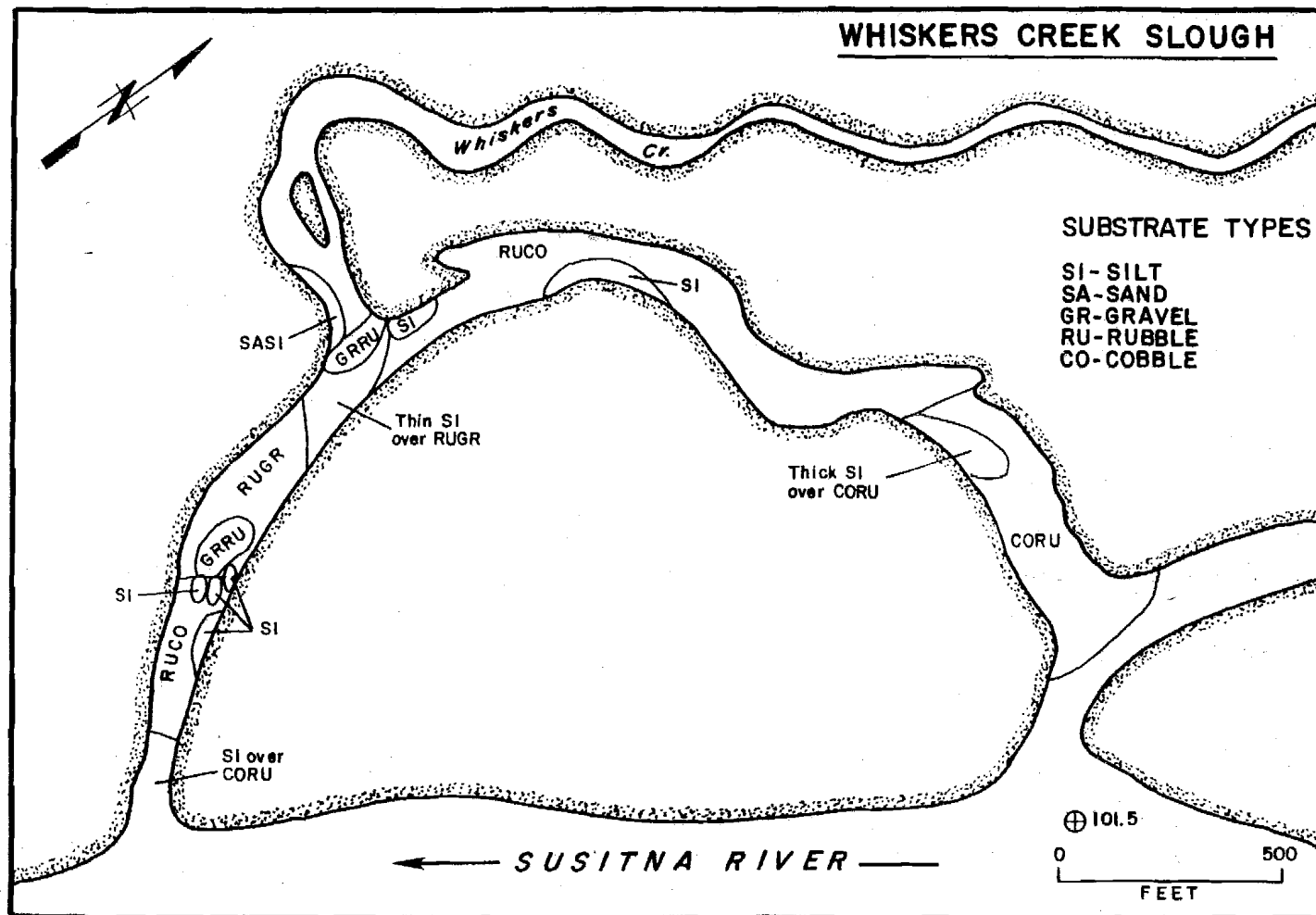
Figure 4-F-15. Whiskers Creek Slough substrate, 1982.
