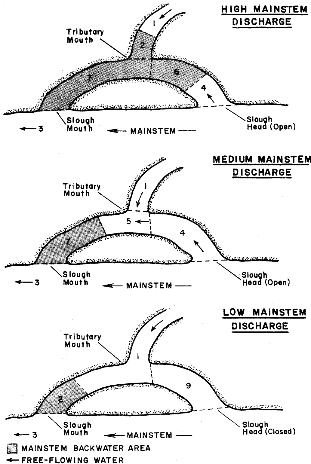
Figure 4-F-92. Hypothetical slough, with associated tributary showing presence of hydraulic zones at three different mainstem discharges.
