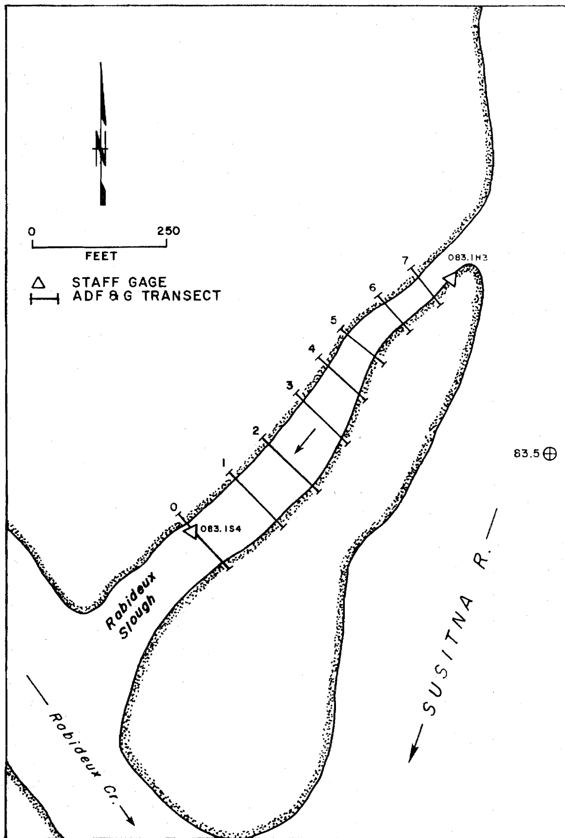
Figure 4-F-12. Rabideux Slough transects, 1982.
