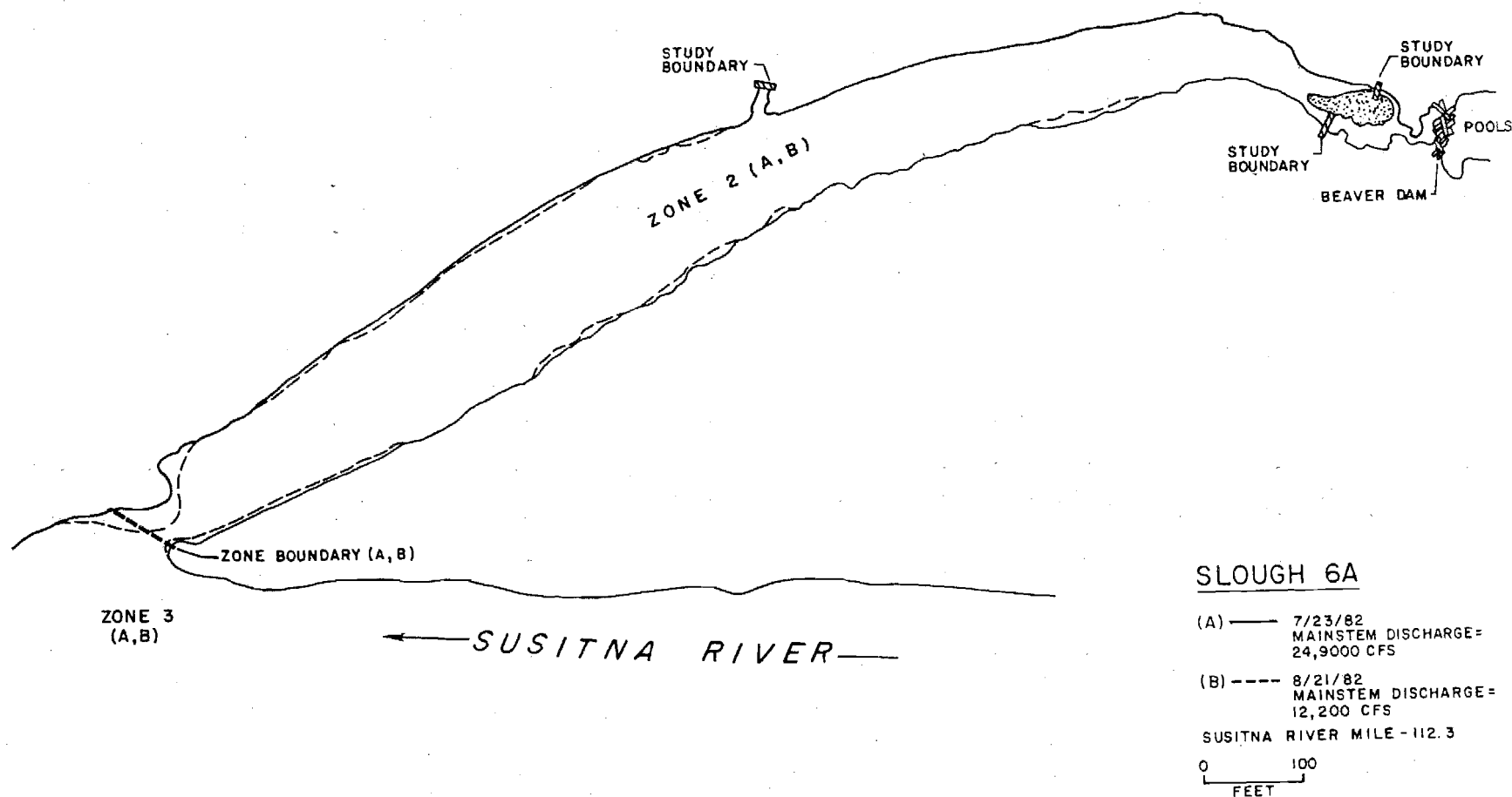
Figure 4-F-95. Map of surface areas and zone types at Slough 6A (RM 112.3) on two sampling dates. Discharges (cfs) at Gold Creek (USGS Provisional Data, 1982, 1529200).
