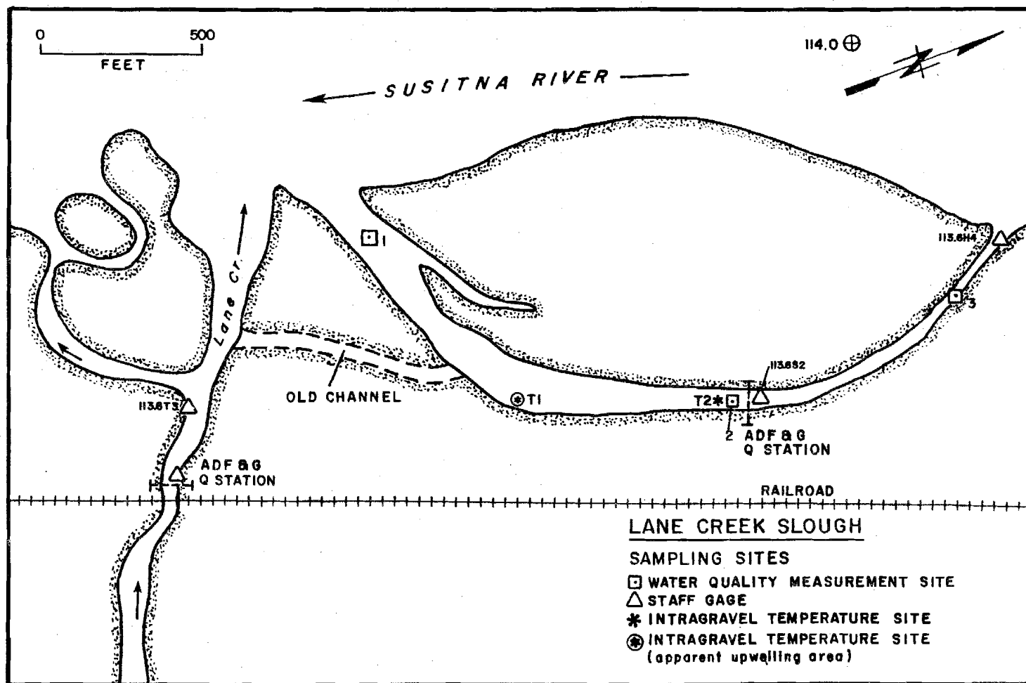
Figure 4-F-20. Lane Creek Slough sampling sites, 1982.
