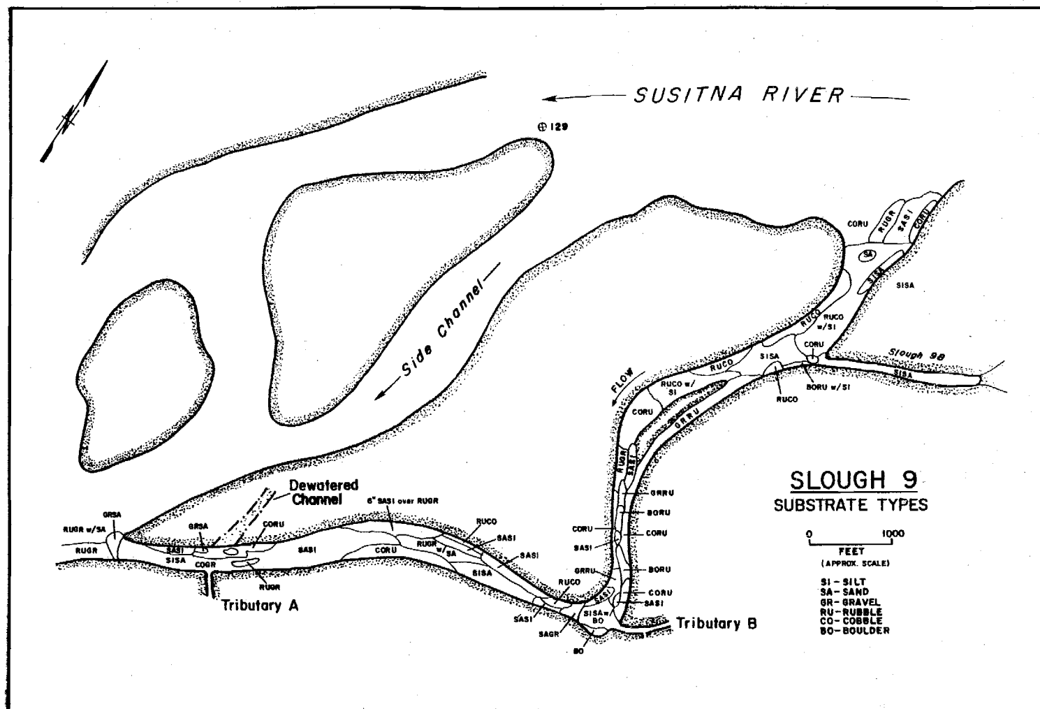
Figure 4-F-31. Slough 9 substrate, 1982.
