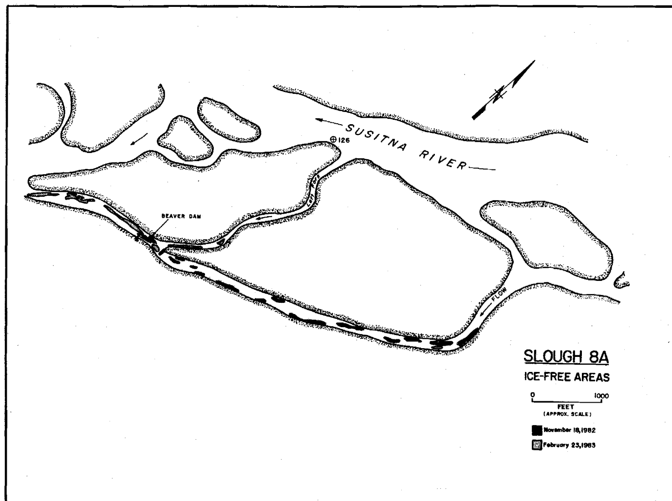
Figure 4-F-27. Slough 8A ice-free areas, winter 1982-83.
