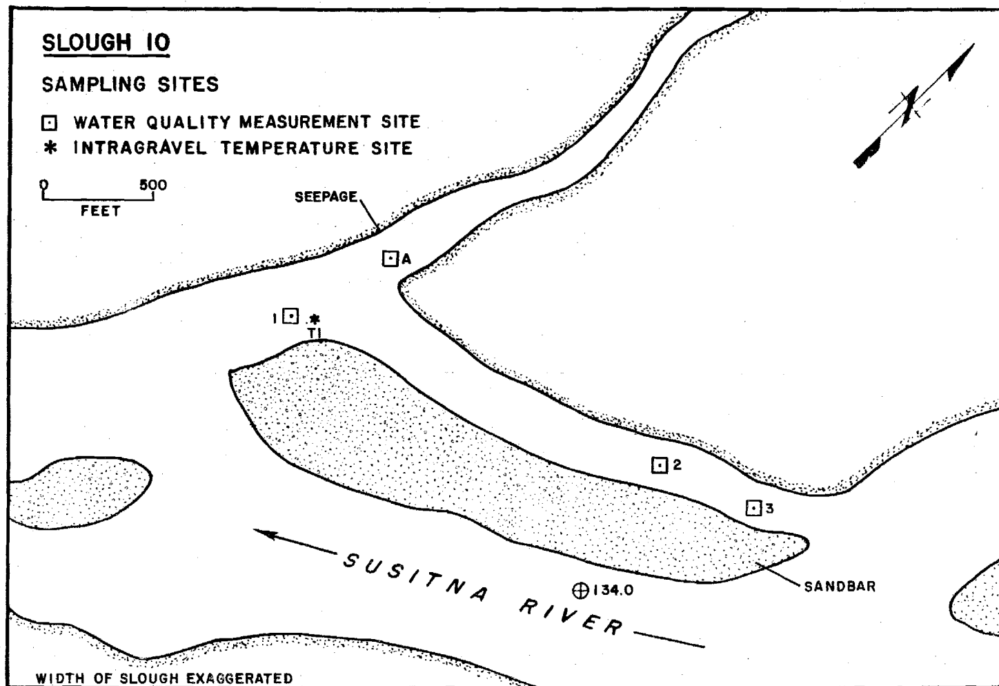
Figure 4-F-40. Slough 10 sampling sites, 1982.
