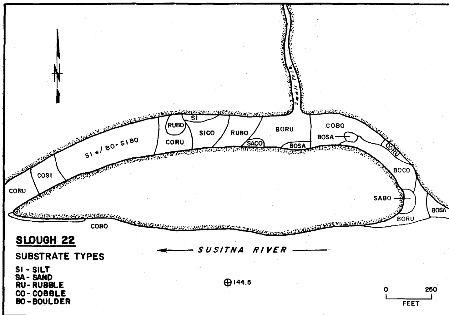
Figure 4-F-67. Slough 22 substrate, 1982.
