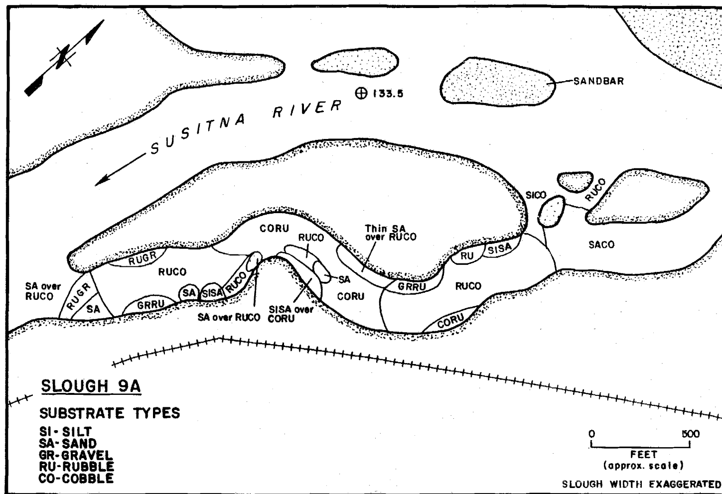
Figure 4-F-37. Slough 9A substrate, 1982.
