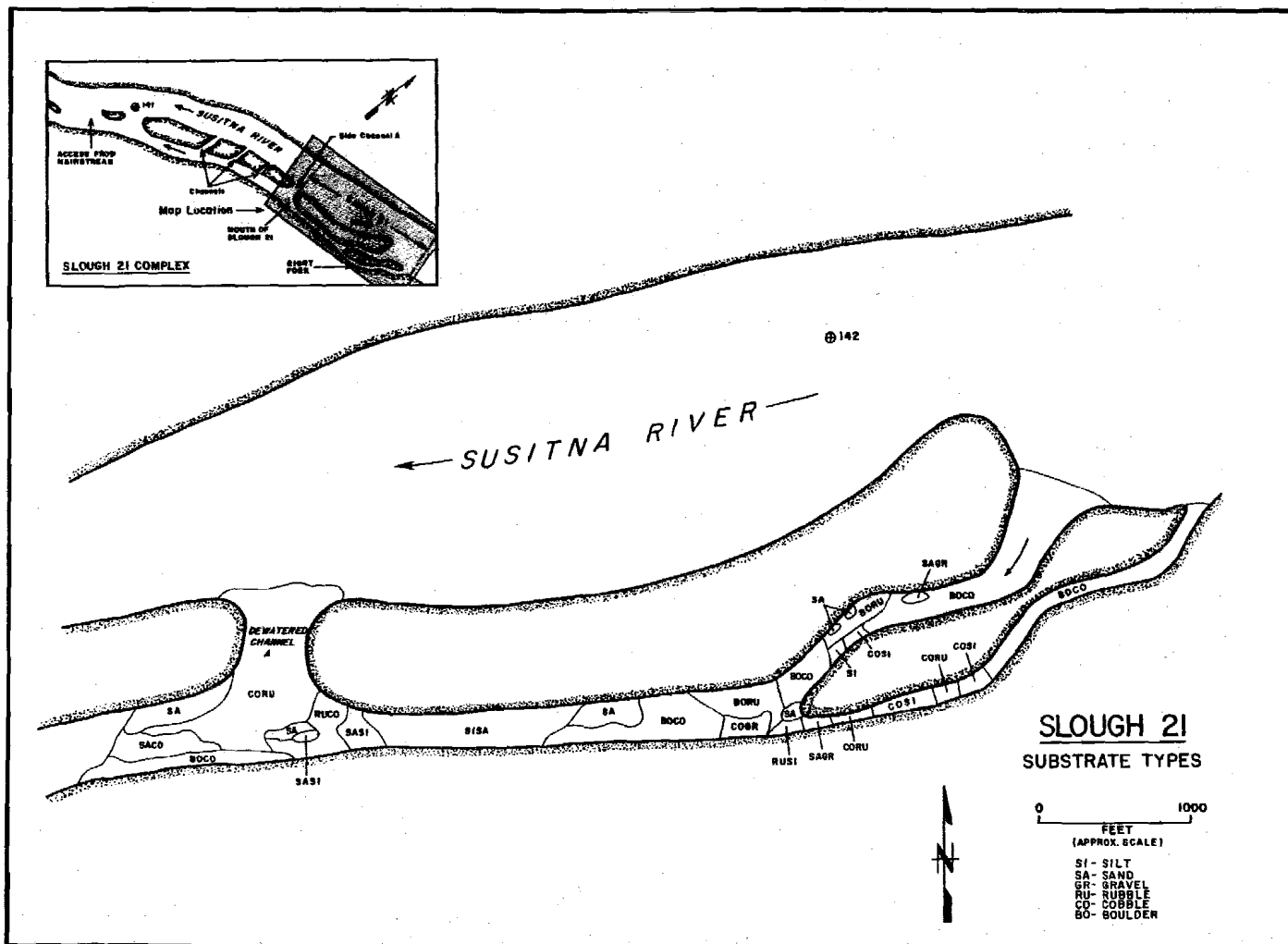
Figure 4-F-60. Slough 21 substrate, 1982.
