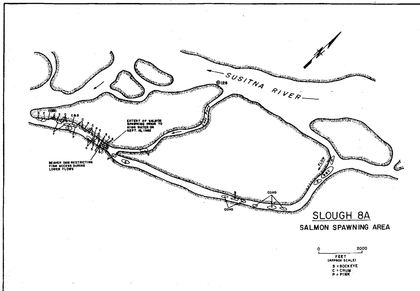
Figure 4-F-28. Slough 8A spawning areas, 1982.
