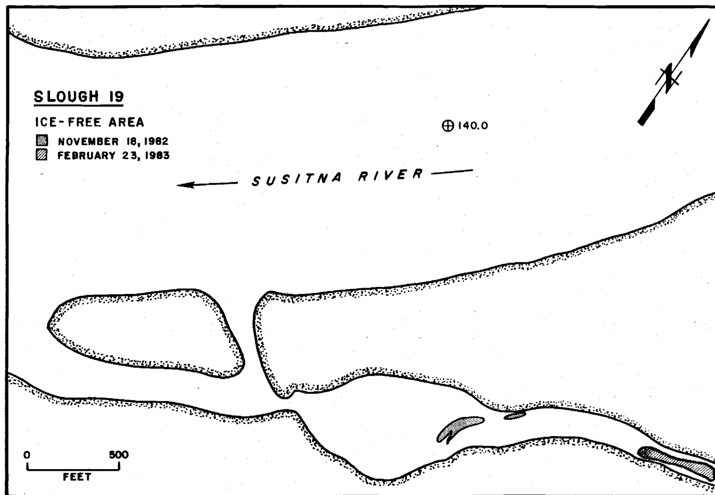
Figure 4-F-55. Slough 19 ice-free areas, winter 1982-83.
