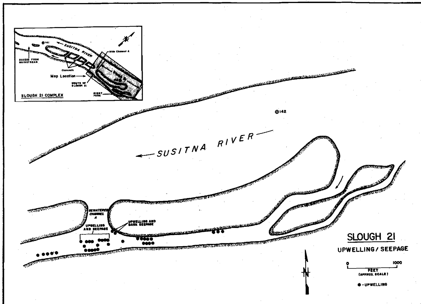
Figure 4-F-61. Slough 21 upwelling/seepage, 1982.
