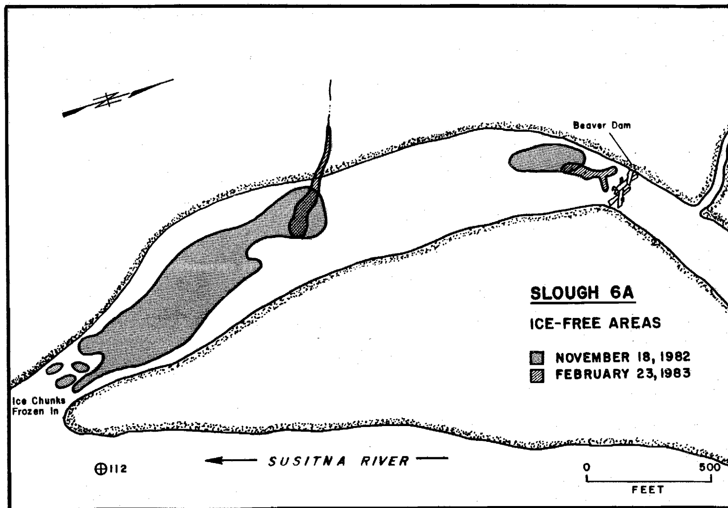
Figure 4-F-19. Slough 6A ice-free areas, winter 1982-83.
