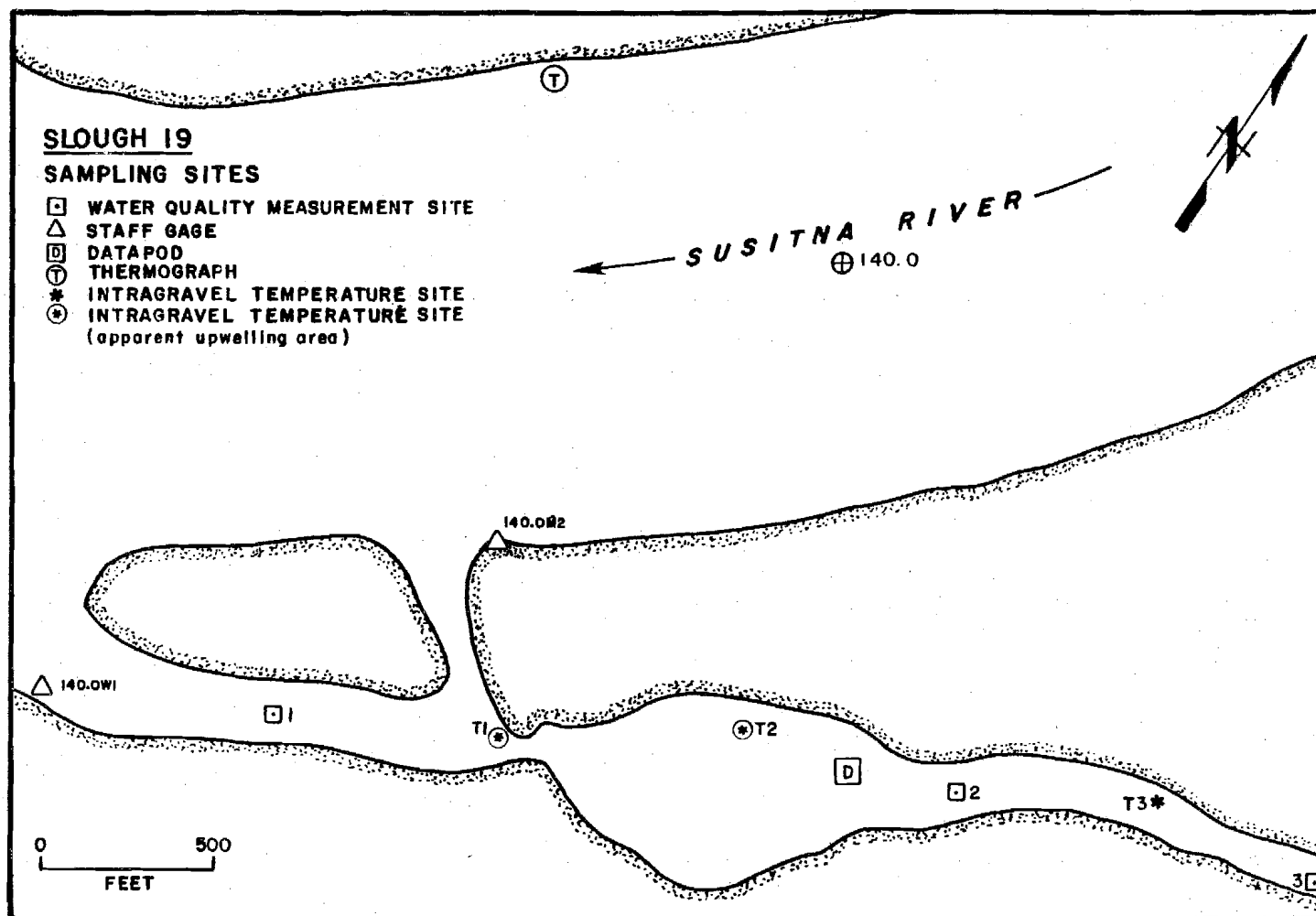
Figure 4-F-52. Slough 19 sampling sites, 1982.
