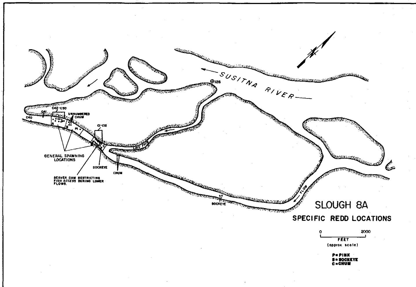
Figure 4-F-29. Slough 8A redd locations, 1982.
