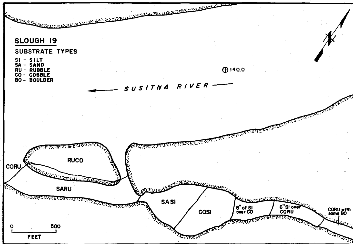
Figure 4-F-53. Slough 19 substrate, 1982.
