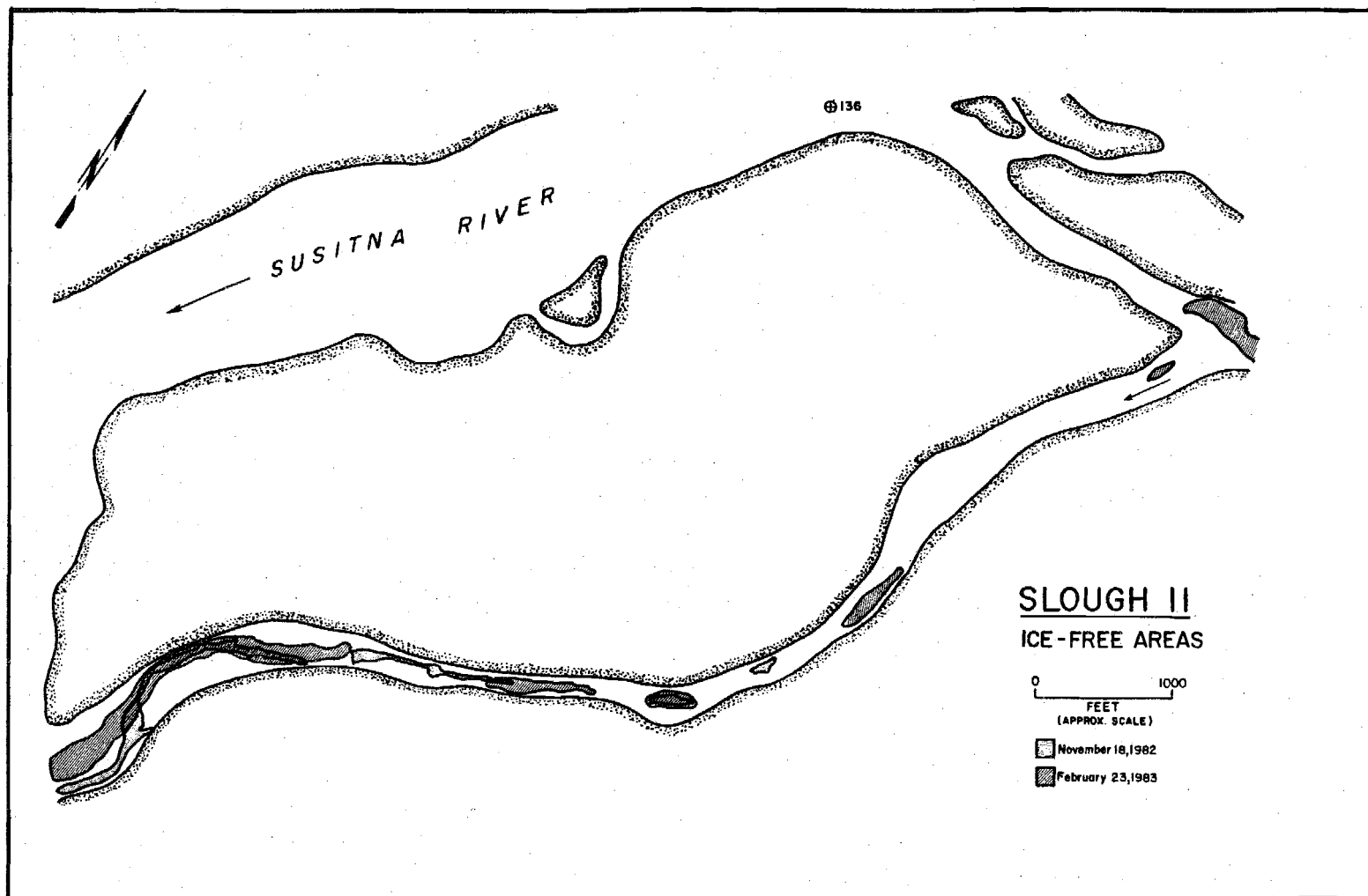
Figure 4-F-46. Slough II ice-free areas, winter 1982-83.
