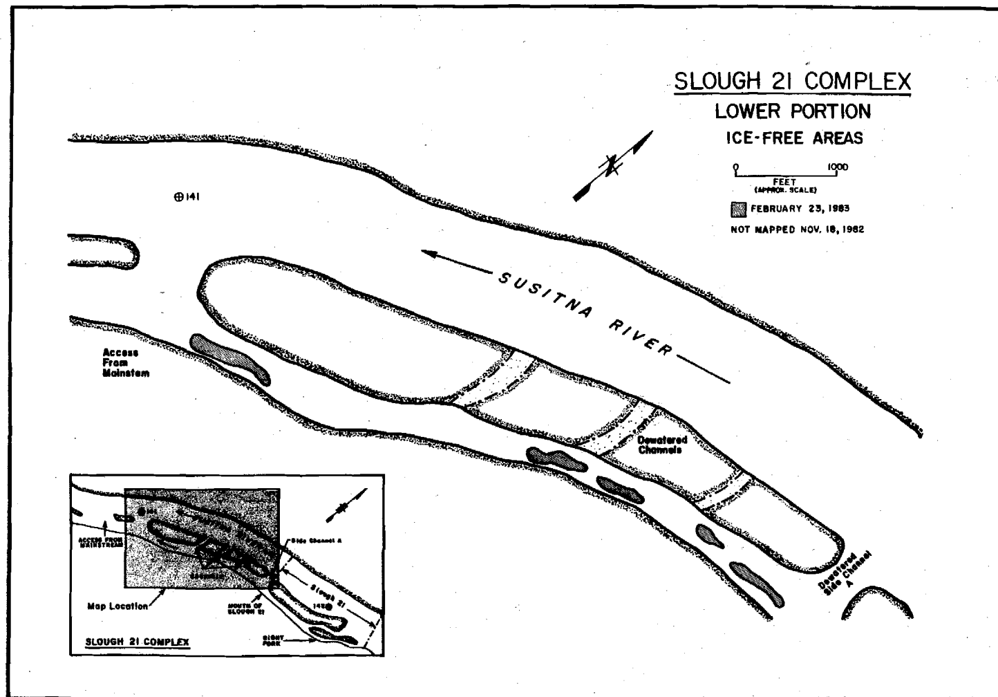
Figure 4-F-63. Slough 21 Complex ice-free areas, winter 1982-83.
