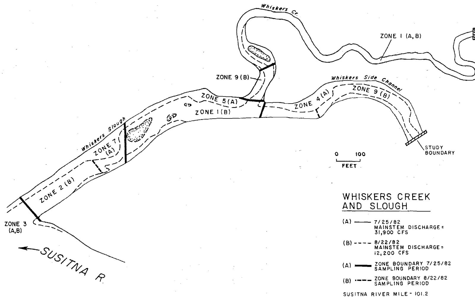
Figure 4-F-94. Map of surface areas and zone types at Whiskers Creek and Slough (RM 101.2) on two sampling dates. Discharges at Gold Creek (USGS Provisional Data, 1982, 1529200).
