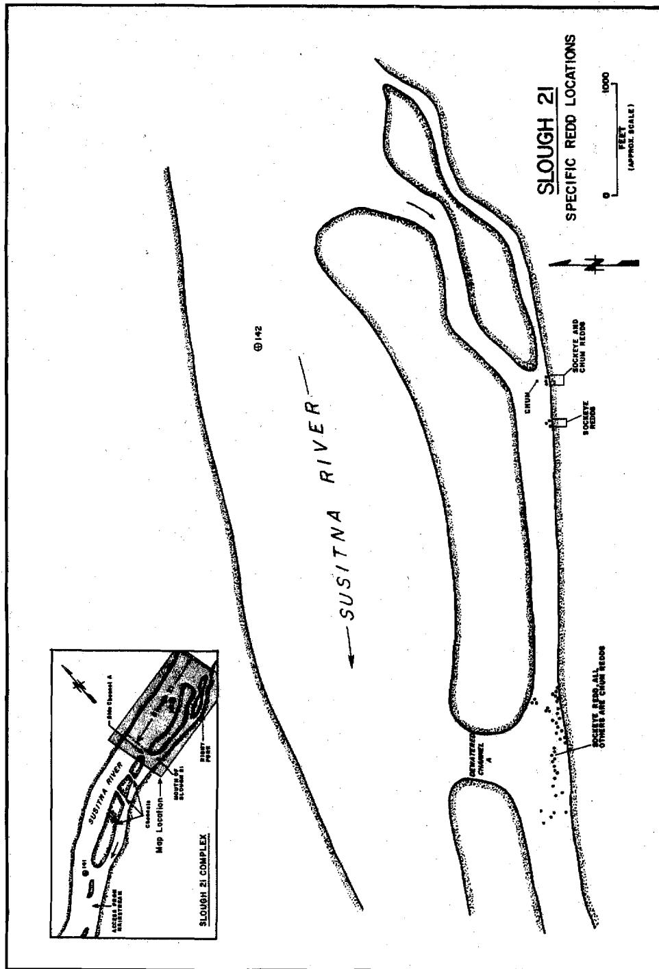
Figure 4-F-65. Slough 21 redd locations, 1982.
