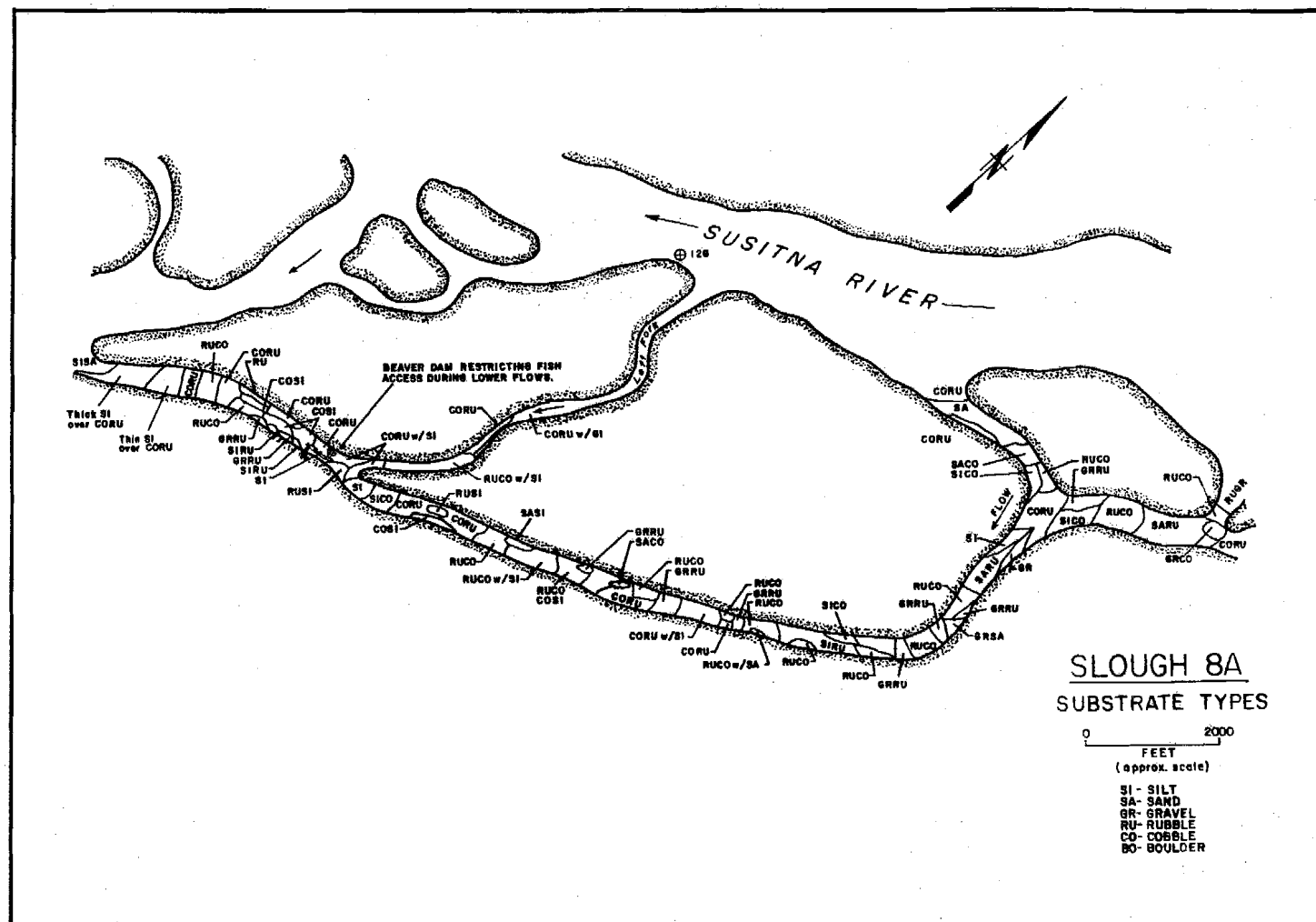
Figure 4-F-25. Slough 8A substrate, 1982.
