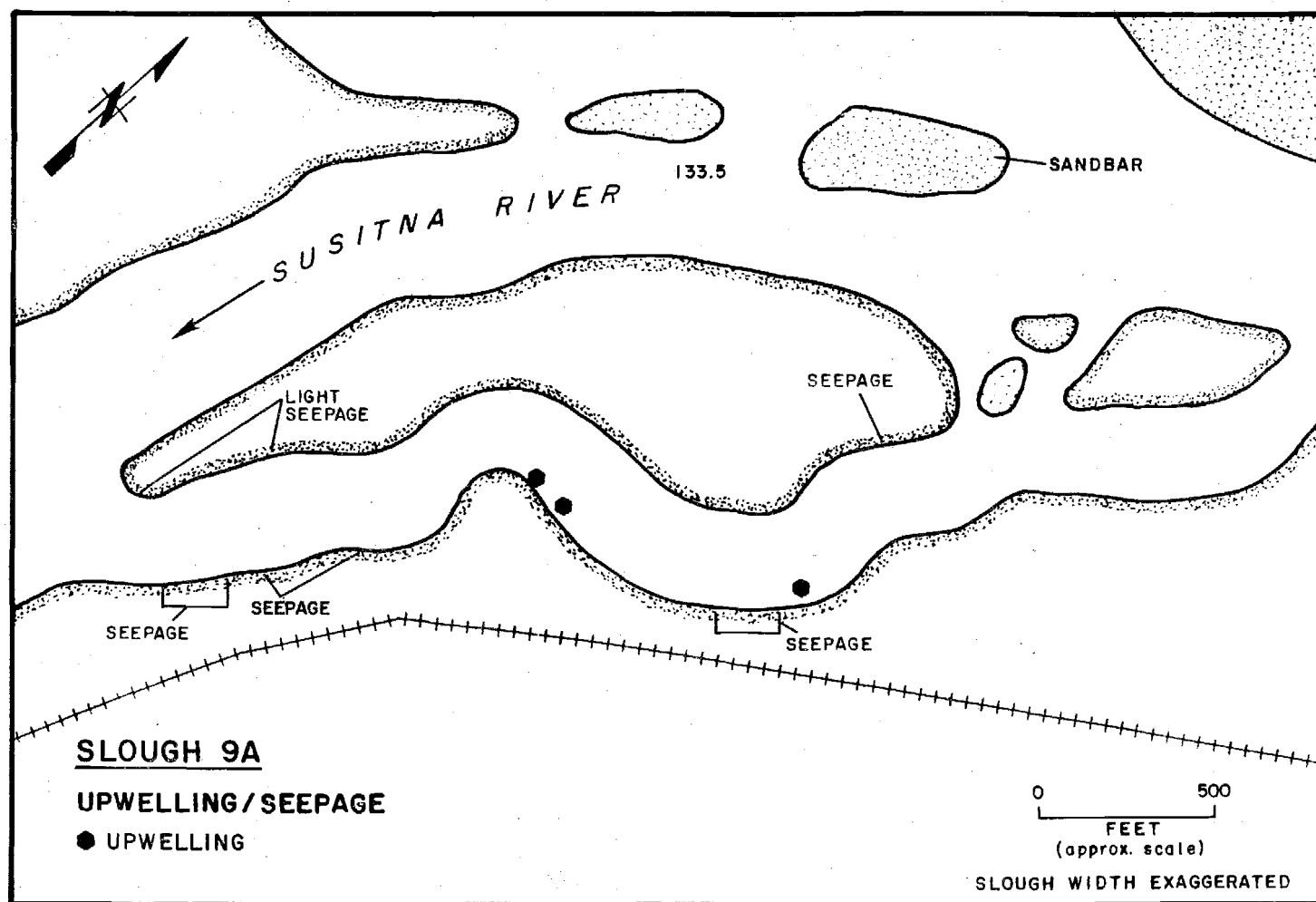
Figure 4-F-38. Slough 9A upwelling/seepage, 1982.
