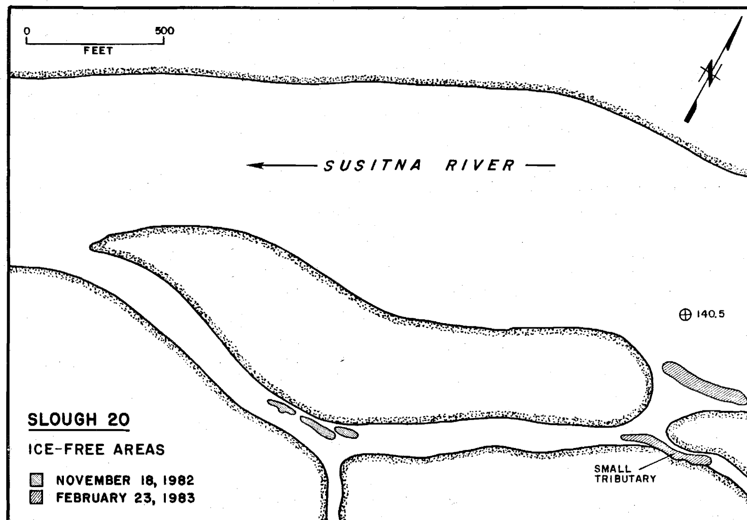
Figure 4-F-58. Slough 20 ice-free areas, winter 1982-83.
