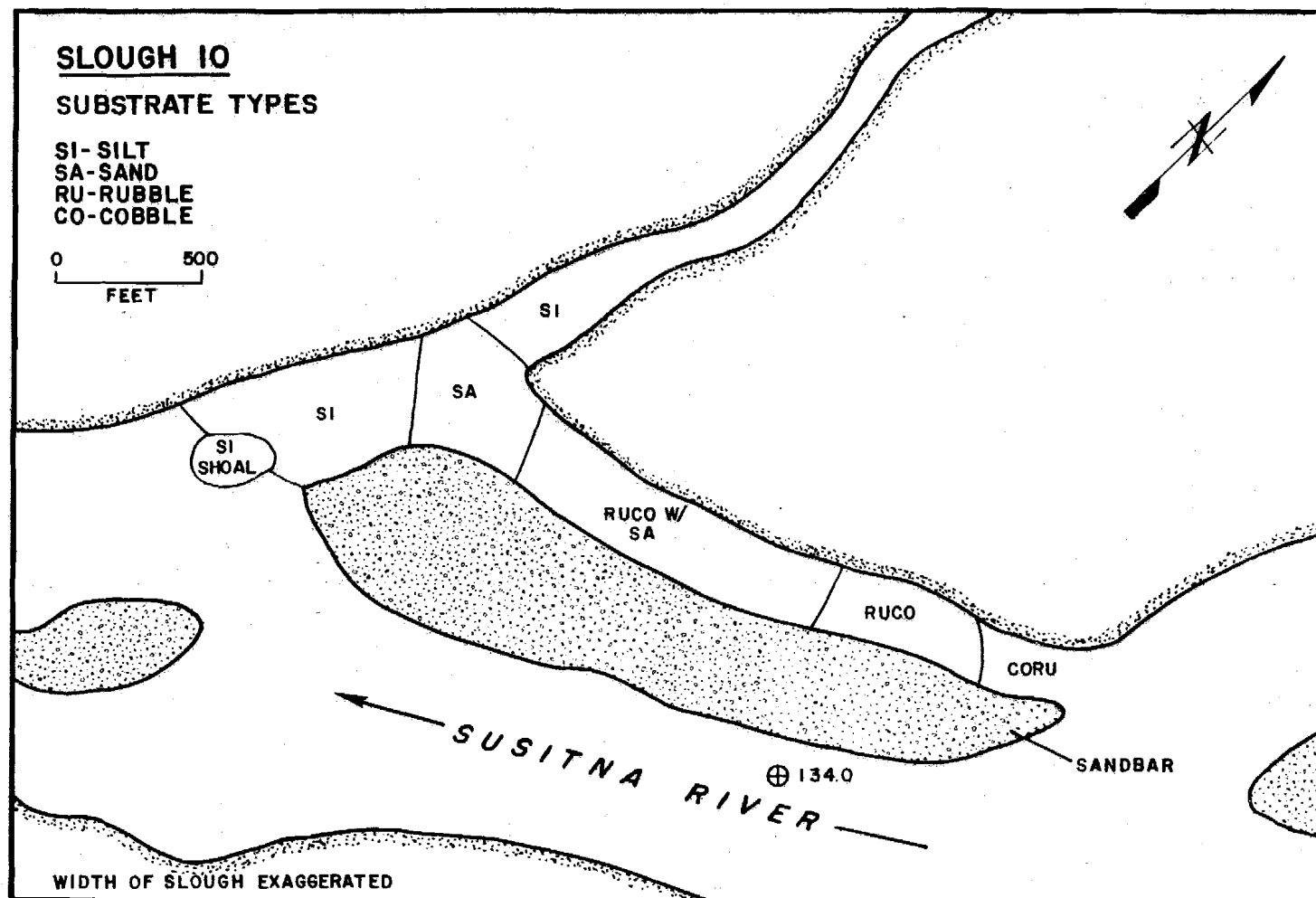
Figure 4-F-41. Slough 10 substrate, 1982.
