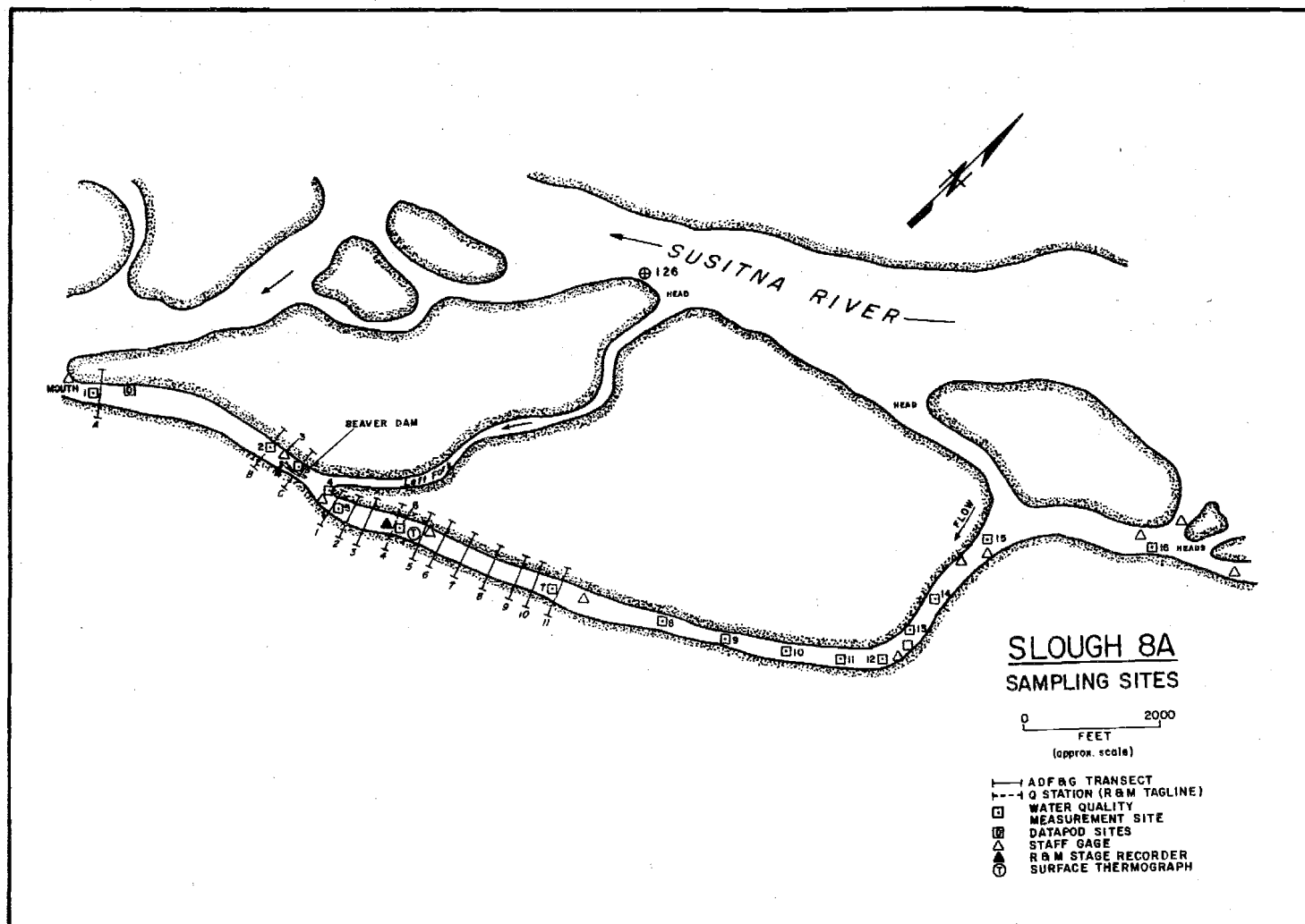
Figure 4-F-24. Slough 8A sampling sites, 1982.
