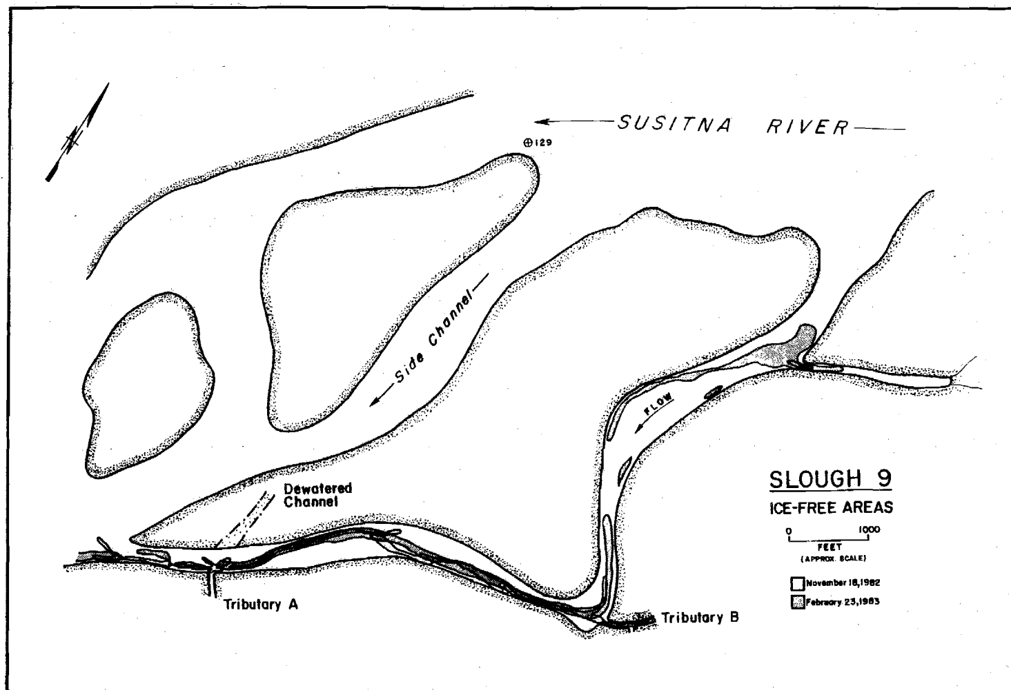
Figure 4-F-33. Slough 9 ice-free areas, winter 1982-83.
