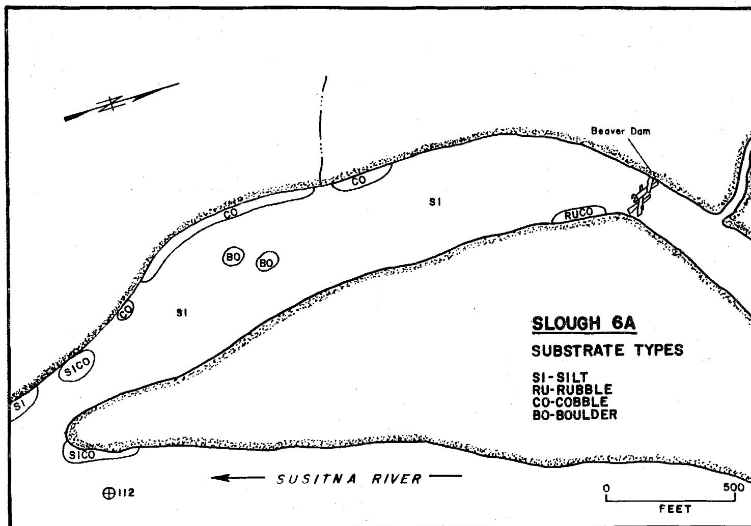
Figure 4-F-18. Slough 6A substrate, 1982.
