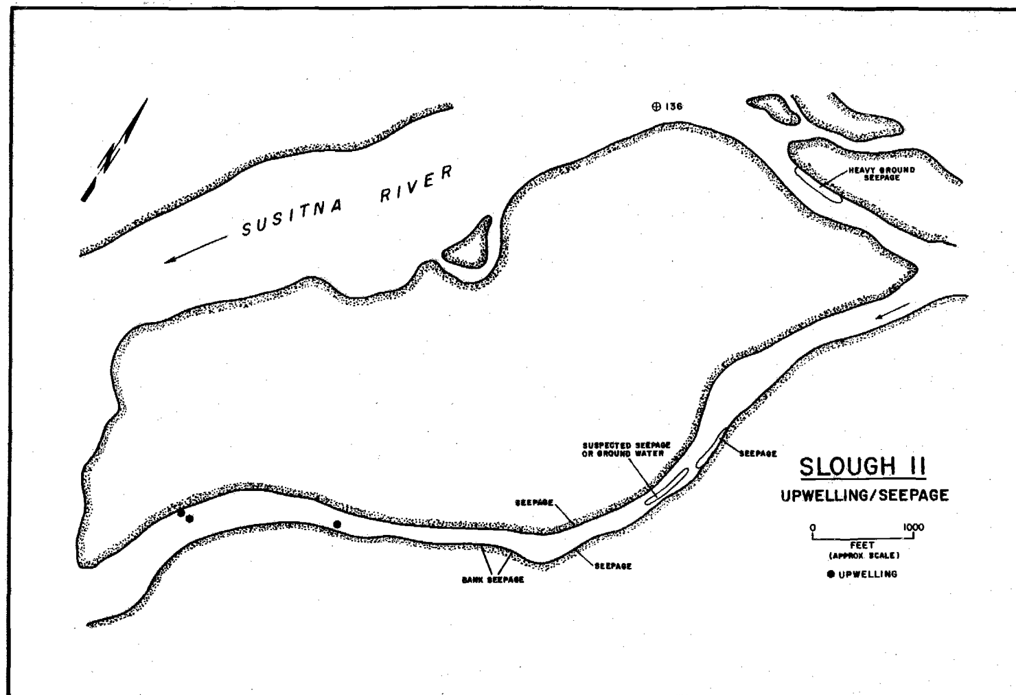
Figure 4-F-45. Slough II upwelling/seepage, 1982.
