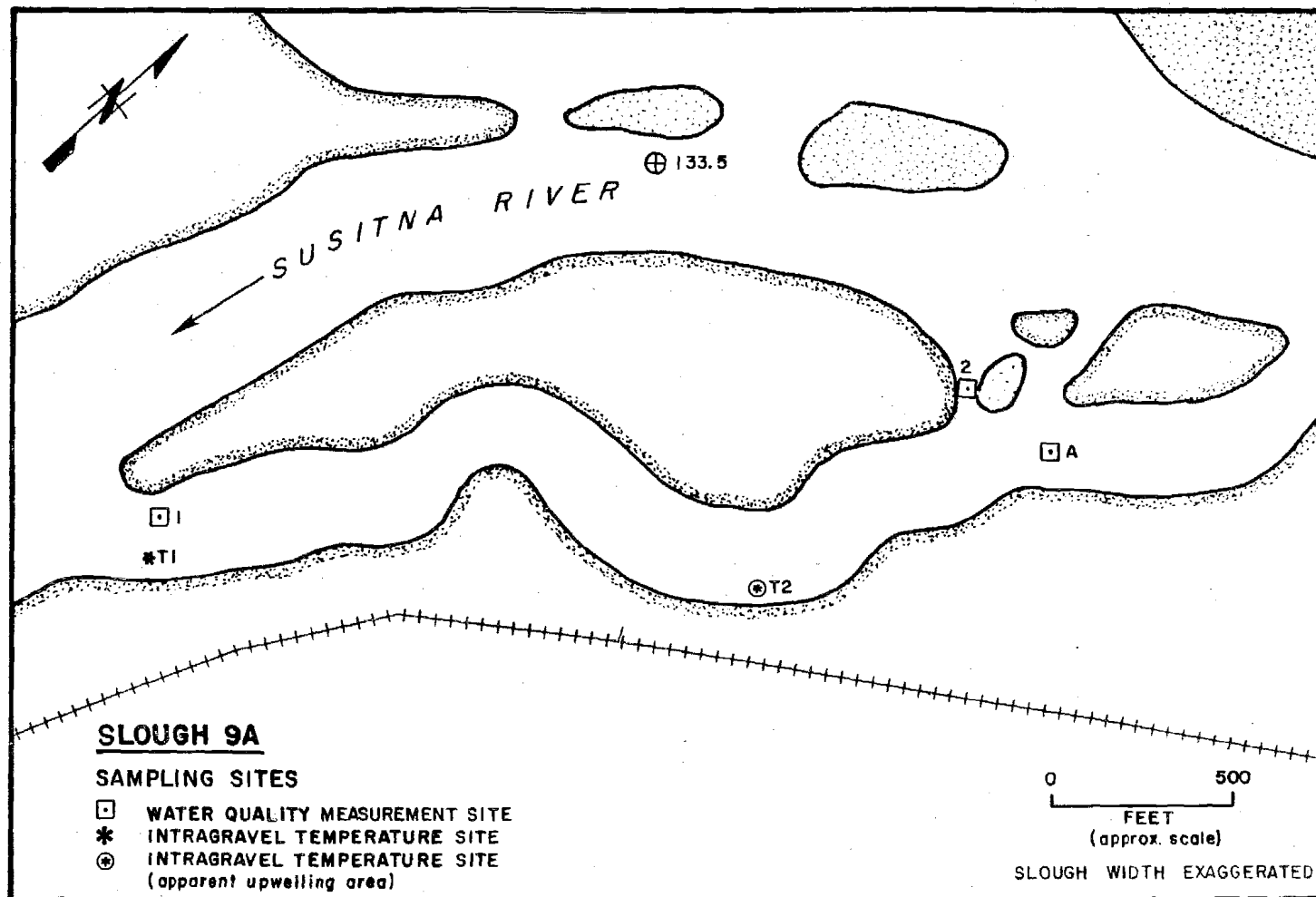
Figure 4-F-36. Slough 9A sampling sites, 1982.
