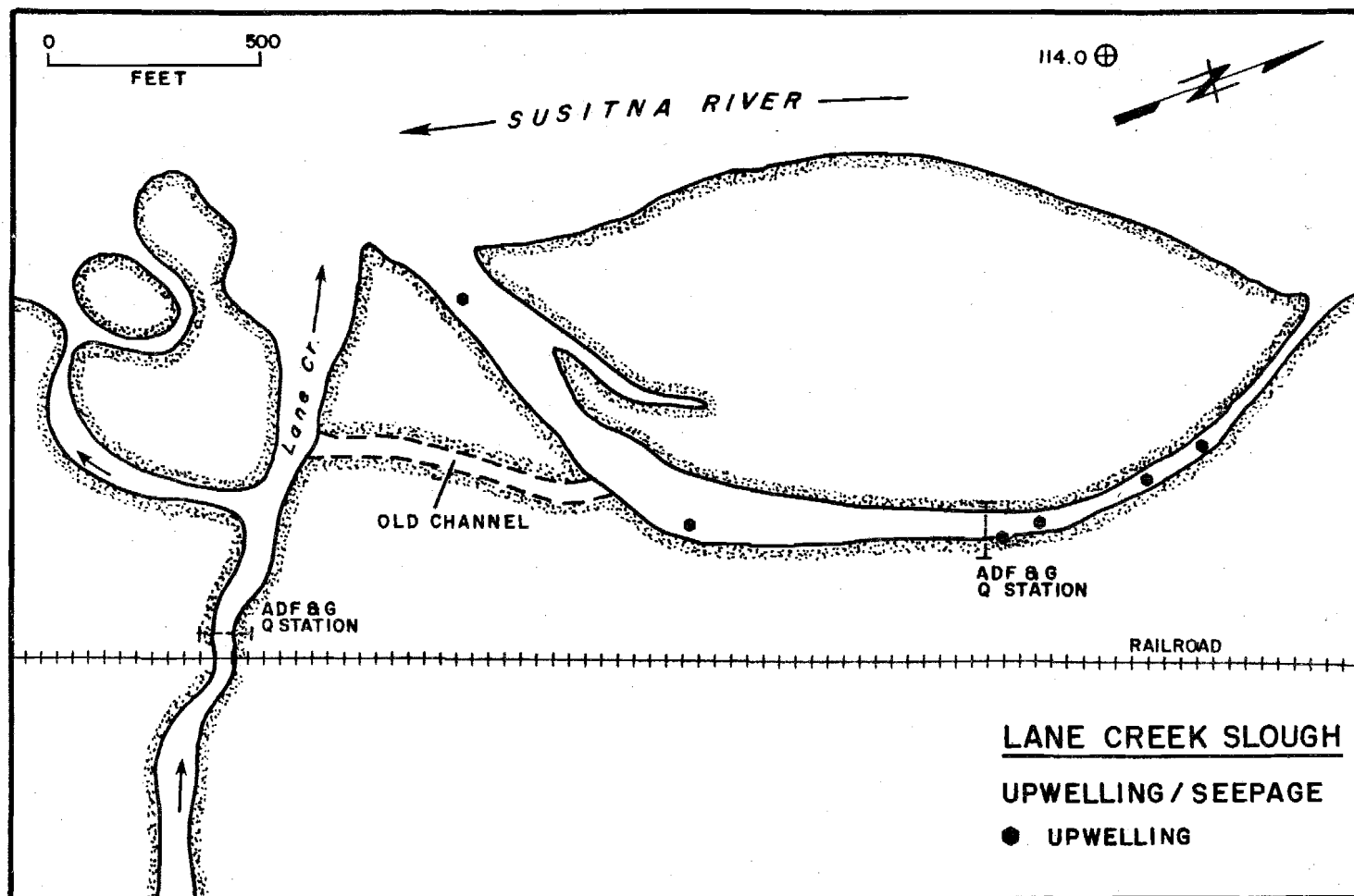
Figure 4-F-22. Lane Creek Slough upwelling/seepage, 1982.
