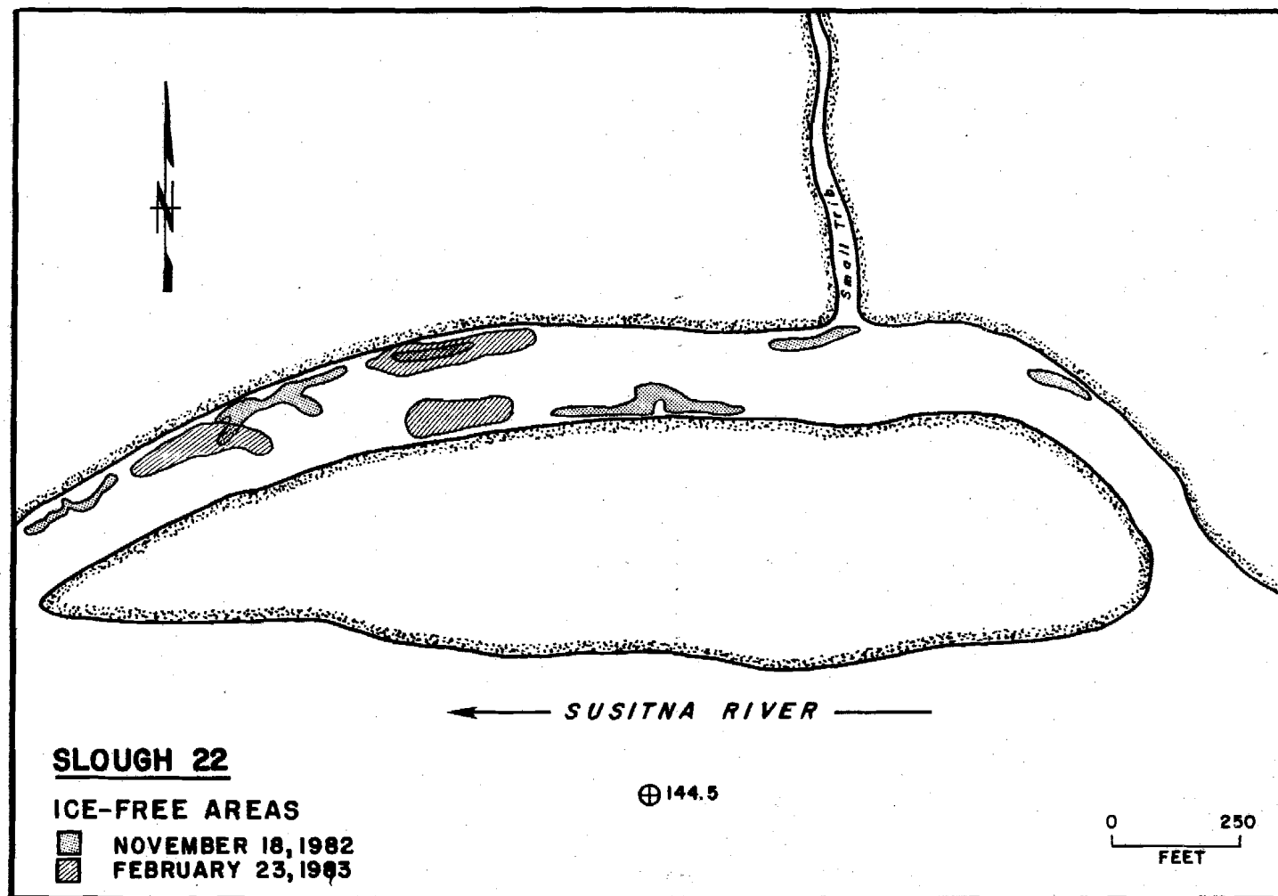
Figure 4-F-69. Slough 22 ice-free areas, winter 1982-83.
