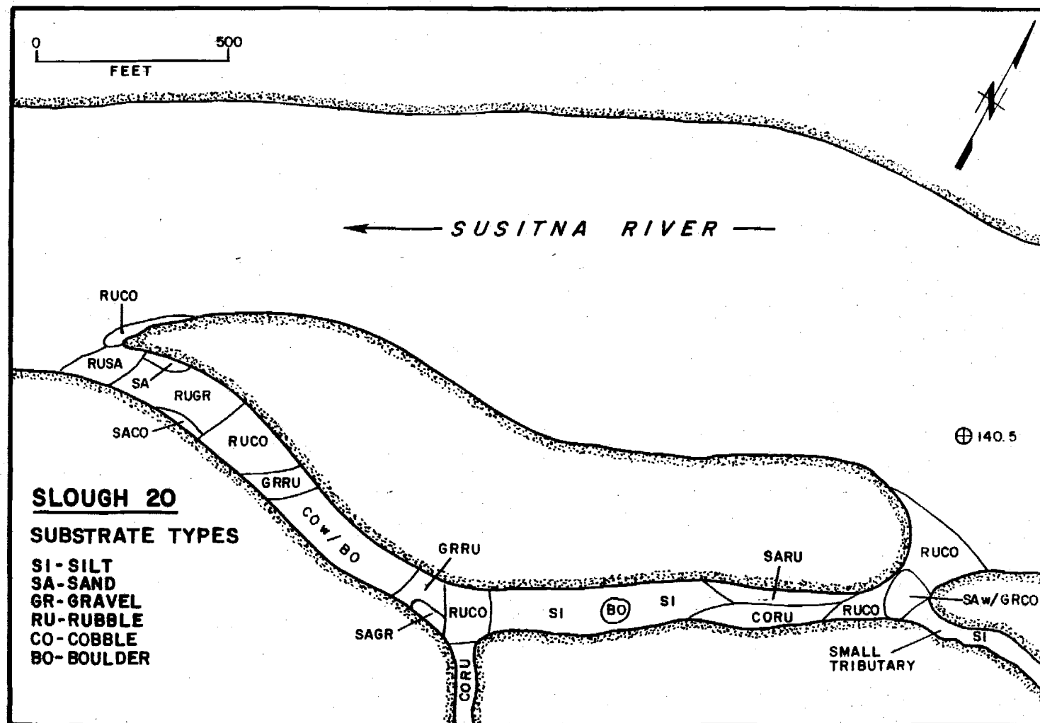
Figure 4-F-57. Slough 20 substrate, 1982.
