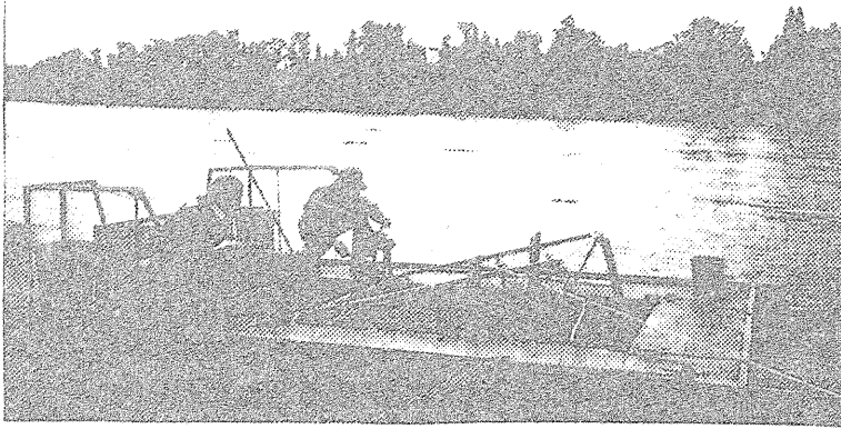
Winching up the inclined plane of the downstream migrant trap to clean the screen surfaces.
