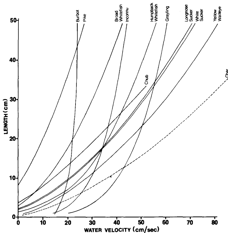
Figure E-1. The relationship between fish fork length and ability to move 100 m against water velocities of 0-80 cm/sec in 10 min. The same curves may also be used to indicate the ability to make progress against these currents over shorter distances. For instance, to cross a 50-m barrier in 10 min the curves should be shifted 8 cm/sec to the right; to cross a 25-m barrier in 10 min the curves should be shifted 12 cm/sec to the right. The line for char is derived from the hypothetical equation V = 17 L^{0.5} and represents the measured value in these experiments (from Jones 1973).
