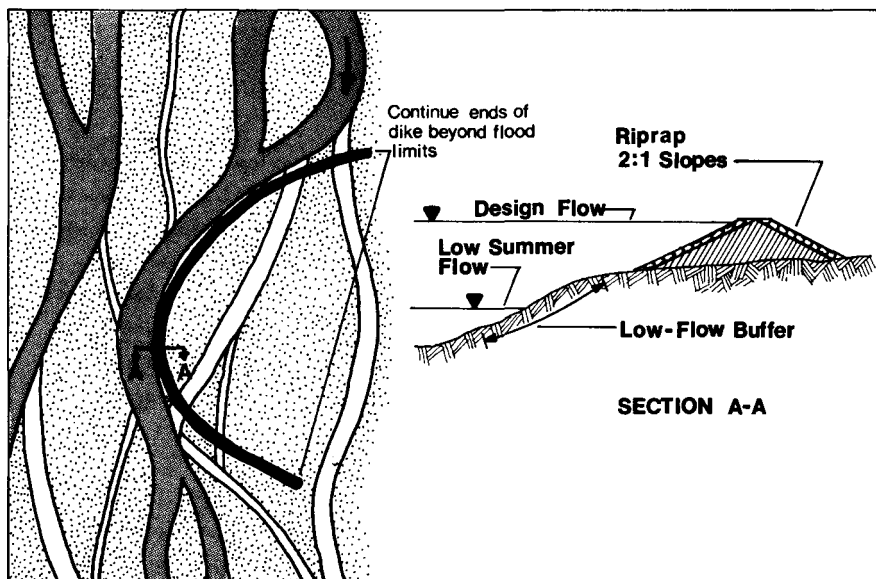
Figure C-1. Dike design considerations.
