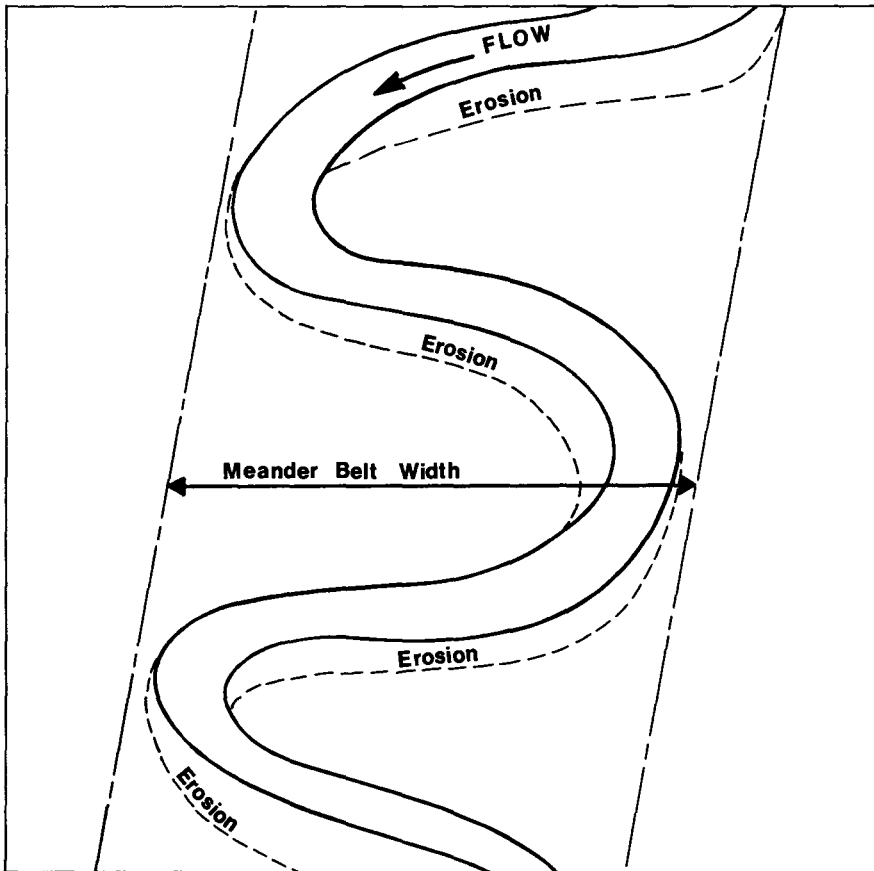
Figure A-7. Schematic of a meandering river showing the expected zones of erosion as the river meanders migrate down the valley.
