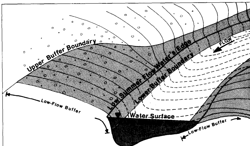
Figure 4. Schematic diagram of the low-flow buffer.
