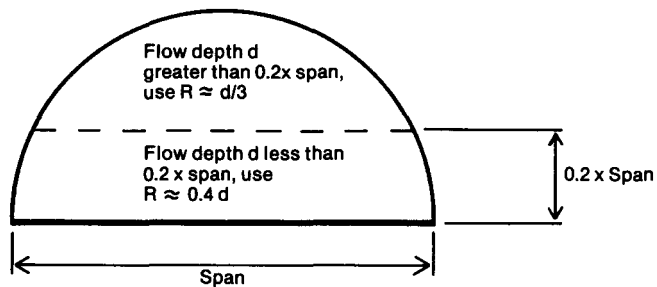
Figure H-1. Methods of estimating hydraulic radius of culverts.
