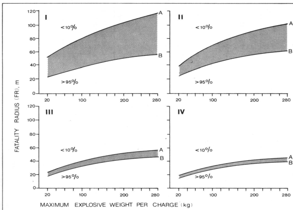
Figure G-1. Relationship of kilogram per charge to fatality radii (FR): A = 10-20% mortality, B = 95% mortality.
