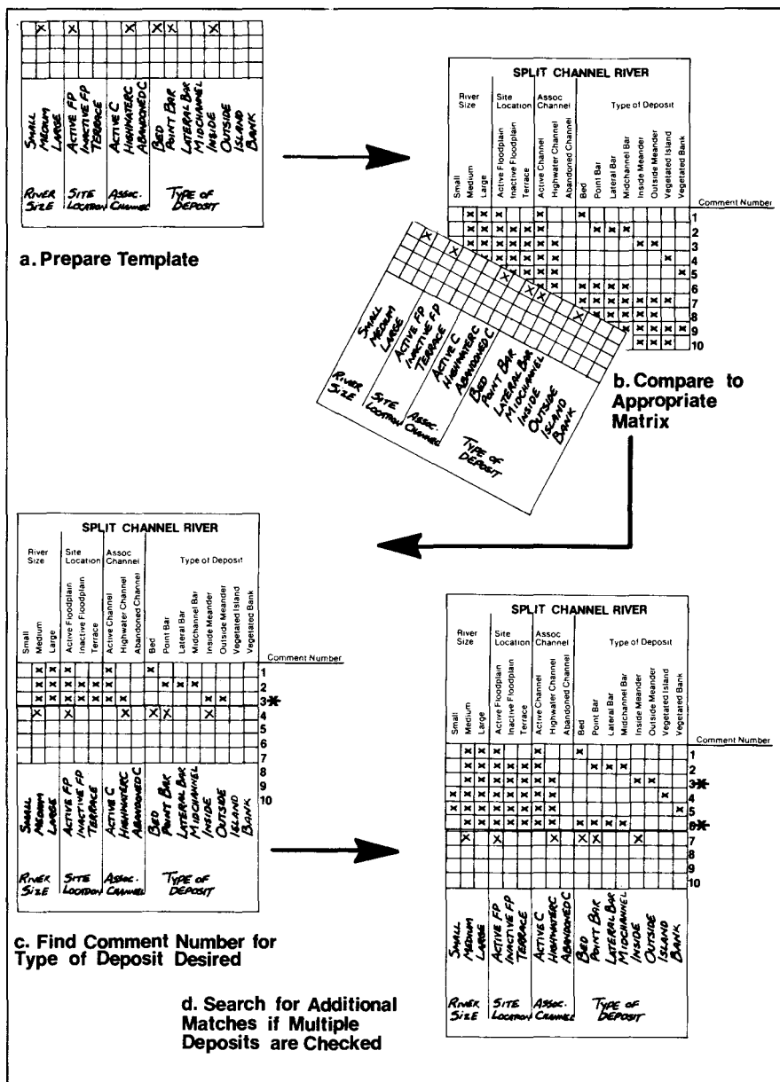
Figure 12. Example of how the completed template is matched to determine availability of gravel.
