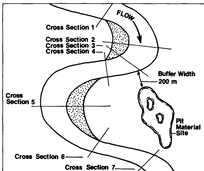
Figure A-13. Schematic of an example of buffer height design.
