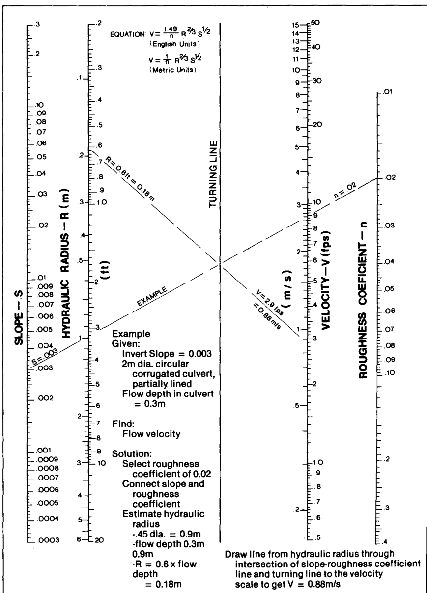
Figure H-2. Nomograph for solution of Manning's equation.
