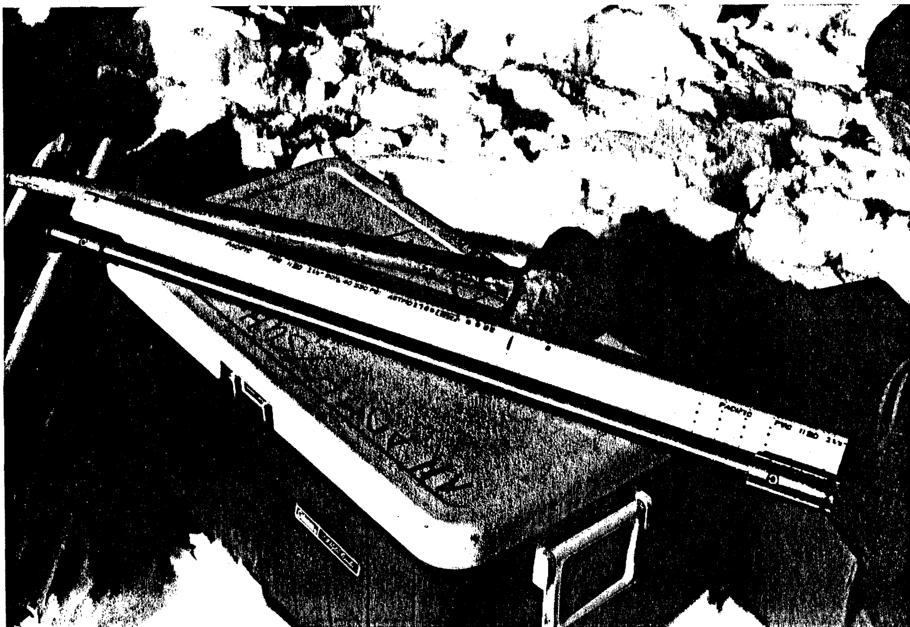
Plate 1. Standpipe (with 48 one-eighth inch holes) used for monitoring intragravel water quality and driver used for installation.
