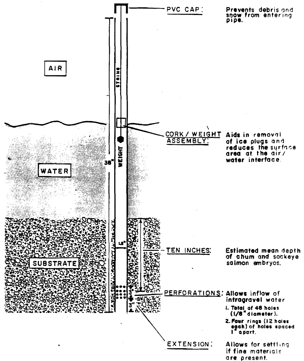
Figure 10. Diagram of a polyvinyl chloride (PVC) standpipe installed by ADF&G in substrate.
