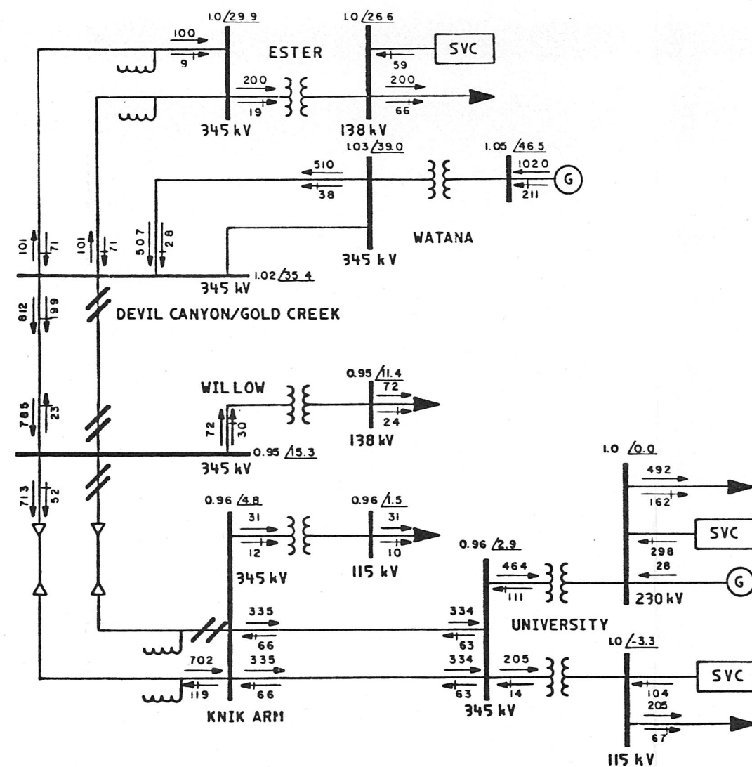
1993 PEAK LOAD, DOUBLE CONTINGENCY
