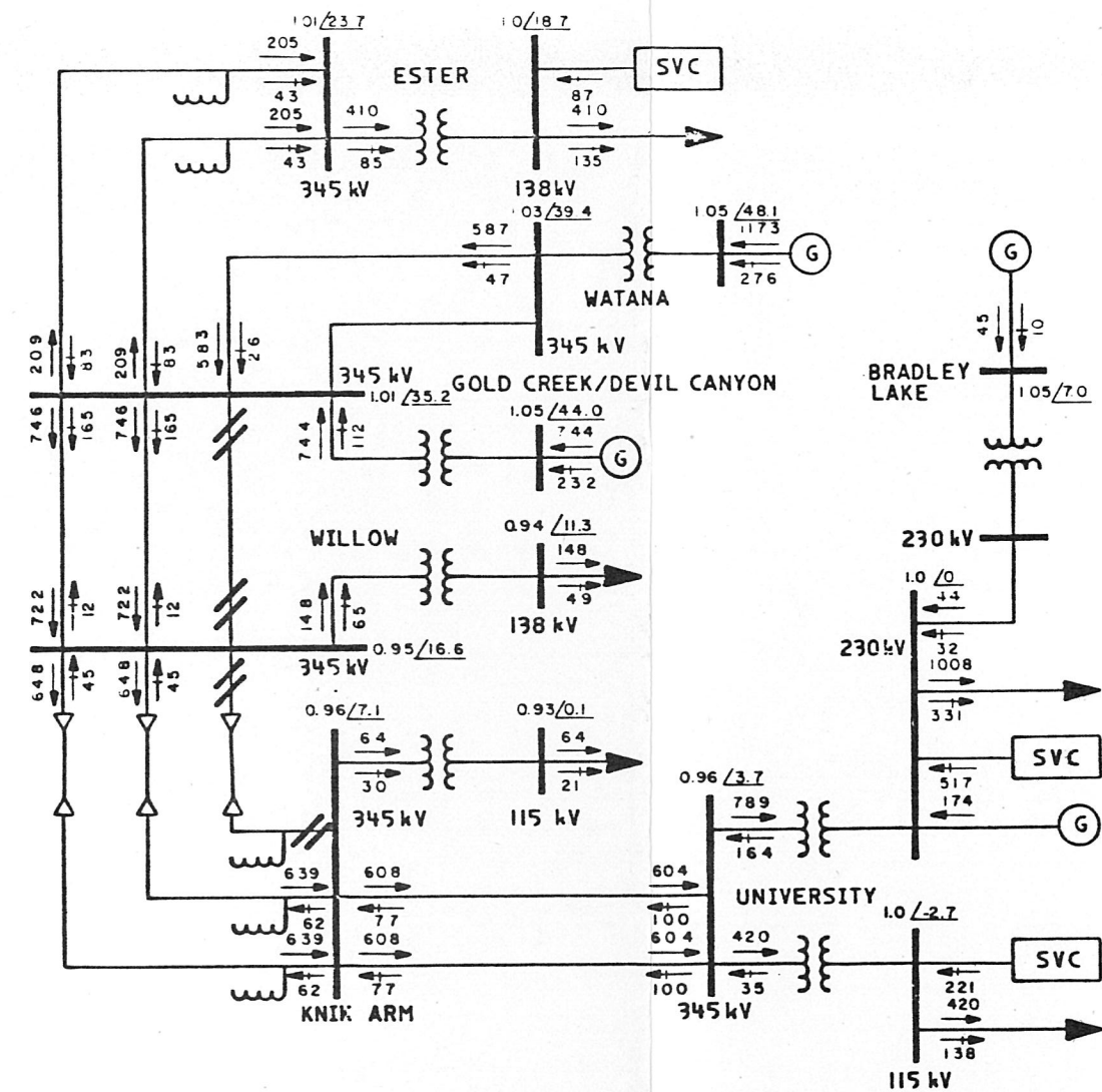
2002 PEAK LOAD, DOUBLE CONTINGENCY
