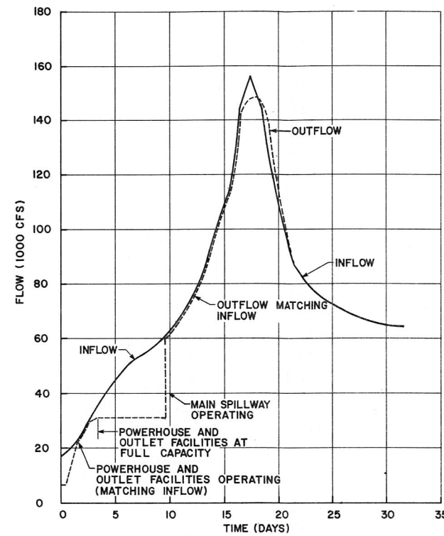
1:10,000 YEAR FLOOD
