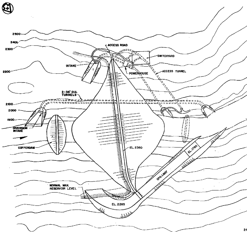
GENERAL ARRANGEMENT SCALE: A
