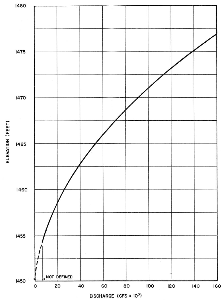
TAILWATER RATING
