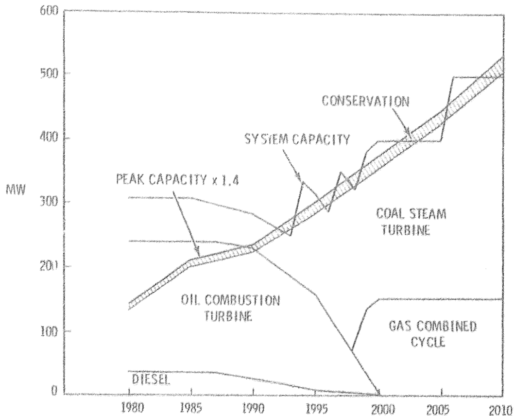
FIGURE 3.4. Plan 1A: Base Case Without Upper Susitna, Illustrating Effects of Conservation for Fairbanks-Tanana Valley
