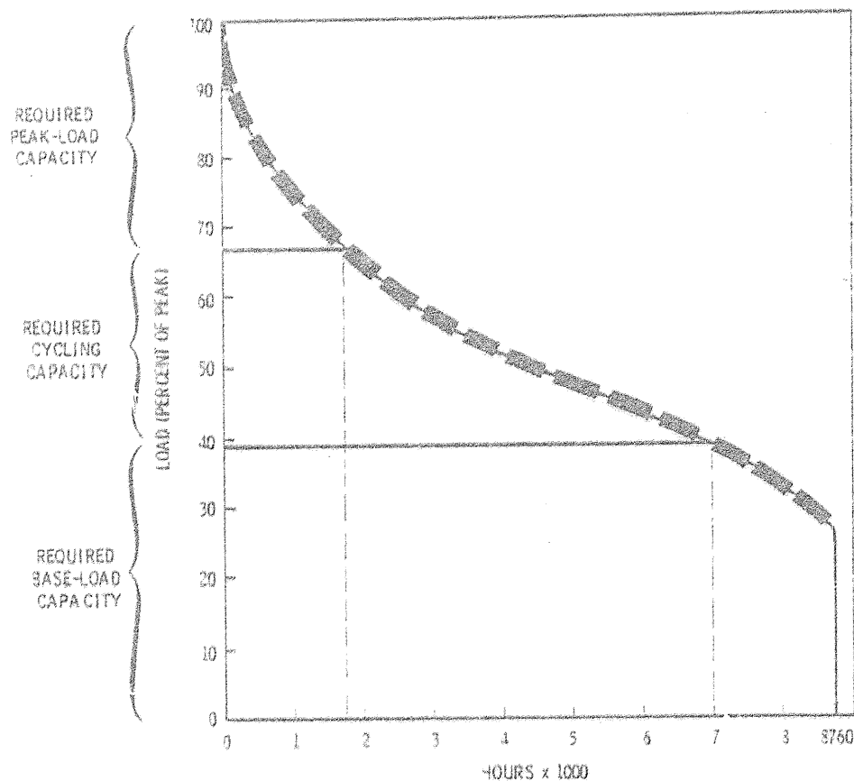
FIGURE 2.15. Typical Load Duration Curve for the Railbelt
