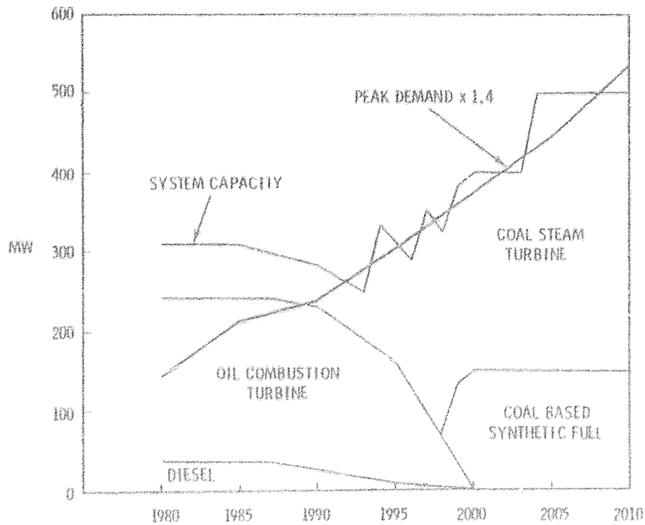
FIGURE 3.12. Plan 3: Increased Use of Coal for Fairbanks-Tinana Valley
