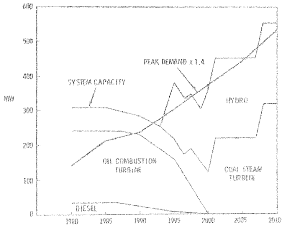
FIGURE 3.6. Plan 1B: Base Case with Upper Susitna for Fairbanks-Tanana Valley
