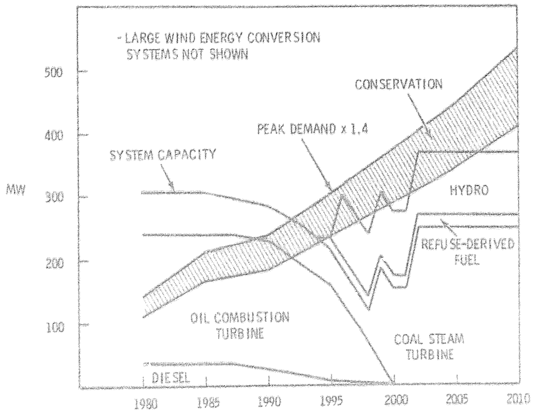
FIGURE 3.8. Plan 2A: High Conservation and Use of Renewables Without Upper Susitna for Fairbanks-Tanana Valley
