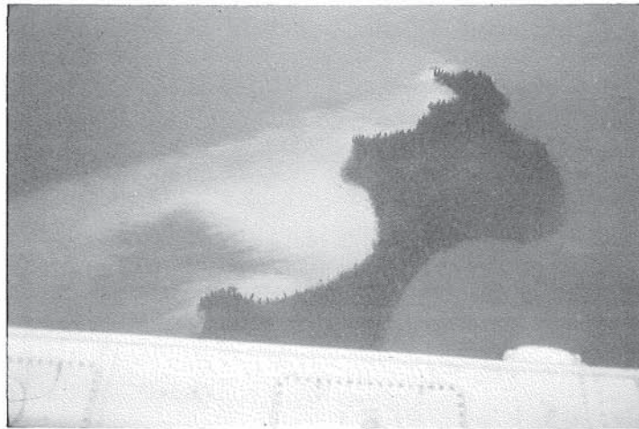
FIG. 10. Plumes of sediment from newly flooded ground, Southern Indian Lake (courtesy of Freshwater Institute, photo by G. McCullough).
