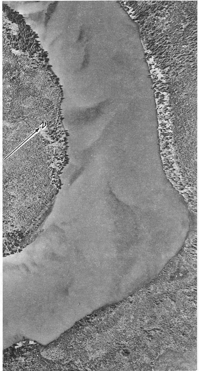
FIGURE 12.—Kenai River between approximate river miles 47.5 and 46.9. Crests of large crescentic gravel dunes appear just below water surface as darker areas. Flow is from bottom of photograph toward top. Scale 1:4,800 or 1 in. = 400 ft. Date: July 11, 1977. Photograph credit: U.S. Army Corps of Engineers.
