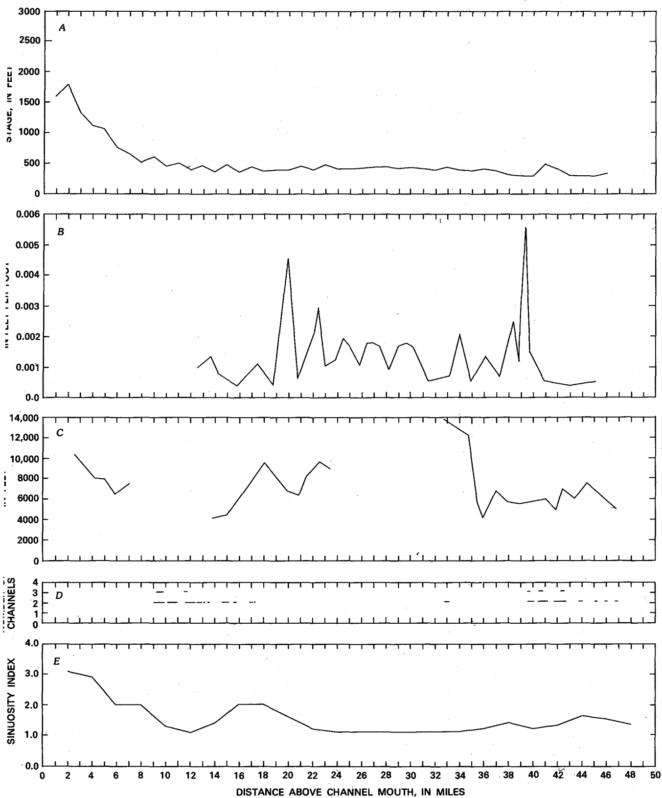
FIGURE 6.—Distance above channel mouth (in river miles) against: channel width at bankfull stage (A), slope of water surface (B), meander wavelength (C), number of channels (D), and sinuosity index (E).
