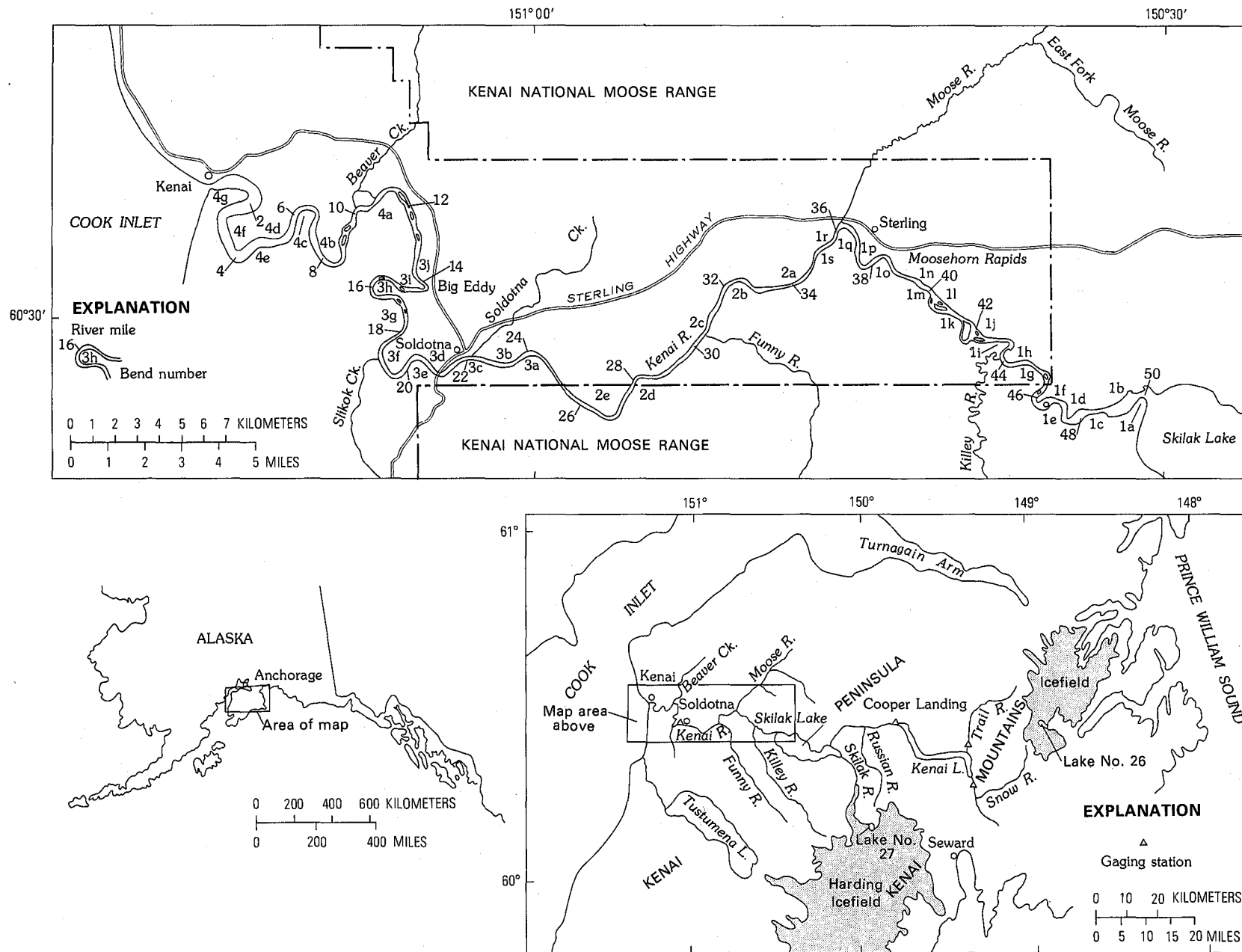
FIGURE 1.— Configuration of the Kenai River downstream from Skilak Lake. Glacial lakes capable of yielding potentially hazardous flood discharges are numbered in accordance with Post and Mayo (1971).
