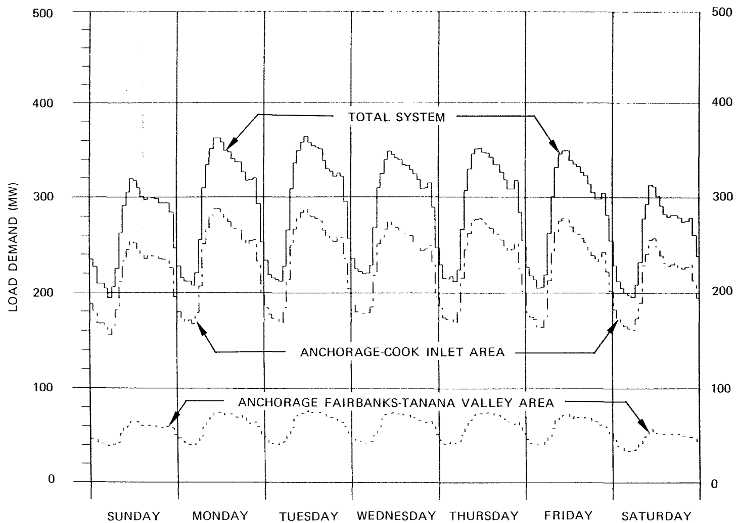
DAILY LOAD CURVES-AUGUST 1982
