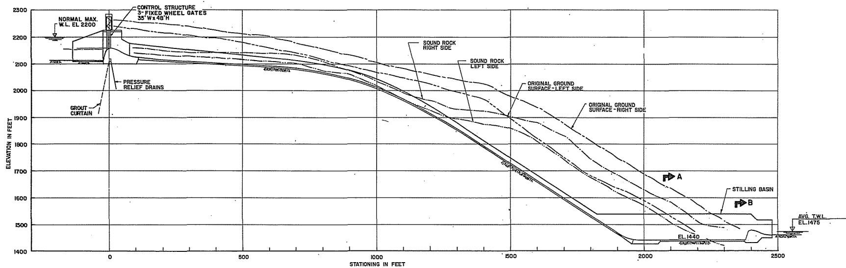
SPILLWAY PROFILE
