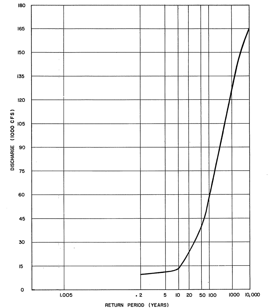
FLOOD FREQUENCY CURVE (INFLOW AFTER ROUTING THROUGH WATANA)
