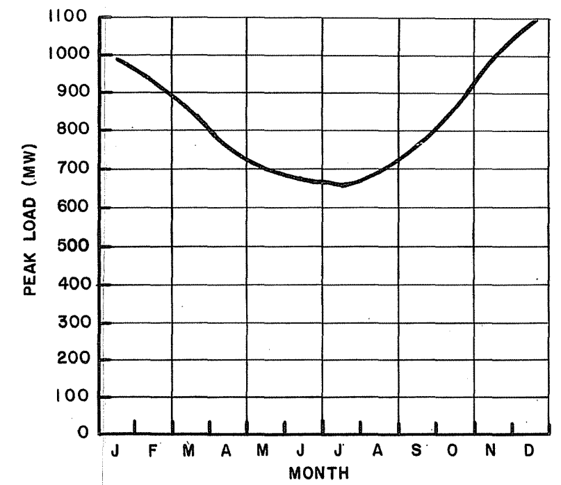
LOAD VARIATION IN YEAR 2000
