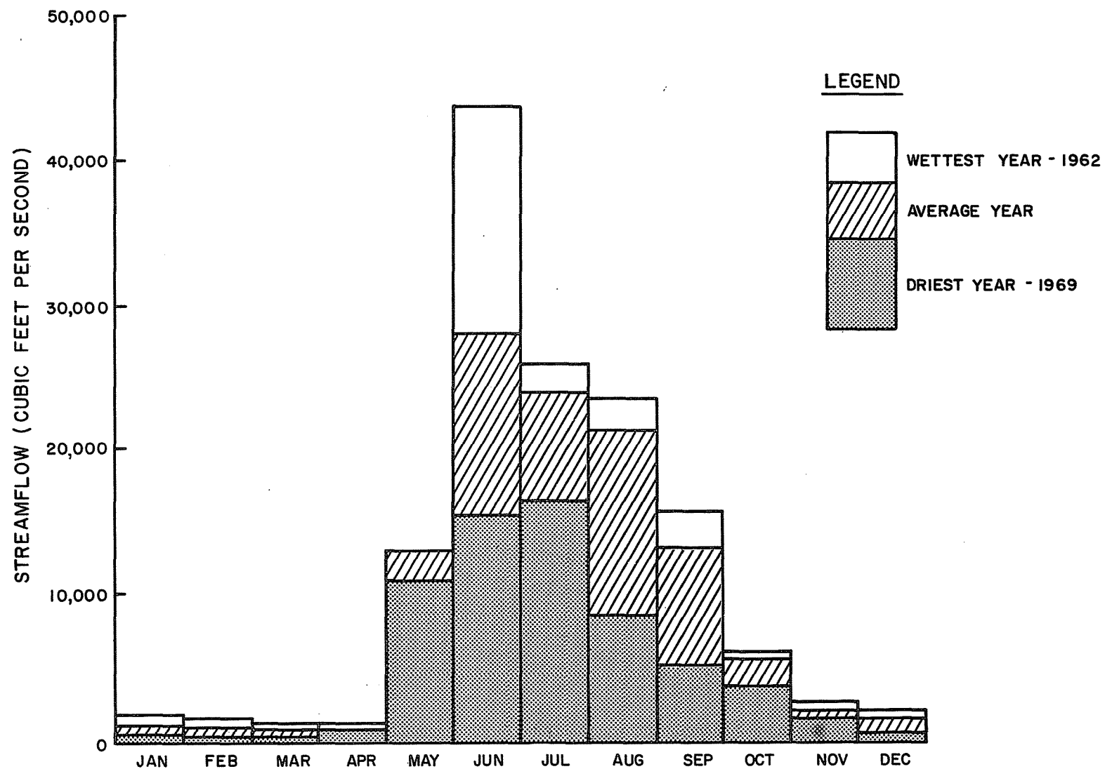
MONTHLY AVERAGE FLOWS SUSITNA RIVER AT GOLD CREEK
