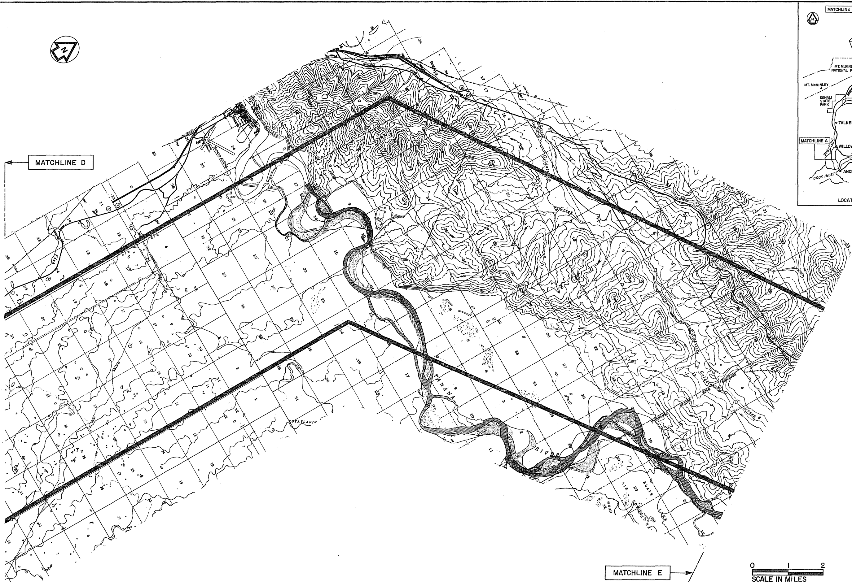
RECOMMENDED TRANSMISSION CORRIDOR NORTHERN STUDY AREA
