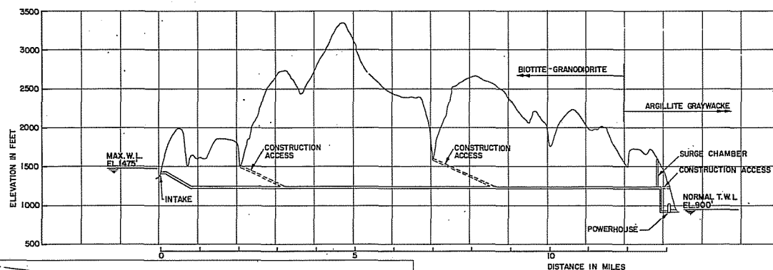
TUNNEL ALIGNMENT
