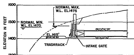
POWER TUNNEL INTAKE SECTION SCALE A
