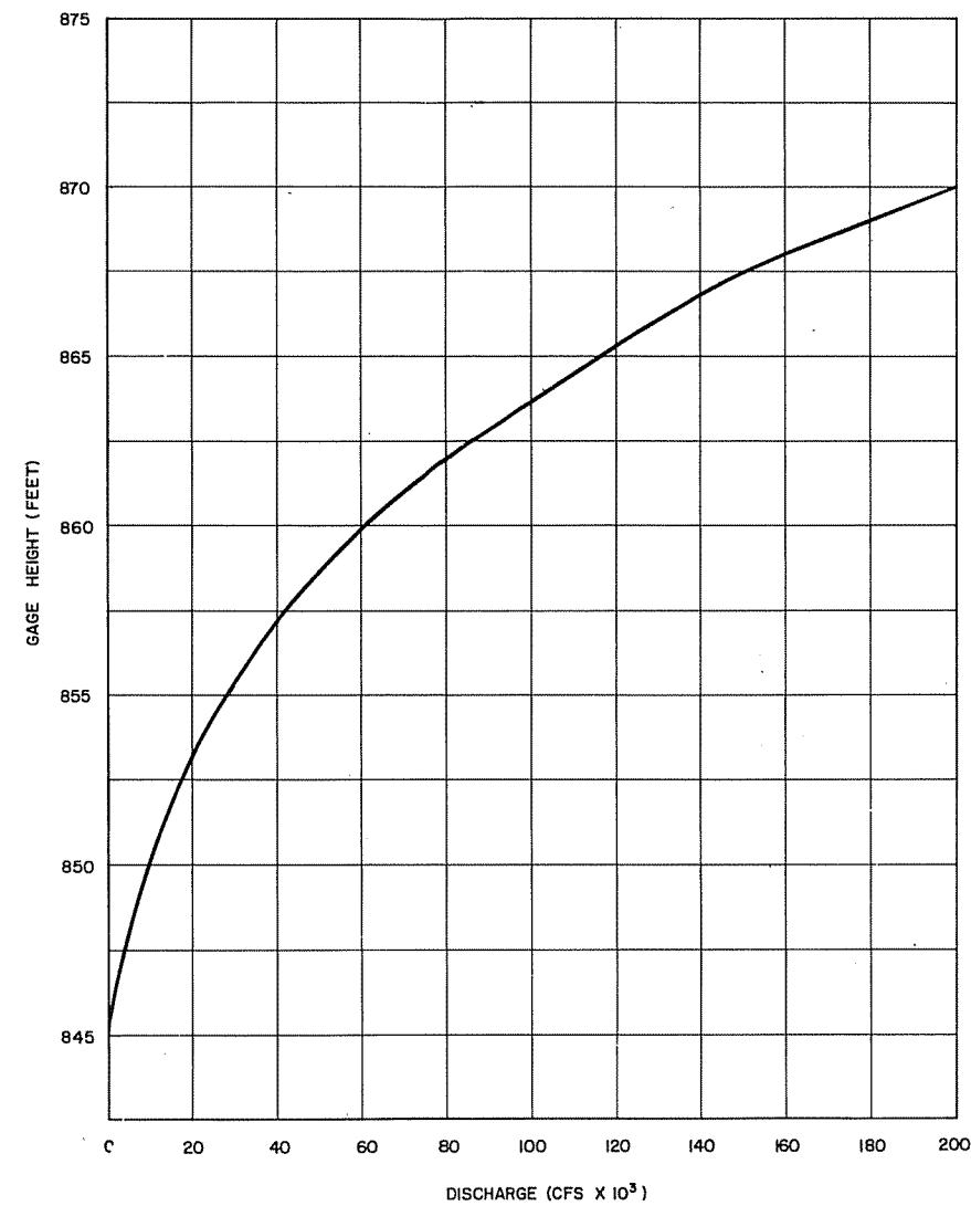
TAILWATER RATING CURVE
