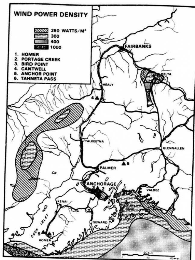
FIGURE 2.4. Wind Resources in the Railbelt Area and Sites Warranting Further Investigation in the Cook Inlet Area
