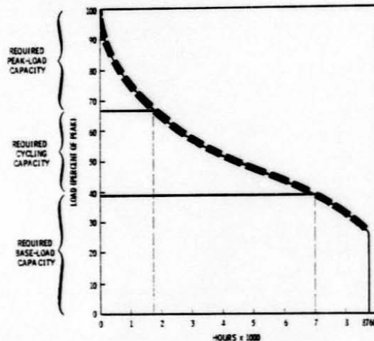
FIGURE 2.15. Typical Load Duration Curve for the Railbelt
