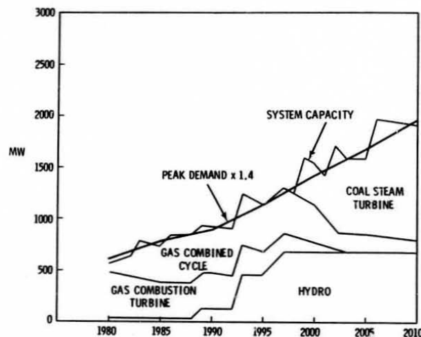
FIGURE 3.1. Plan 1A: Base Case Without Upper Susitna for Anchorage-Cook Inlet
