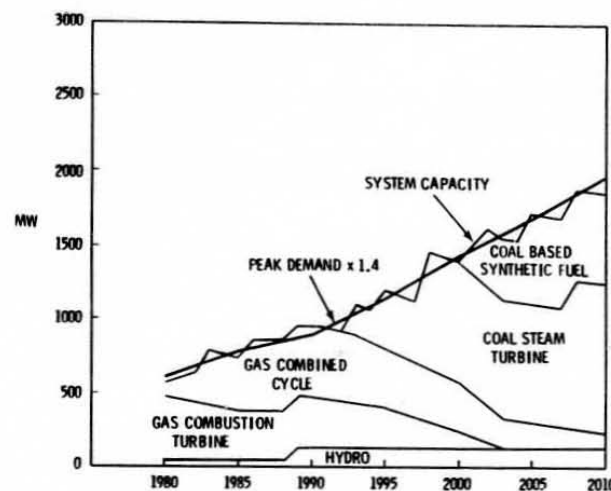
FIGURE 3.11. Plan 3: Increased Use of Coal for Anchorage-Cook Inlet
