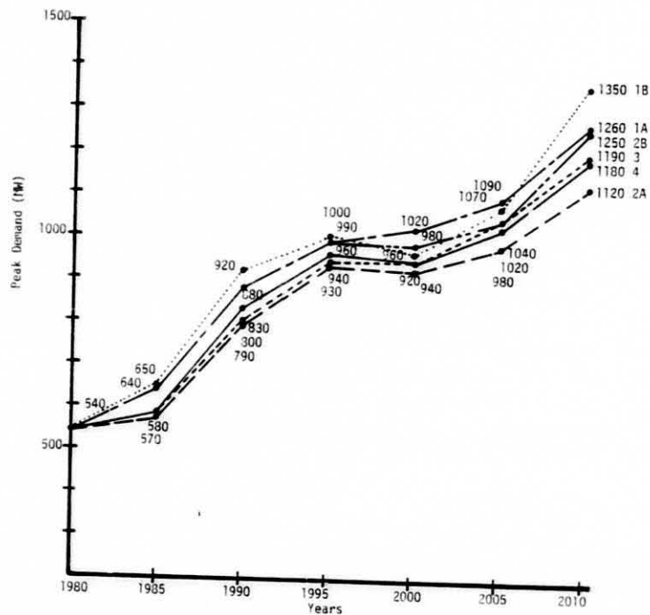
FIGURE 6.3. Peak Electrical Demands for Medium-Medium Economic Scenario
