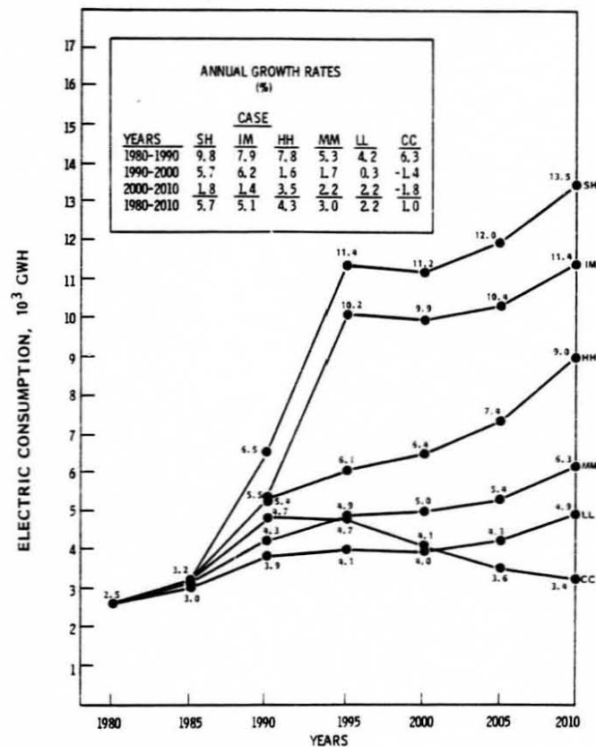
FIGURE 3.5. Railbelt Annual Electricity Consumption, 1980-2010 (a)
