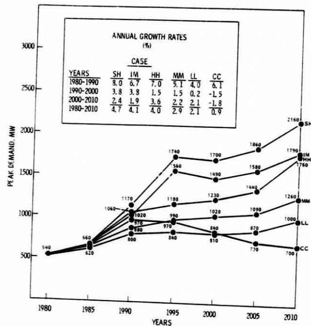
FIGURE 3.6. Railbelt Annual Peak Demand, 1980-2010 (a)
