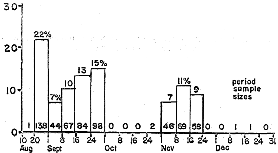
Figure 4. Chronology of 1967 Moose Harvest, Expressed in Percent by Period, Males, Unit 15.
